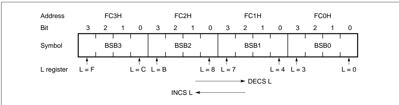
Figure 5-91. Format of the Bit Sequential Buffer
