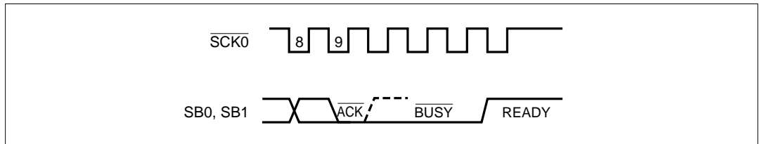
Figure 5-60. Busy and Ready Signals
