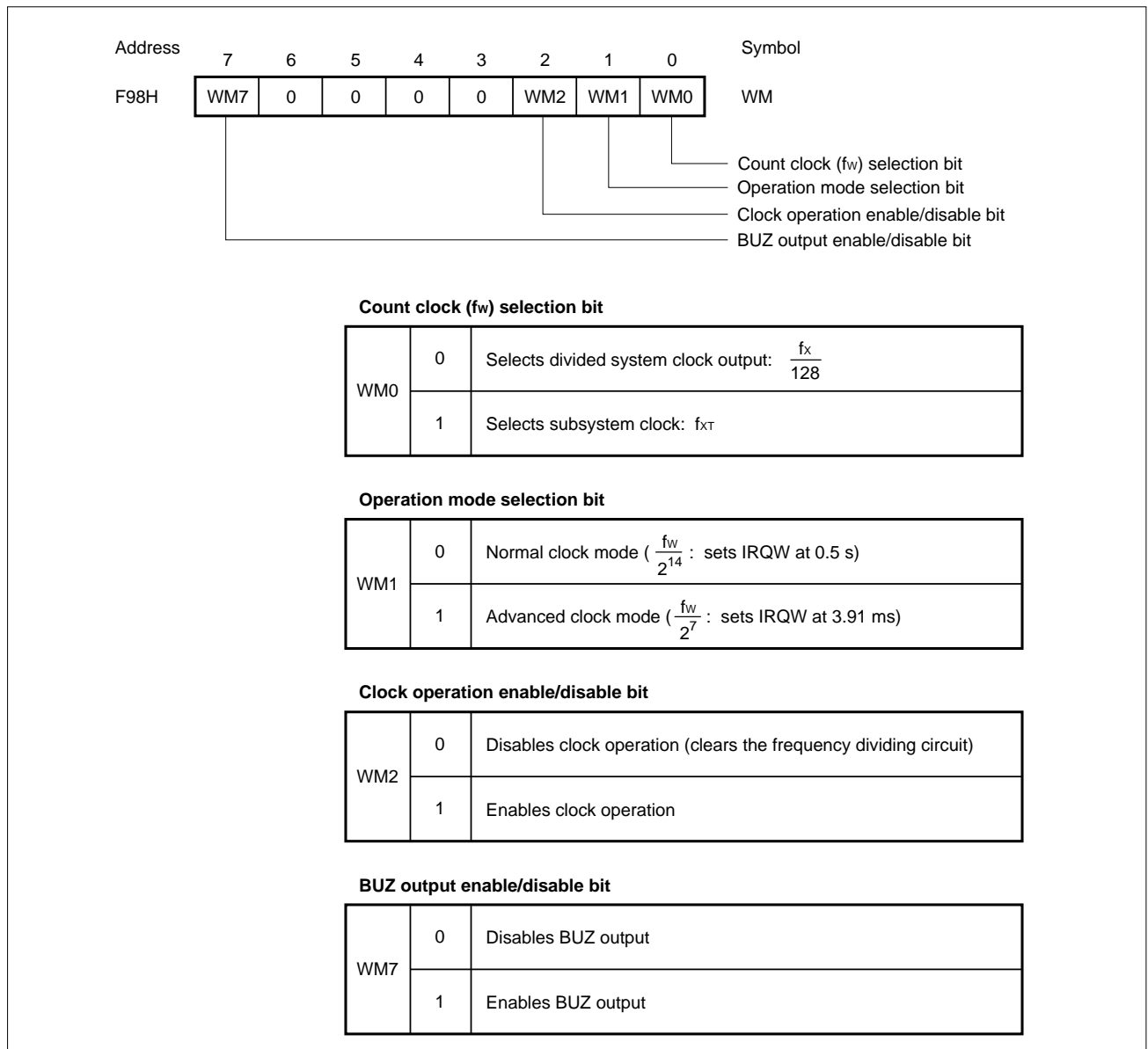
Figure 5-26. Format of the Watch Mode Register
