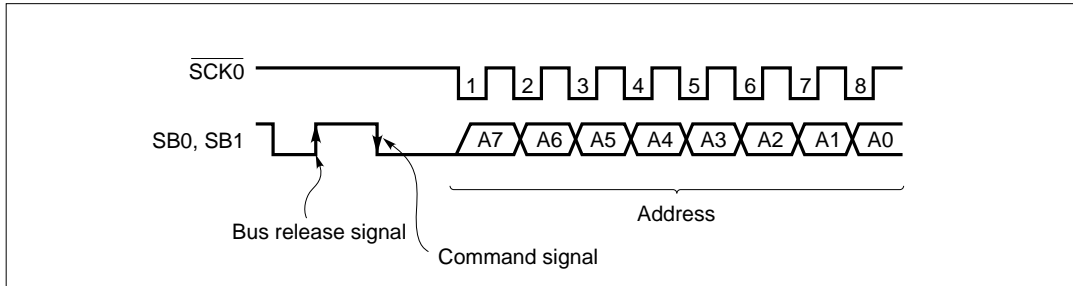
Figure 5-55. Address
