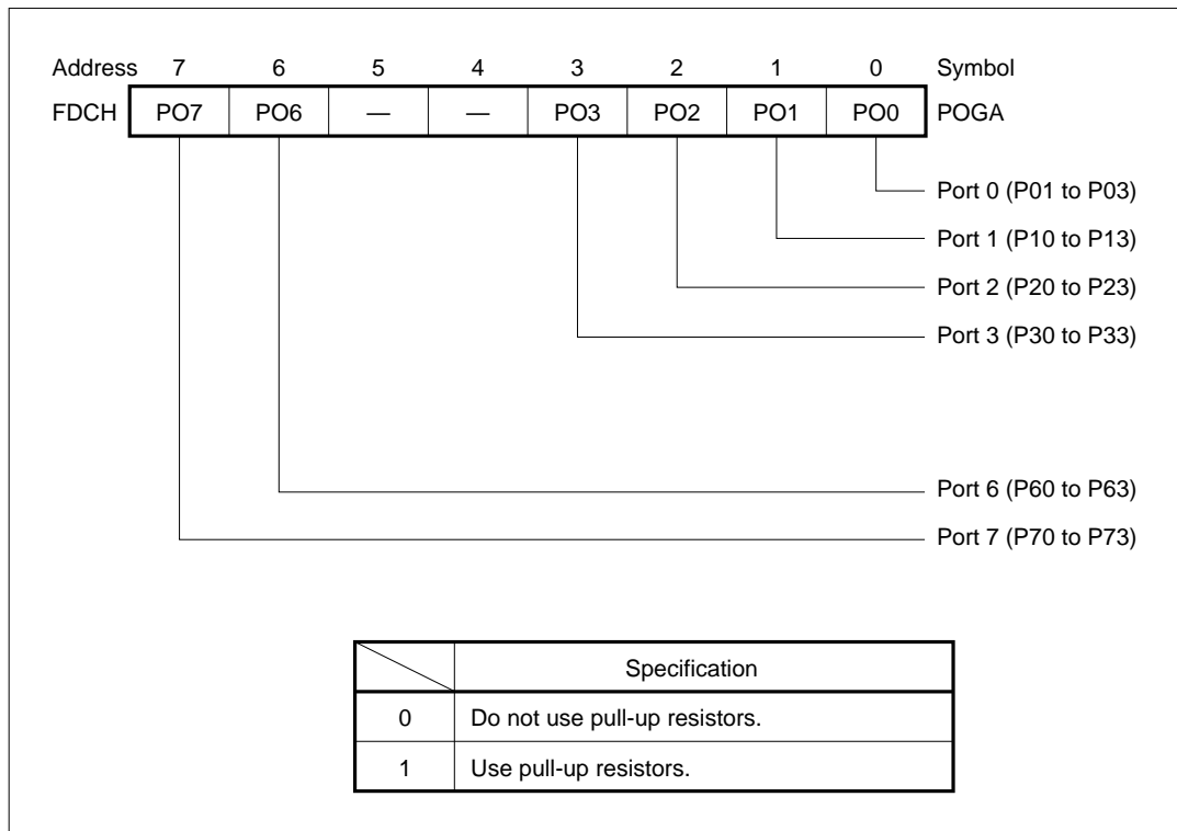
Figure 5-10. Format of the Pull-up Resistor Register
