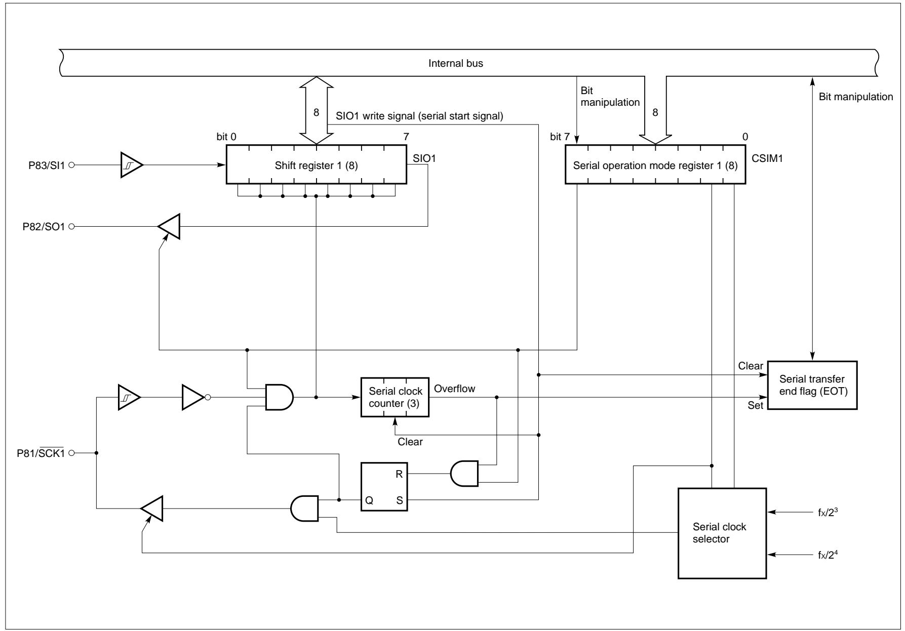
Figure 5-82. Block Diagram of the Serial Interface (Channel 1)
