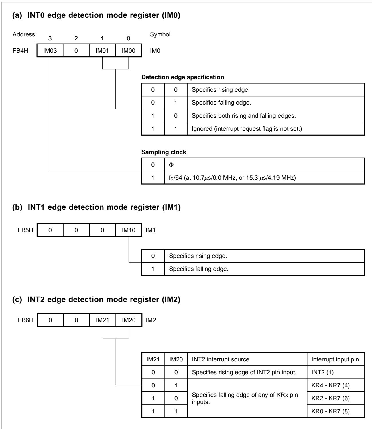
Figure 6-5. Format of Edge Detection Mode Registers
