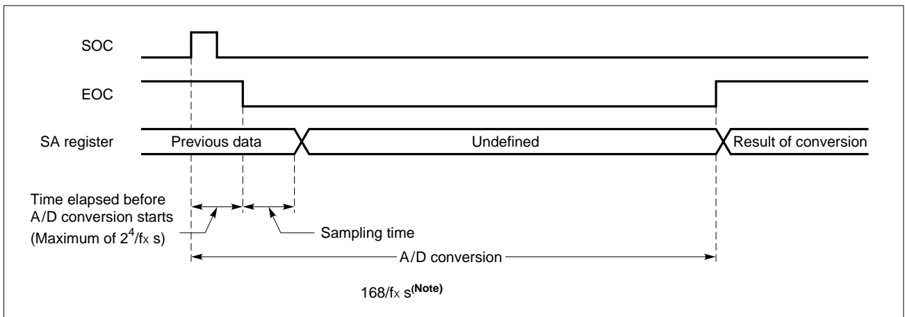
Figure 5-87. Timing Chart of A/D Conversion
