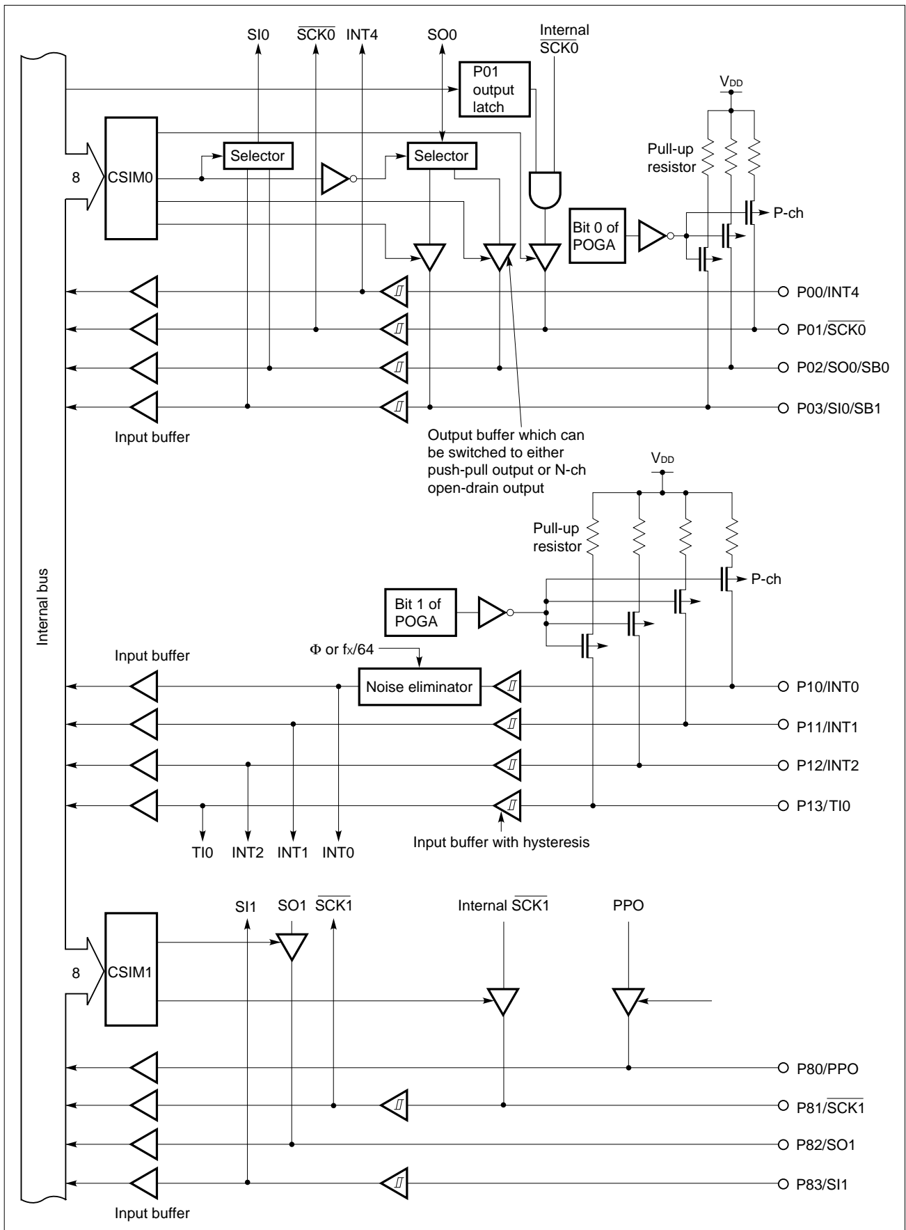
Figure 5-2. Configurations of Ports 0, 1, and 8
