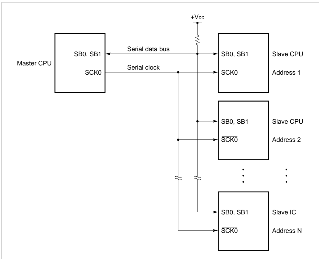
Figure 5-51. Example of SBI System Configuration
