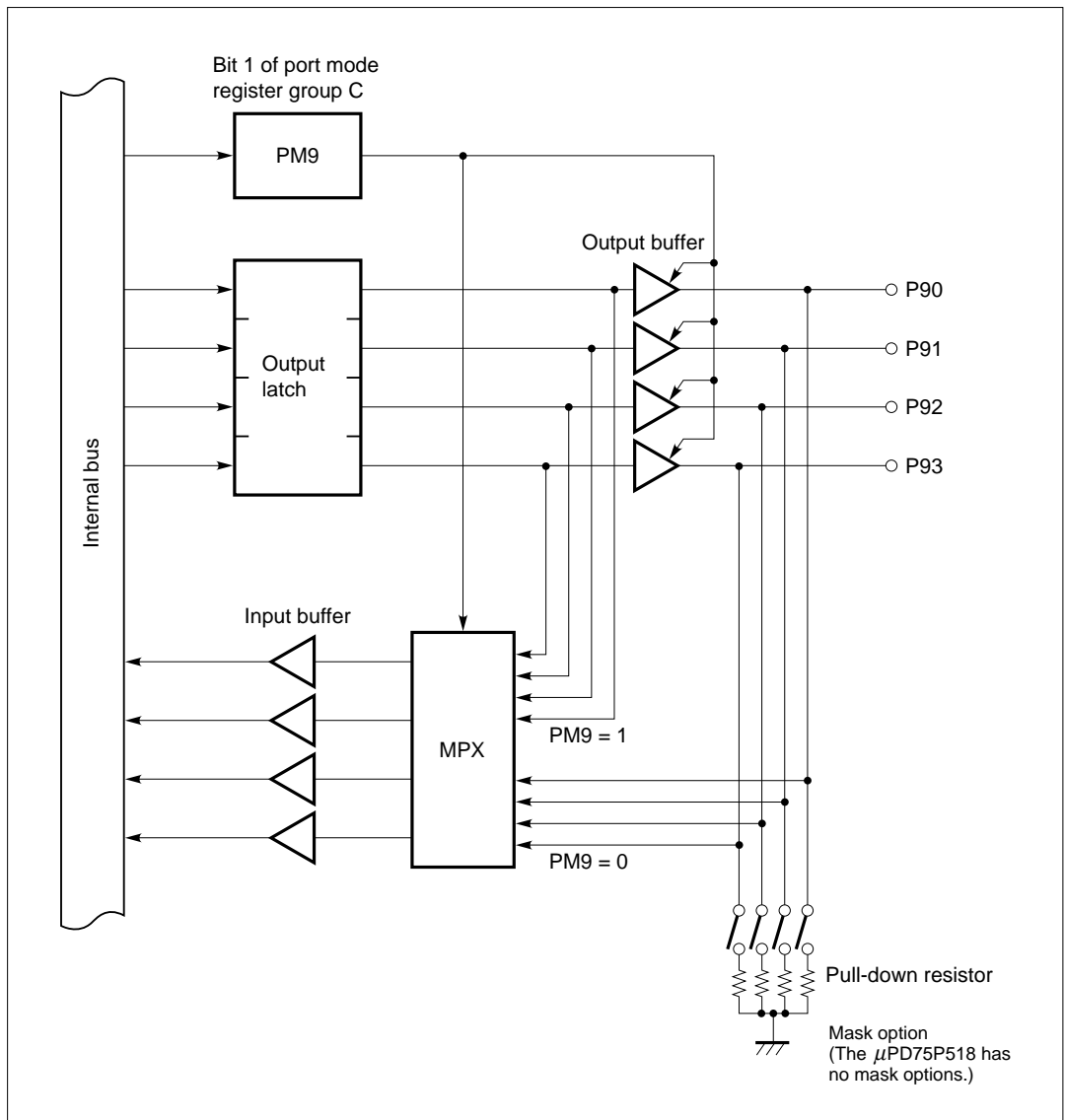
Figure 5-6. Configuration of Port 9
