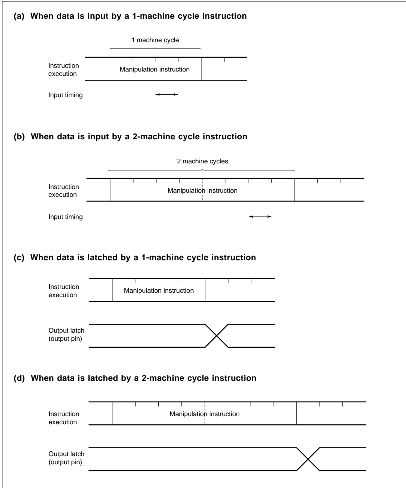
Figure 5-12. I/O Timing of Digital I/O Ports
