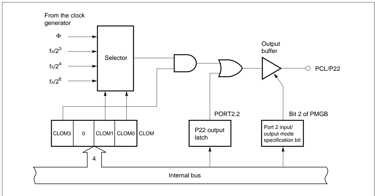
Figure 5-20. Configuration of the Clock Output Circuit
