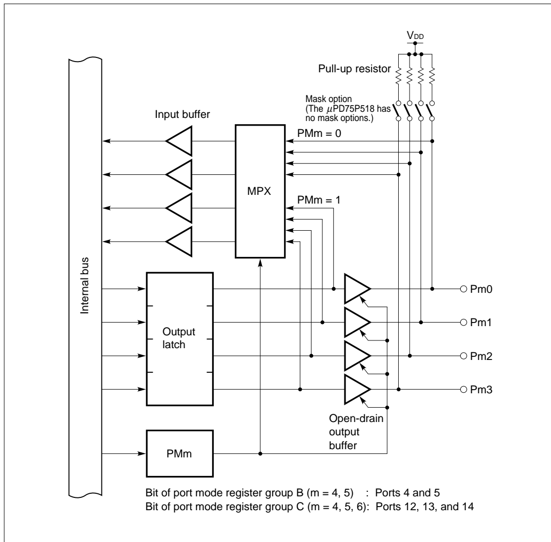
Figure 5-5. Configurations of Ports 4, 5, 12, 13, and 14
