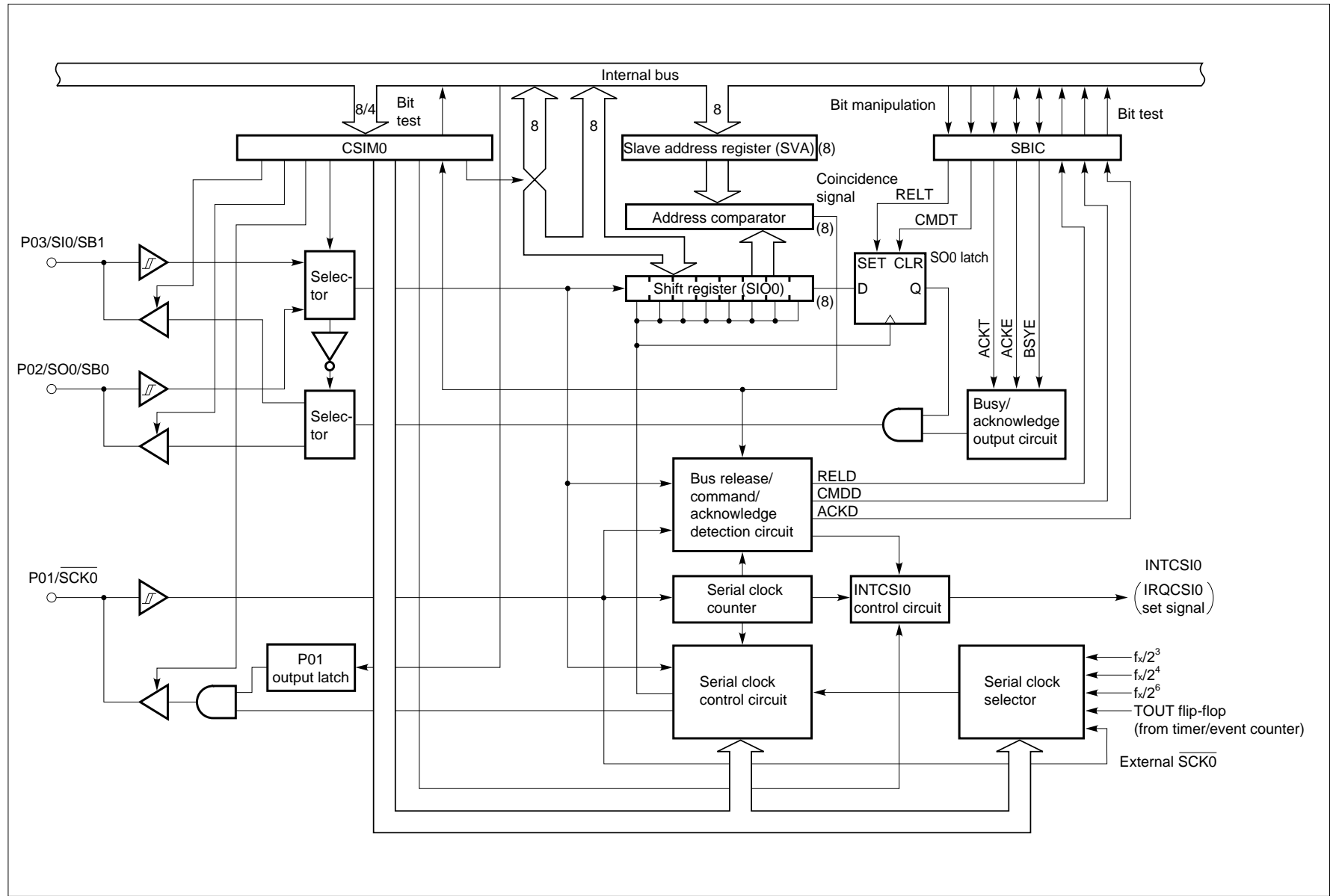
Figure 5-40. Block Diagram of the Serial Interface (Channel 0)
