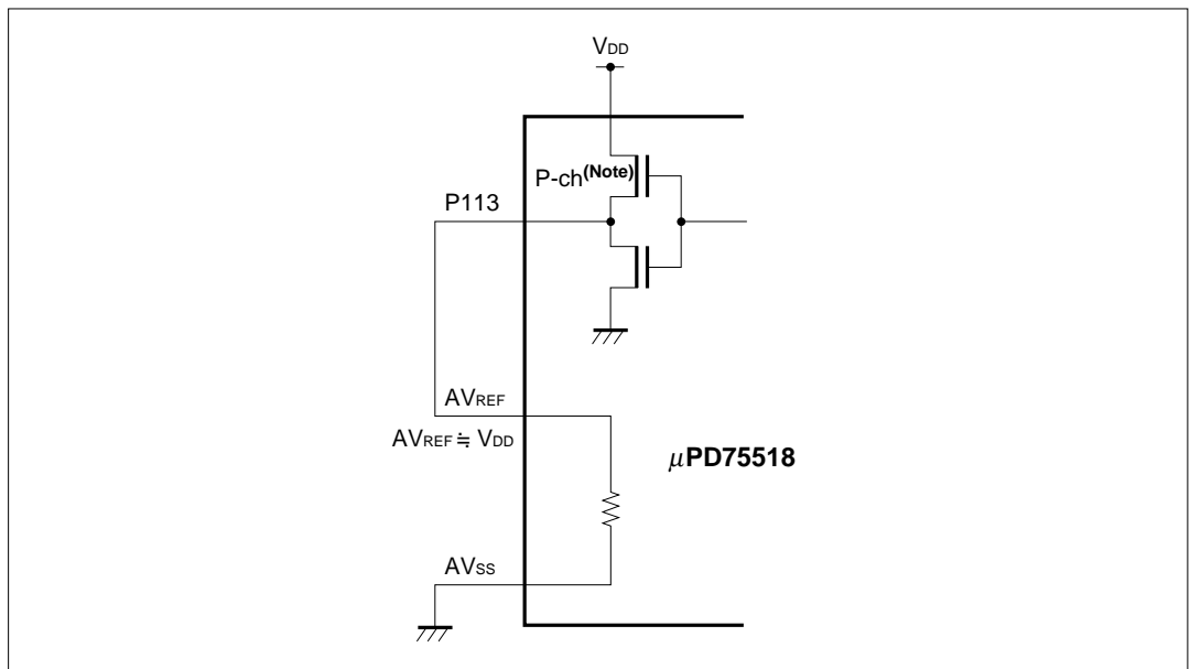
Figure 5-89. Reducing Power Consumption in the Standby Mode
