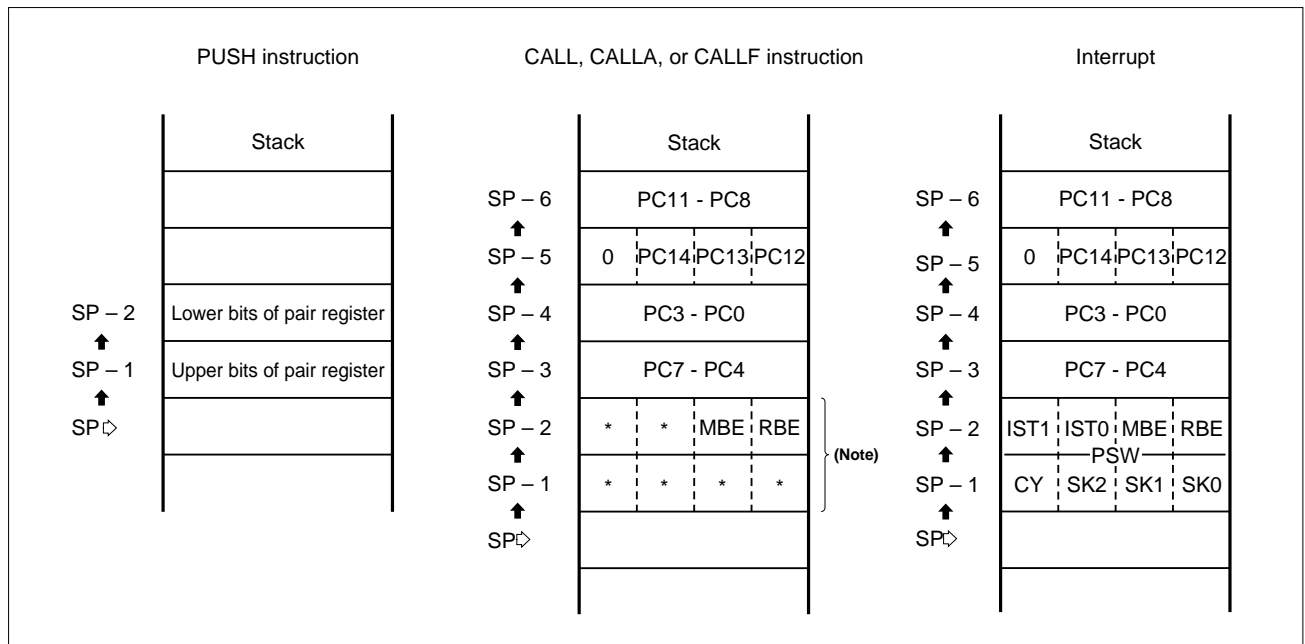
Figure 4-9. Data Saved to Stack Memory
