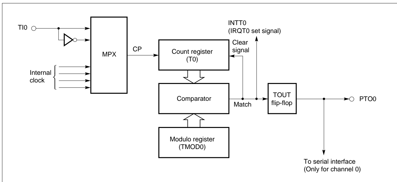
Figure 5-31. Operation in the Count Operation Mode
