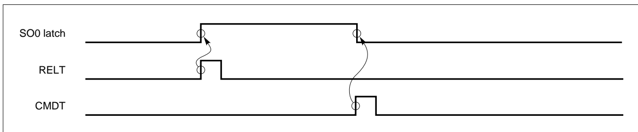
Figure 5-46. Operations of RELT and CMDT
