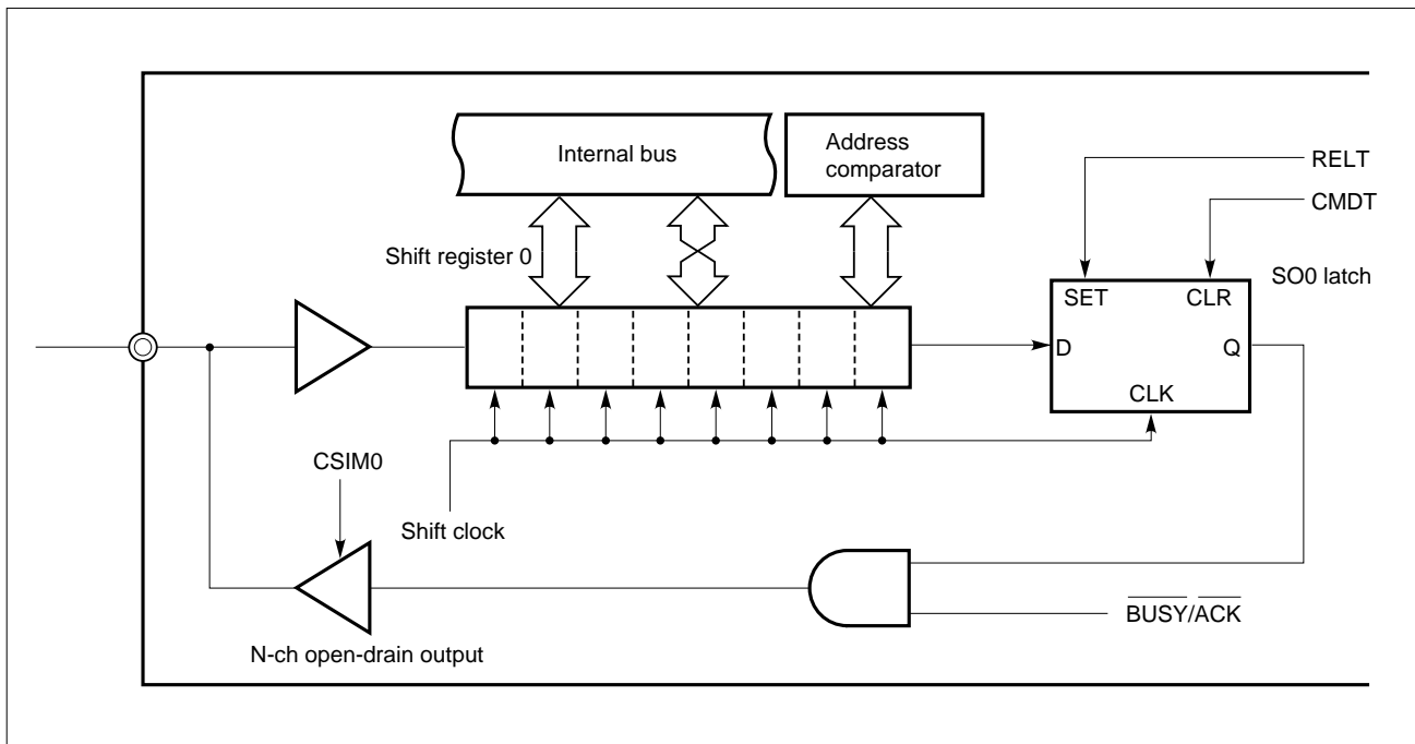
Figure 5-43. Peripheral Hardware of Shift Register 0
