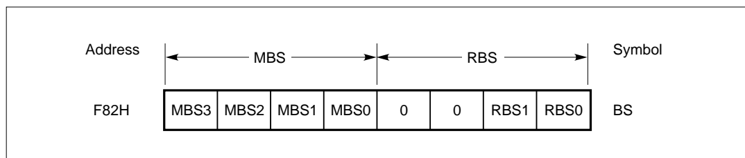
Figure 4-12. Bank Select Register Format
