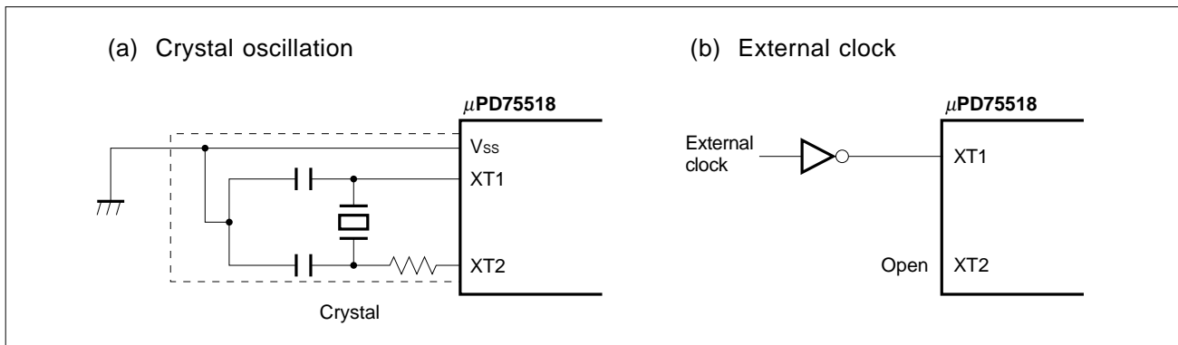
Figure 5-17. External Circuit for the Subsystem Clock Oscillator
