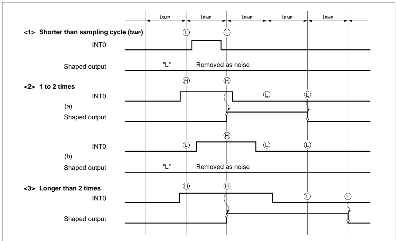
Figure 6-4. I/O Timing of a Noise Eliminator
