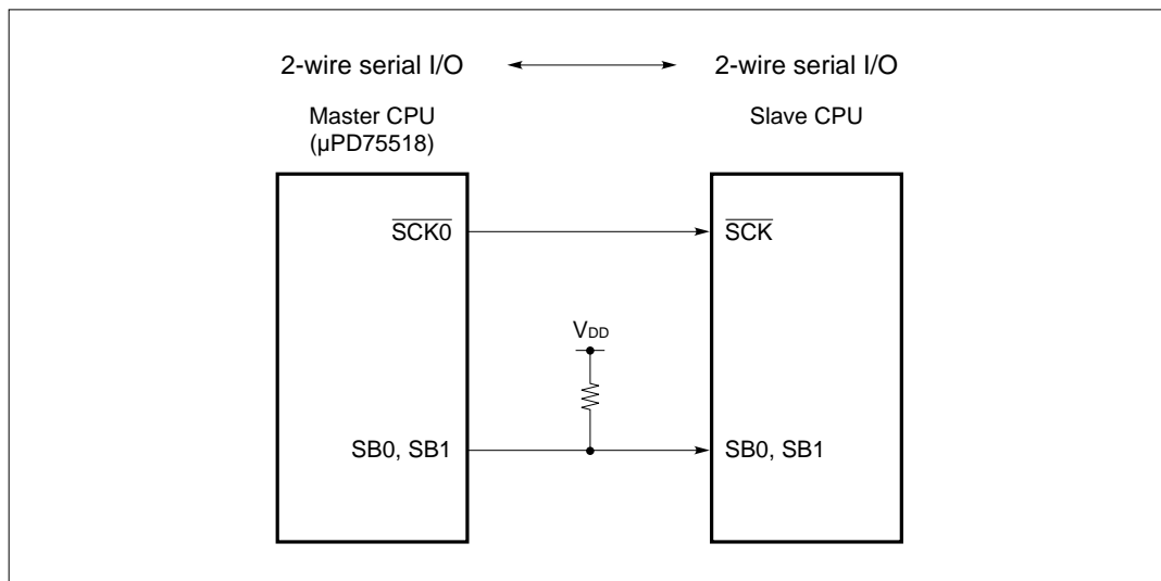
Figure 5-48. Example of Two-Wire Serial I/O System Configuration
