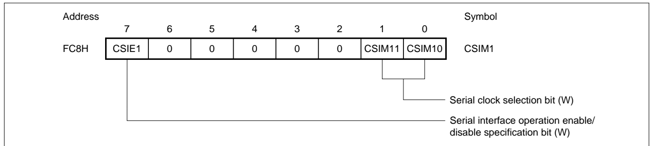
Figure 5-83. Format of Serial Operation Mode Register 1 (CSIM1)
