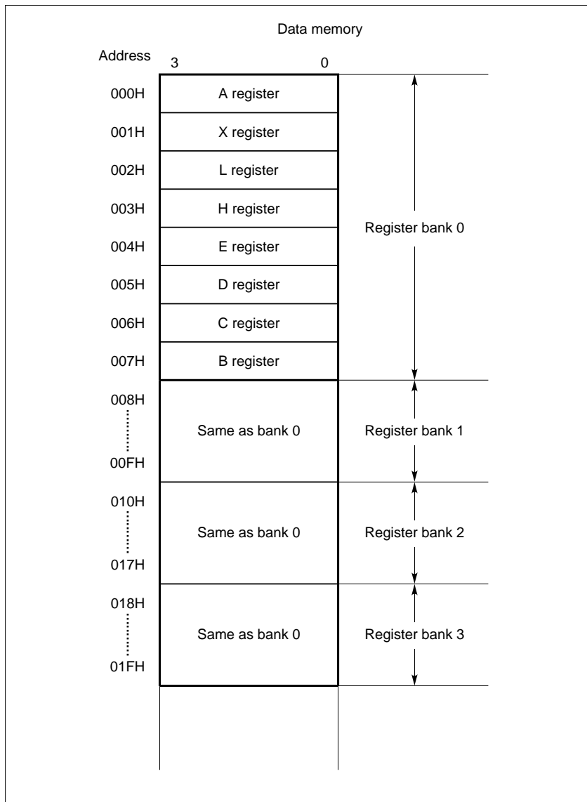
Figure 4-5. General Register Format
