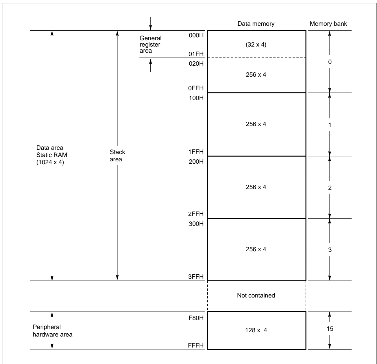
Figure 4-4. Data Memory Map
