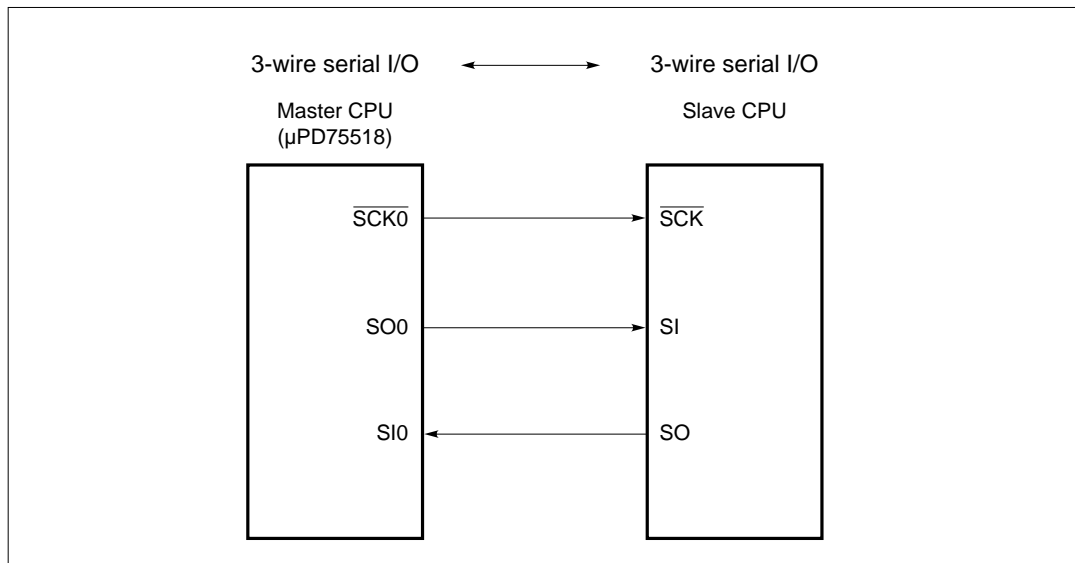
Figure 5-44. Example of Three-Wire Serial I/O System Configuration
