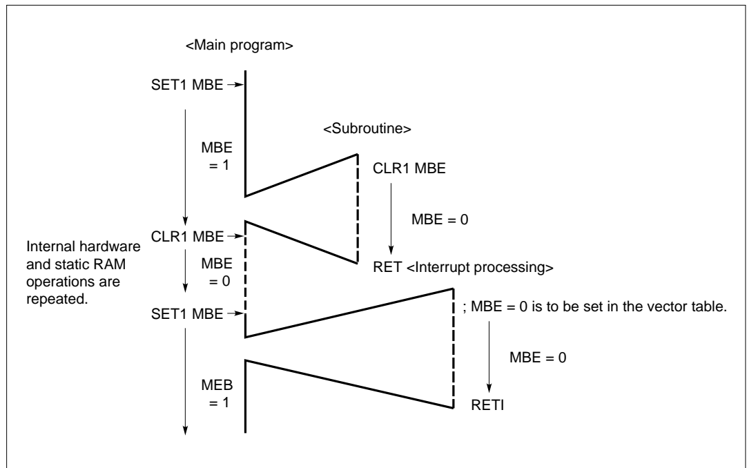
Figure 3-1. Use of MBE = 0 Mode and MBE = 1 Mode
