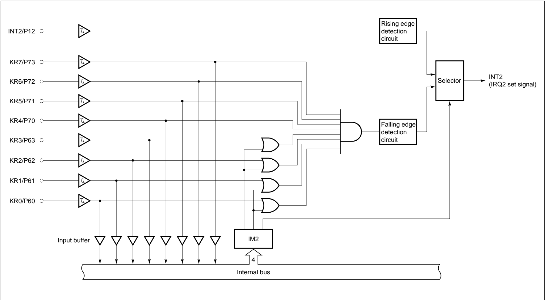
Figure 6-6. Configuration of the INT2 and KR0 to KR7 Circuits
