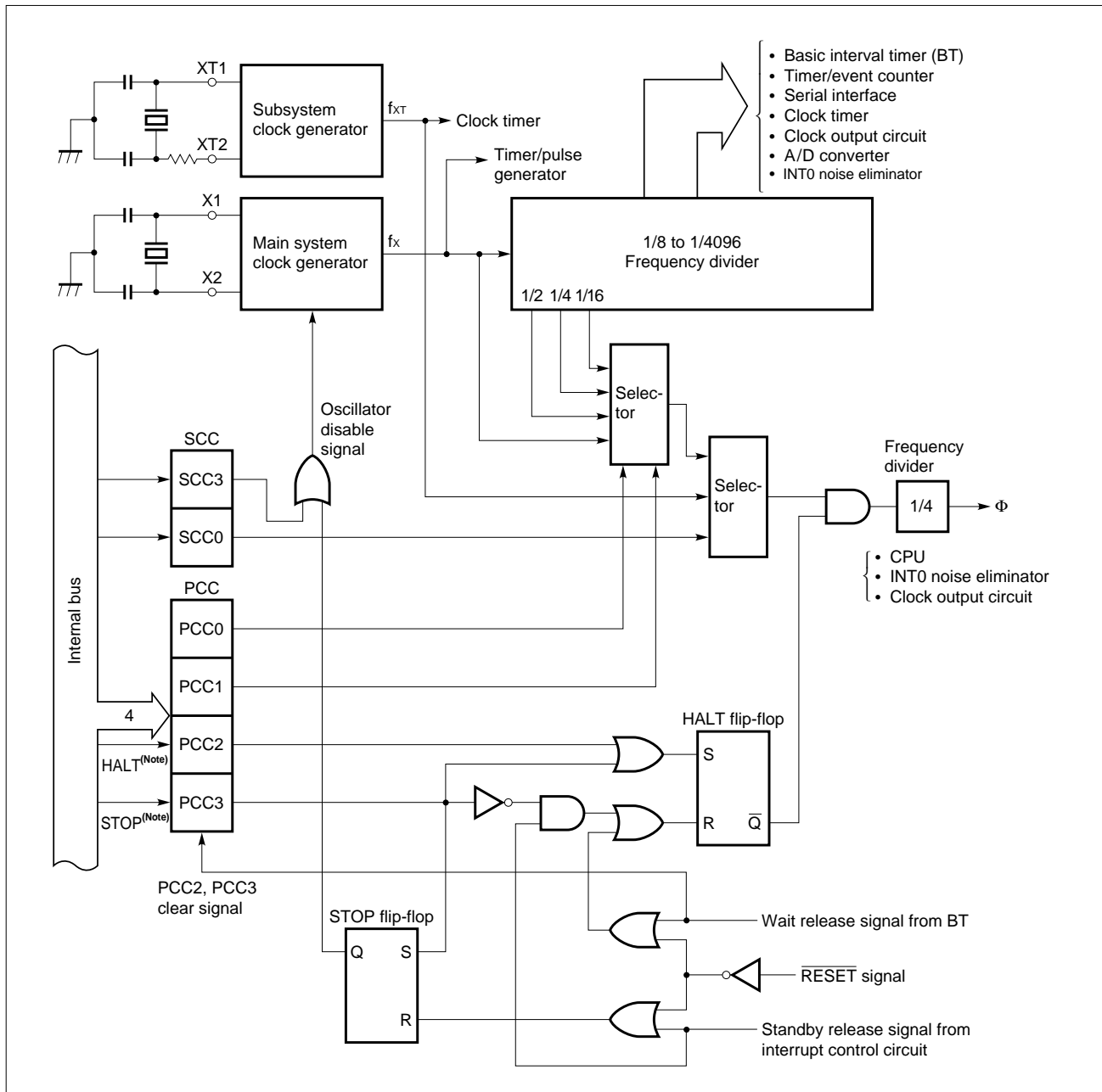
Figure 5-13. Block Diagram of the Clock Generator
