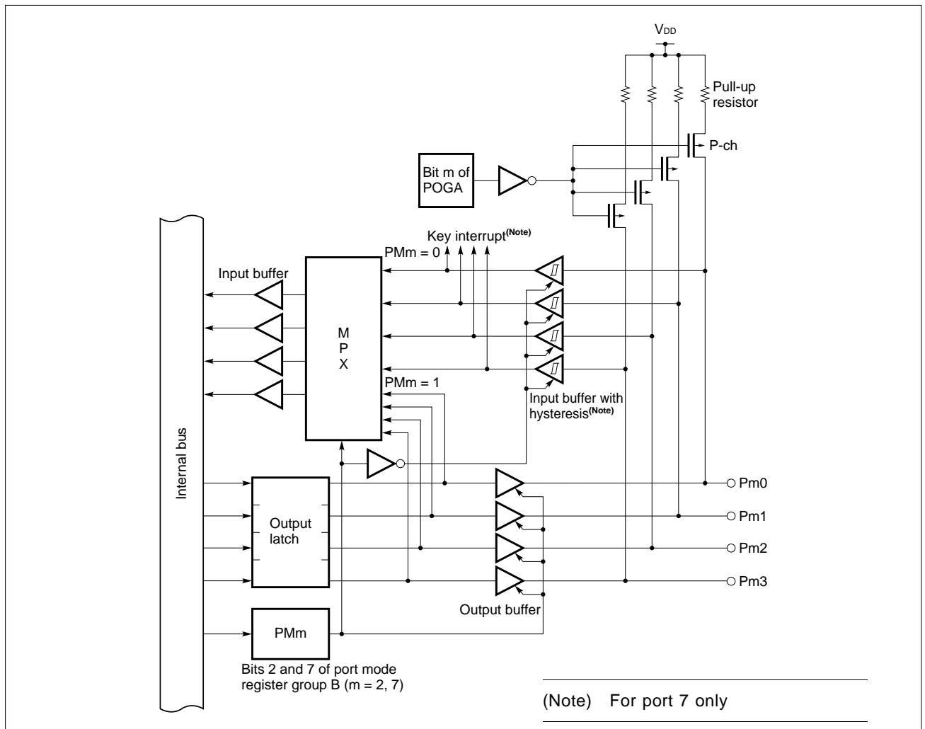
Figure 5-4. Configurations of Ports 2 and 7
