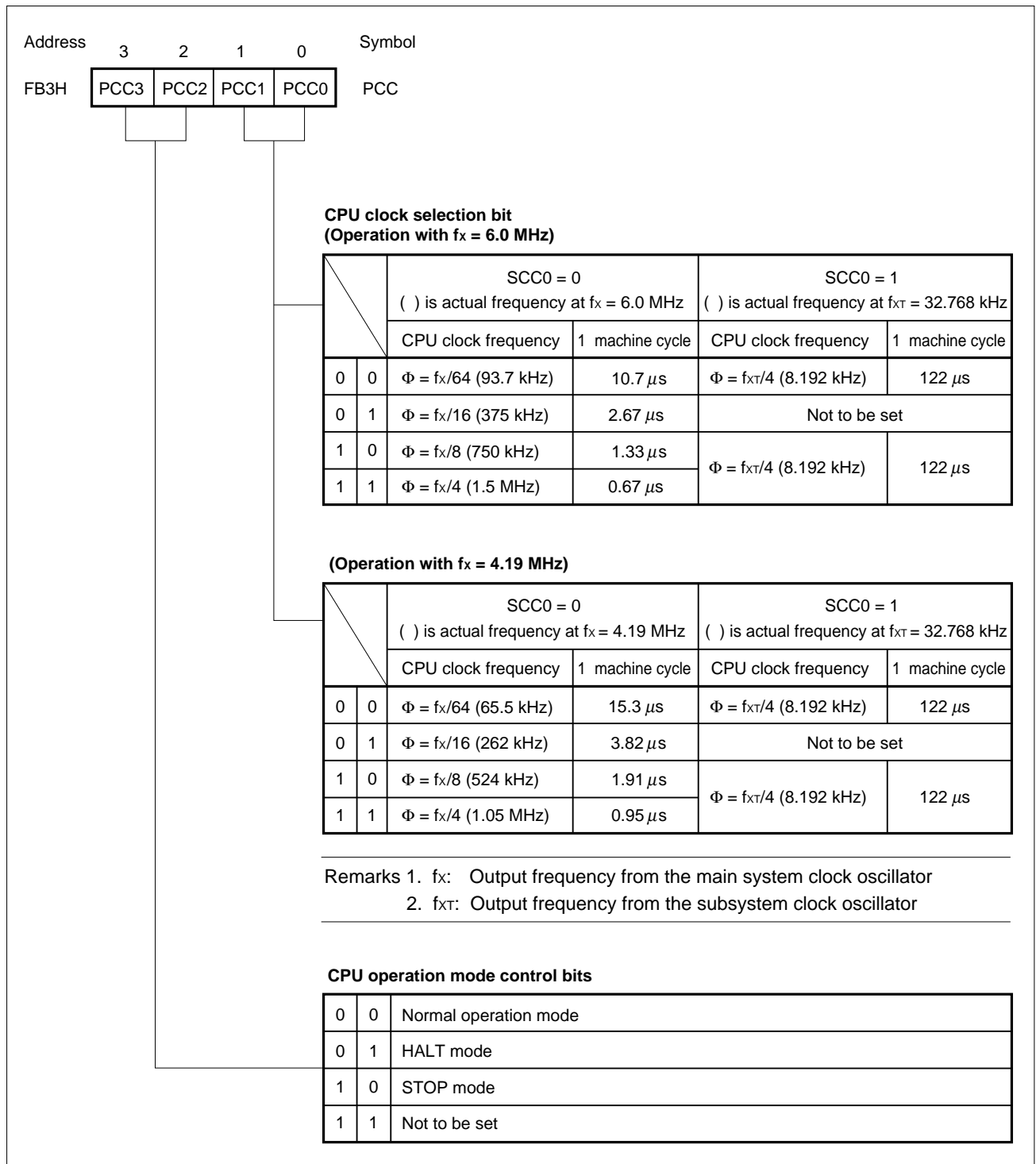
Figure 5-14. Format of the Processor Clock Control Register
