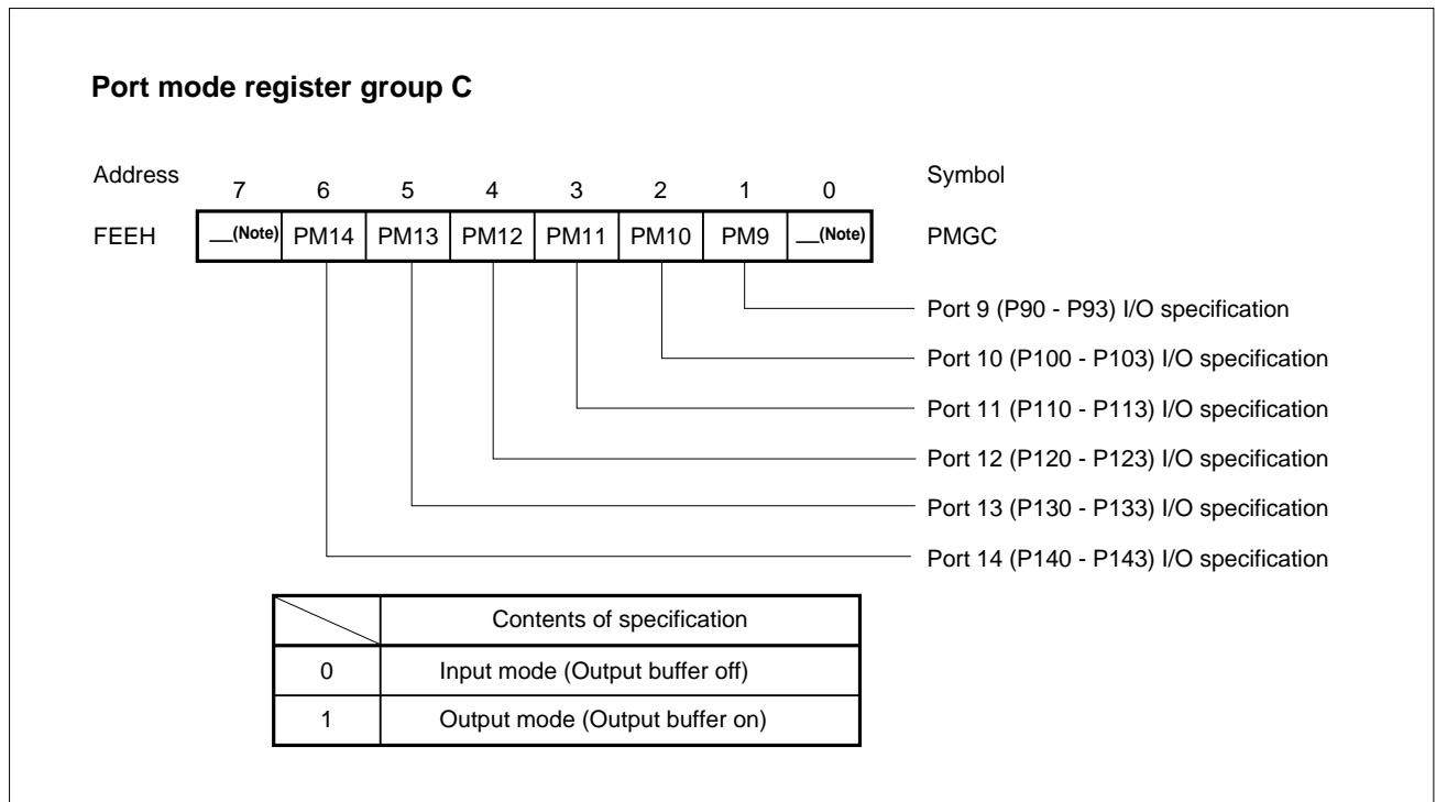
Figure 5-9. Formats of Port Mode Registers (2/2)
