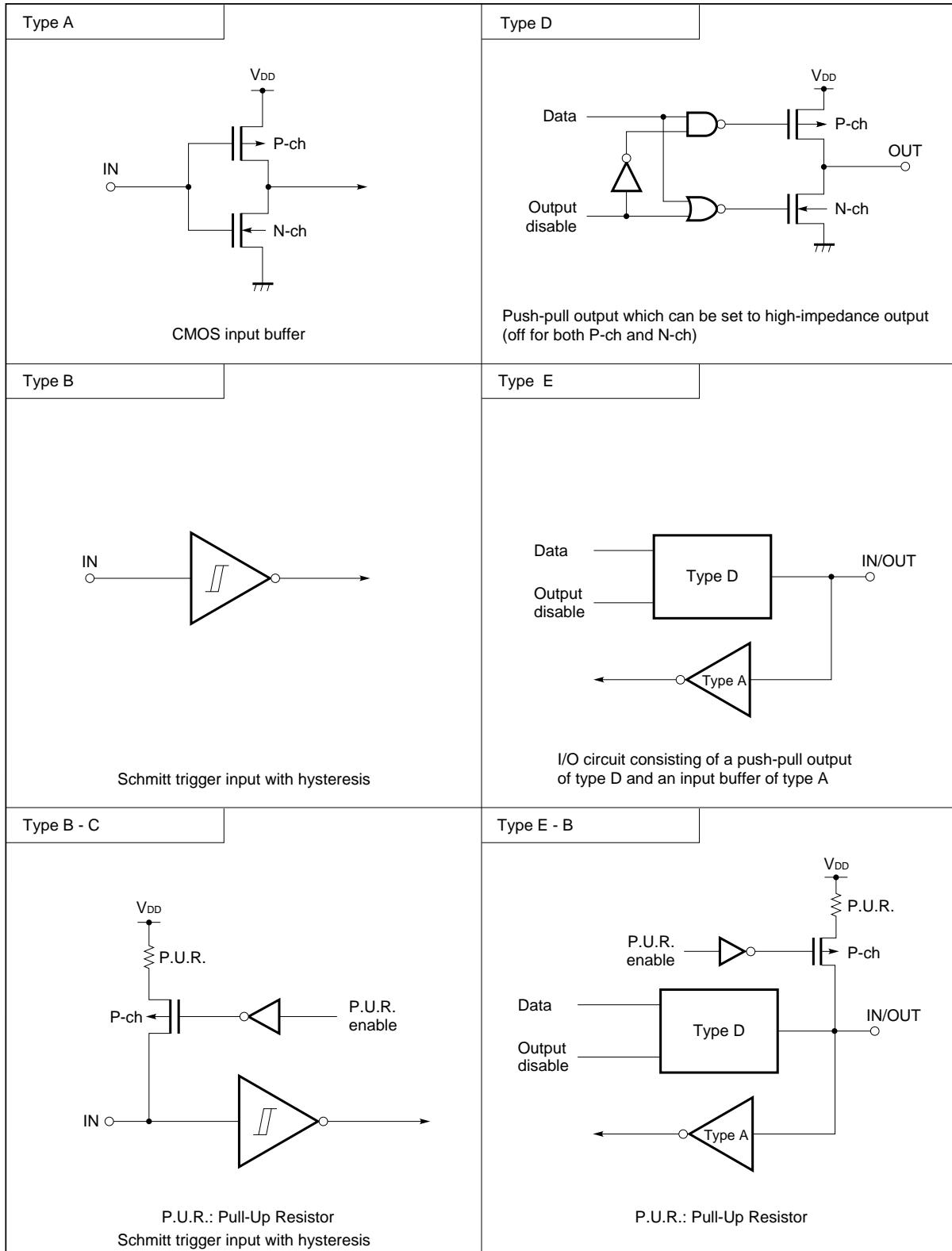
Figure 2-1. Pin Input/Output Circuits (1/3)
