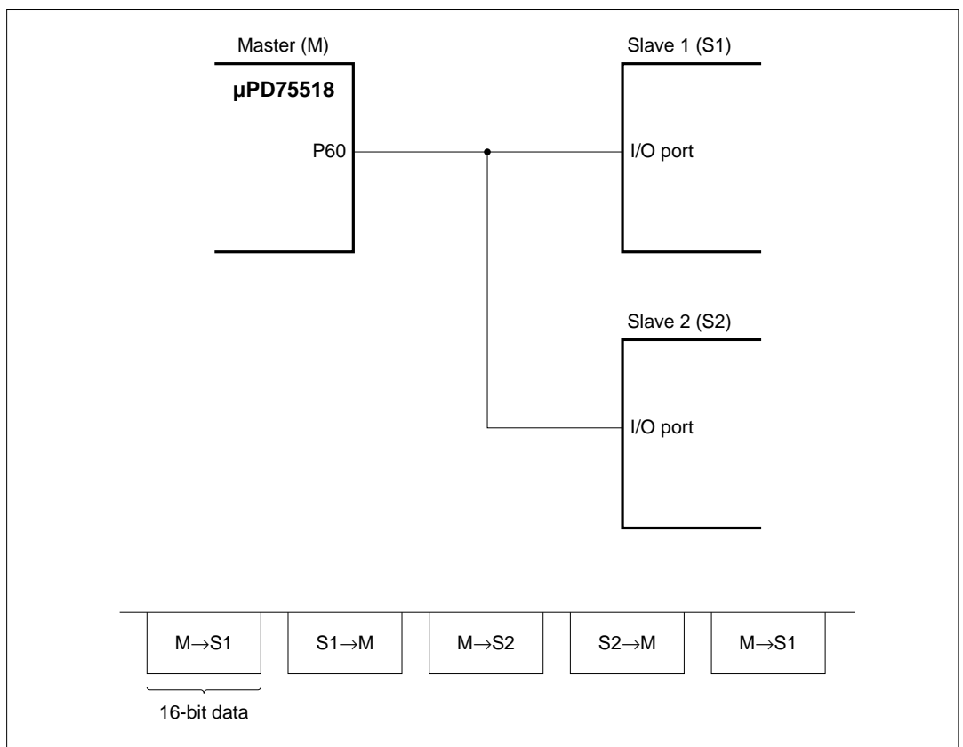
Figure 5-94. Bus Configuration Example
