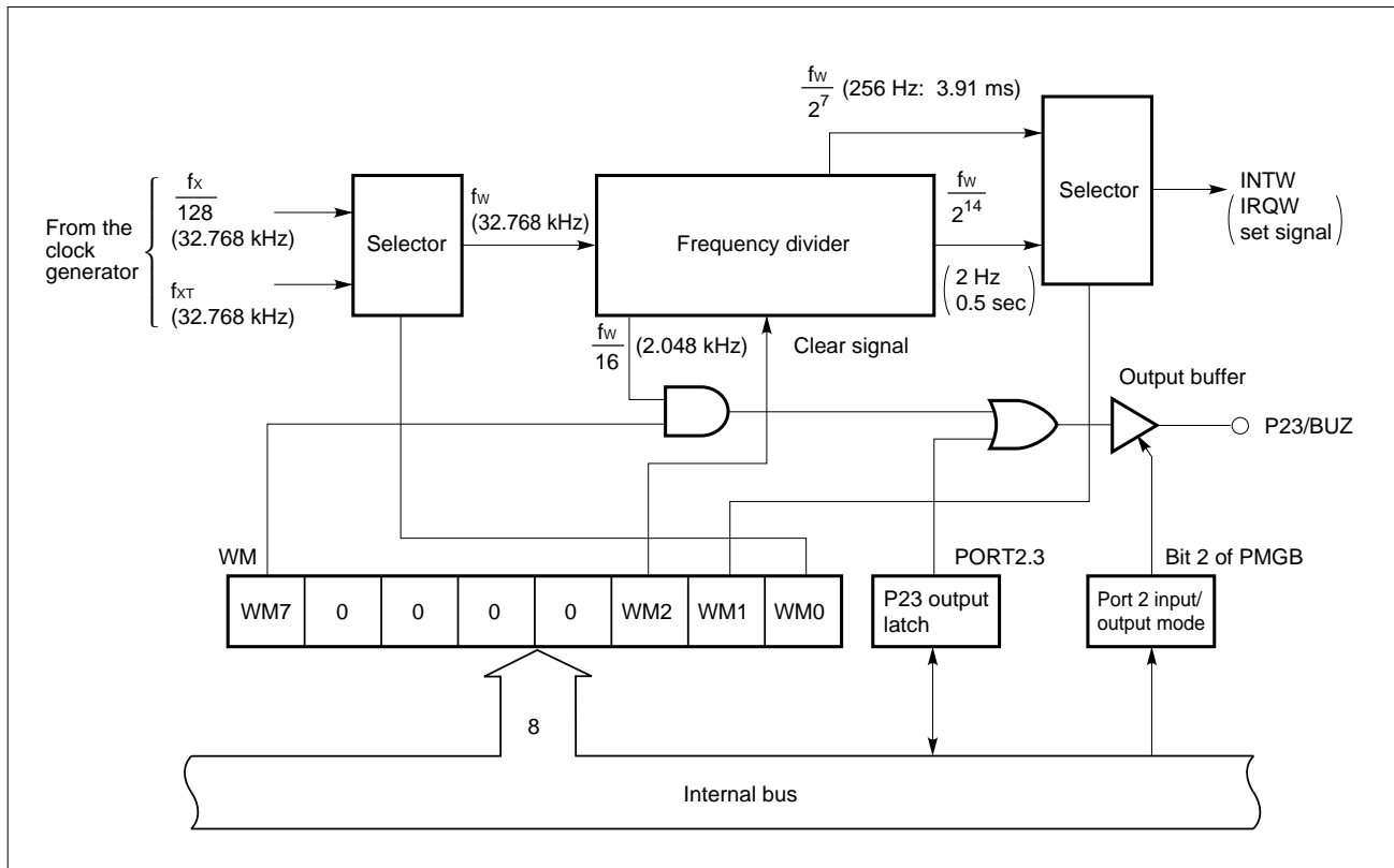
Figure 5-25. Block Diagram of the Clock Timer
