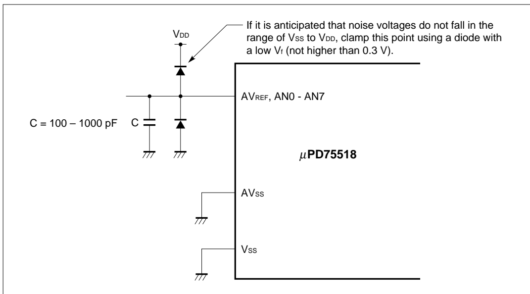
Figure 5-90. Analog Input Pin Connection
