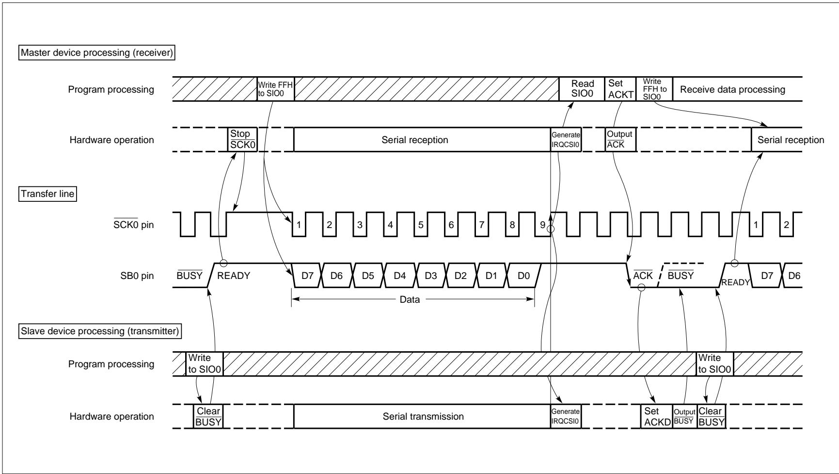
Figure 5-71. Data Transfer Operation from Slave Device to Master Device
