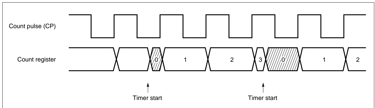
Figure 5-32. Error at the Start of the Timer
