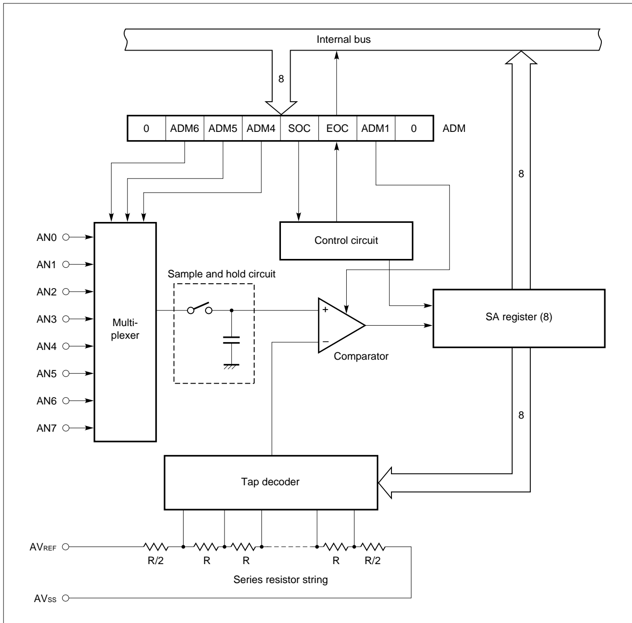
Figure 5-85. Block Diagram of the A/D Converter
