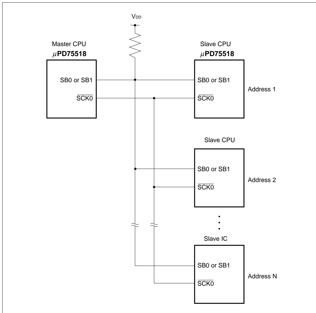
Figure 5-72. Example of Serial Bus Configuration
