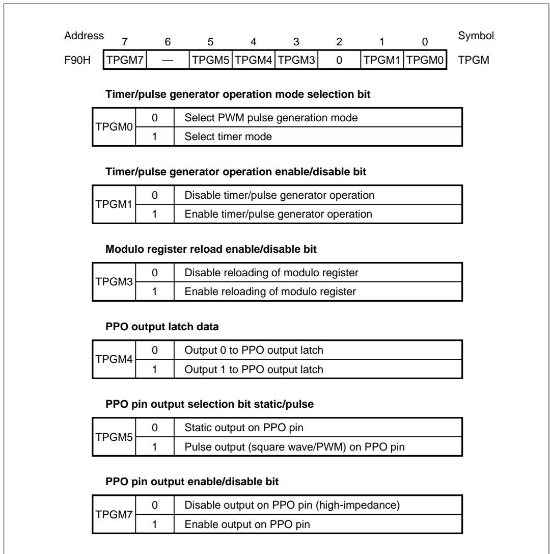
Figure 5-33. Format of Timer/Pulse Generator Mode Register
