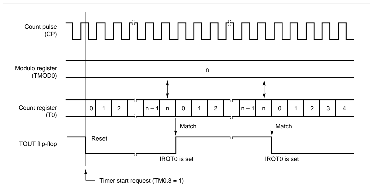
Figure 5-28. Timing of Count Operation
