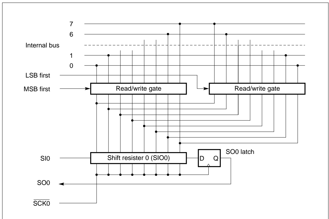
Figure 5-47. Transfer Bit Switching Circuit
