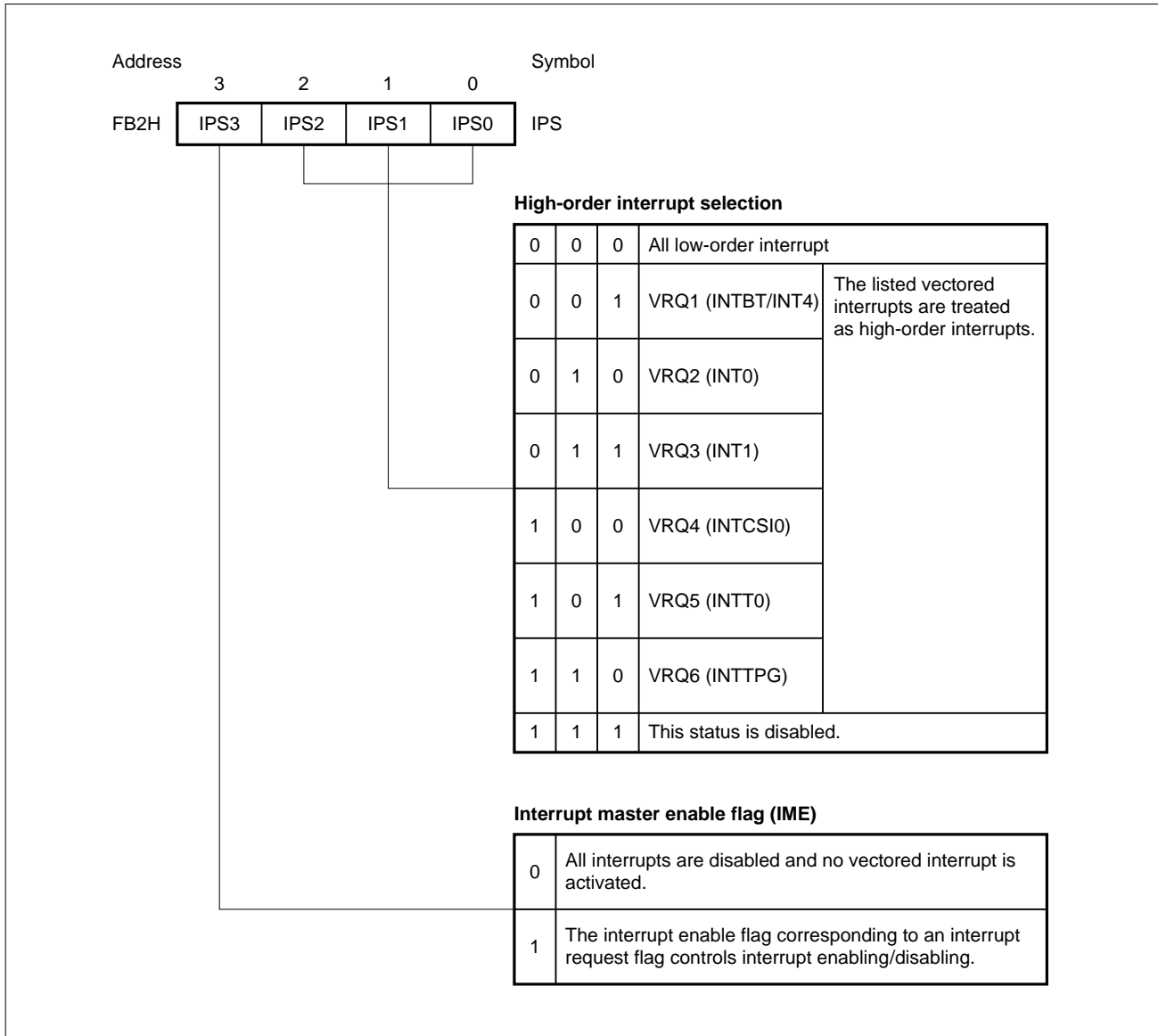
Figure 6-7. Interrupt Priority Specification Register
