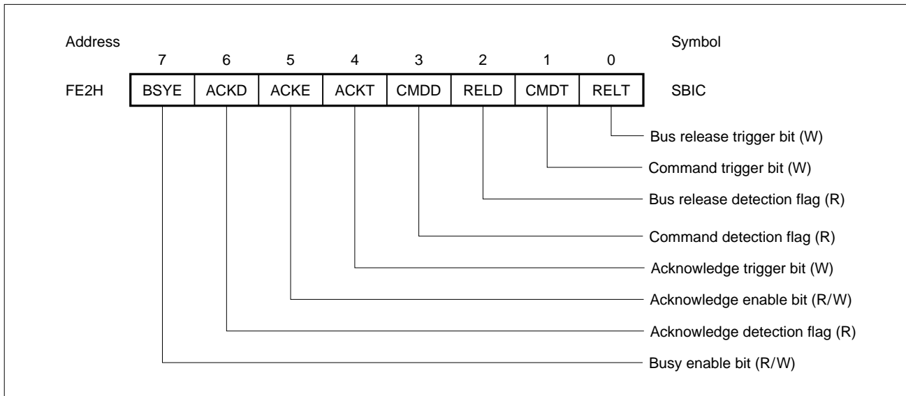
Figure 5-42. Format of Serial Bus Interface Control Register (SBIC) (1/3)
