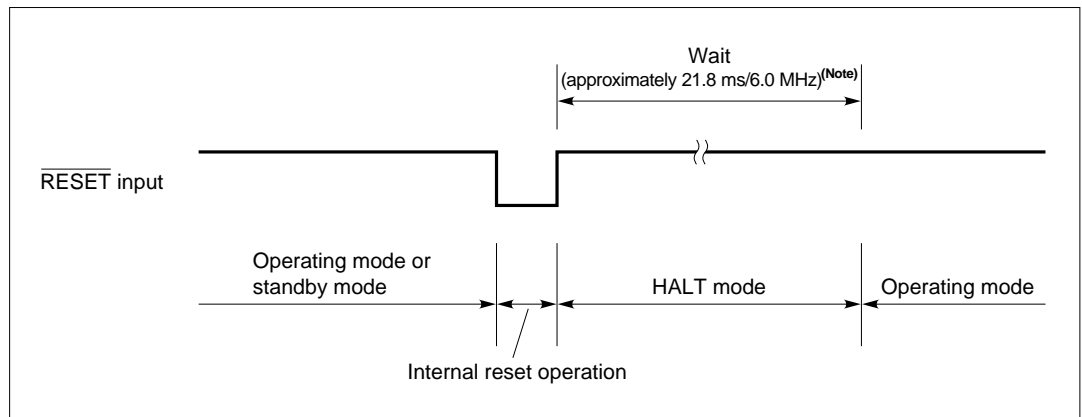
Figure 8-1. Reset Operation by a \overline{\text{RESET}} signal
