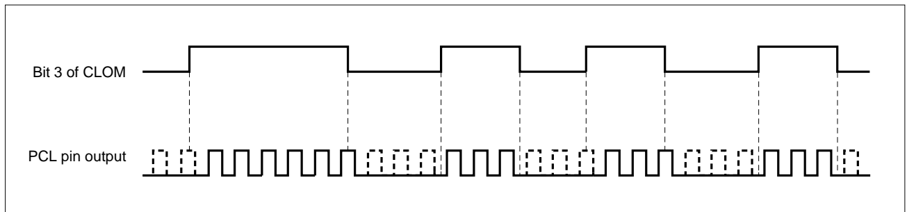
Figure 5-22. Application to Remote Control Output
