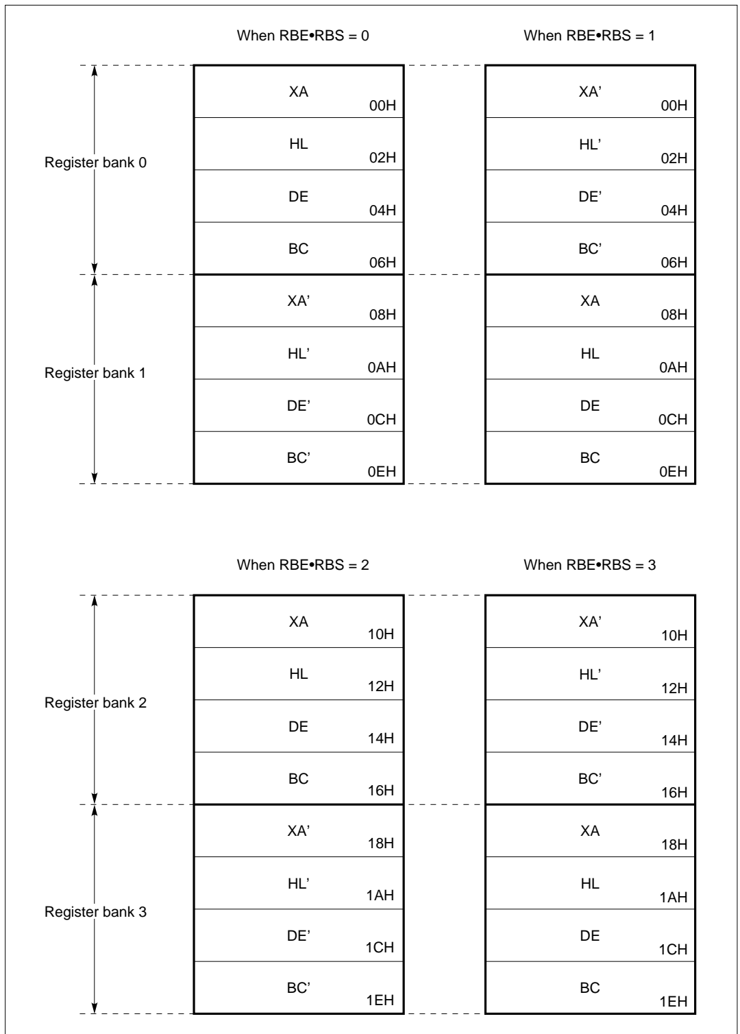
Figure 3-6. General Register Configuration (8-bit Processing)
