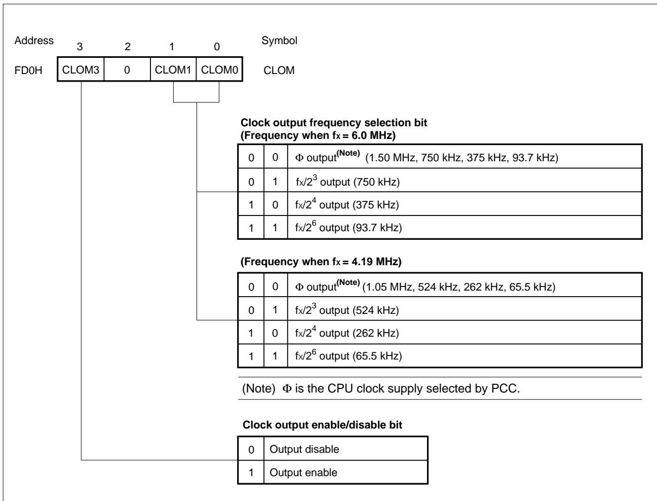
Figure 5-21. Format of the Clock Output Mode Register
