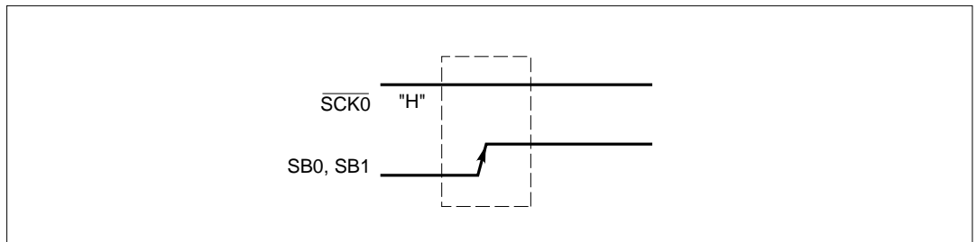
Figure 5-53. Bus Release Signal
