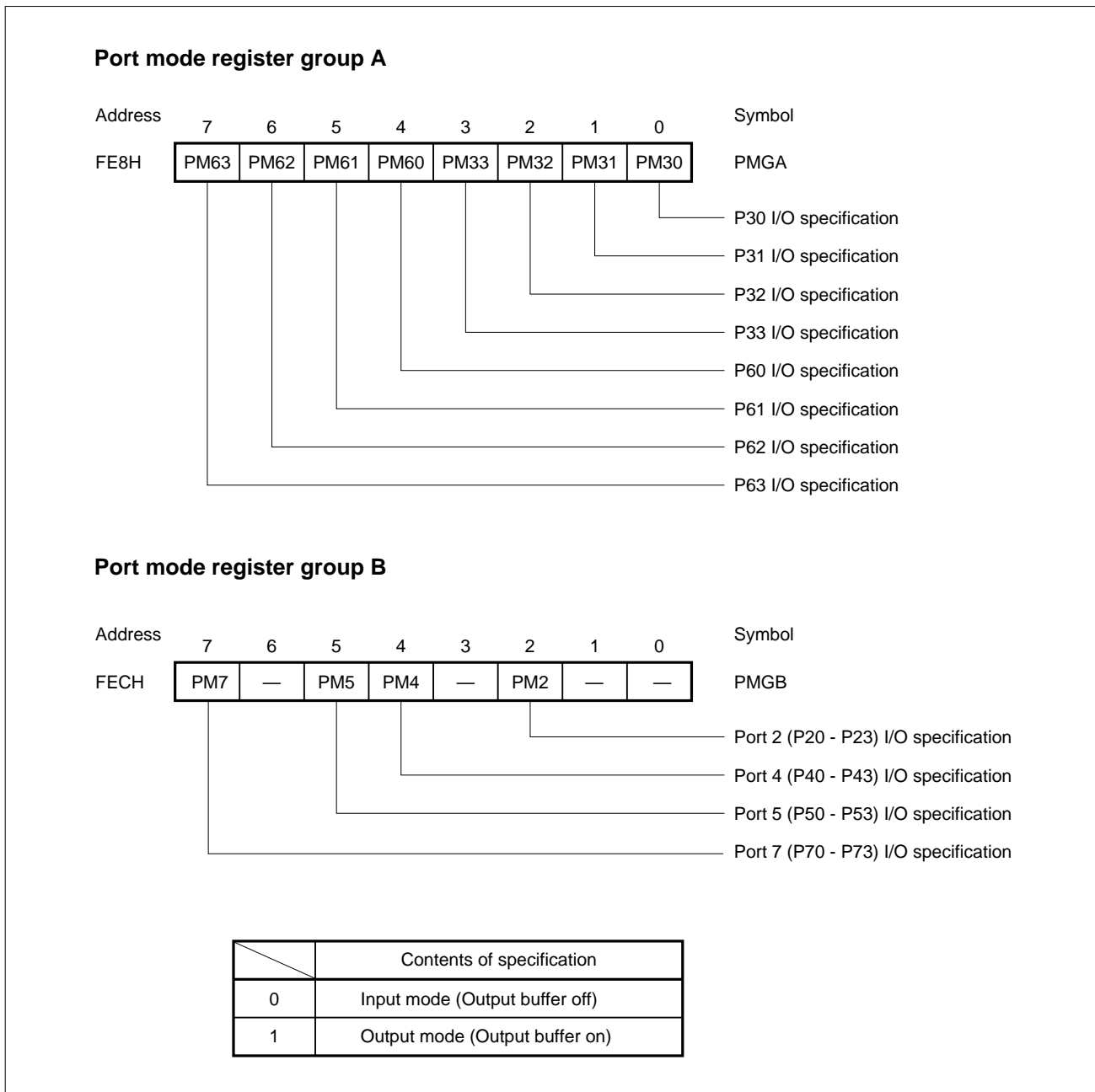
Figure 5-9. Formats of Port Mode Registers (1/2)
