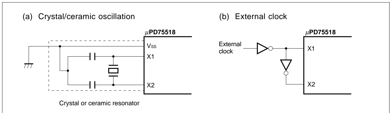
Figure 5-16. External Circuit for the Main System Clock Oscillator
