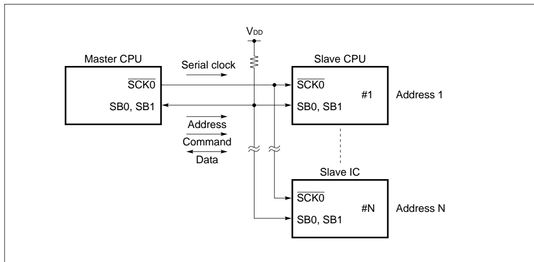
Figure 5-39. Example of the SBI System Configuration
