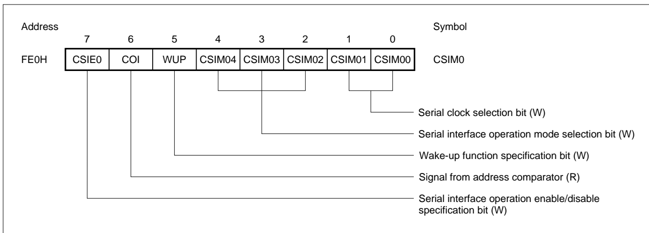
Figure 5-41. Format of Serial Operation Mode Register 0 (CSIM0) (1/3)
