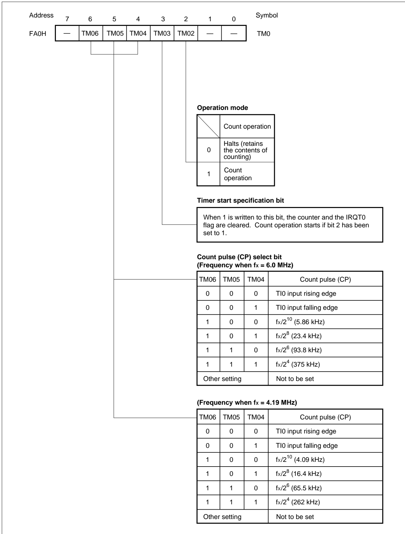
Figure 5-29. Format of the Timer/Event Counter Mode Register
