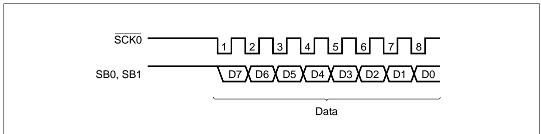
Figure 5-58. Data
