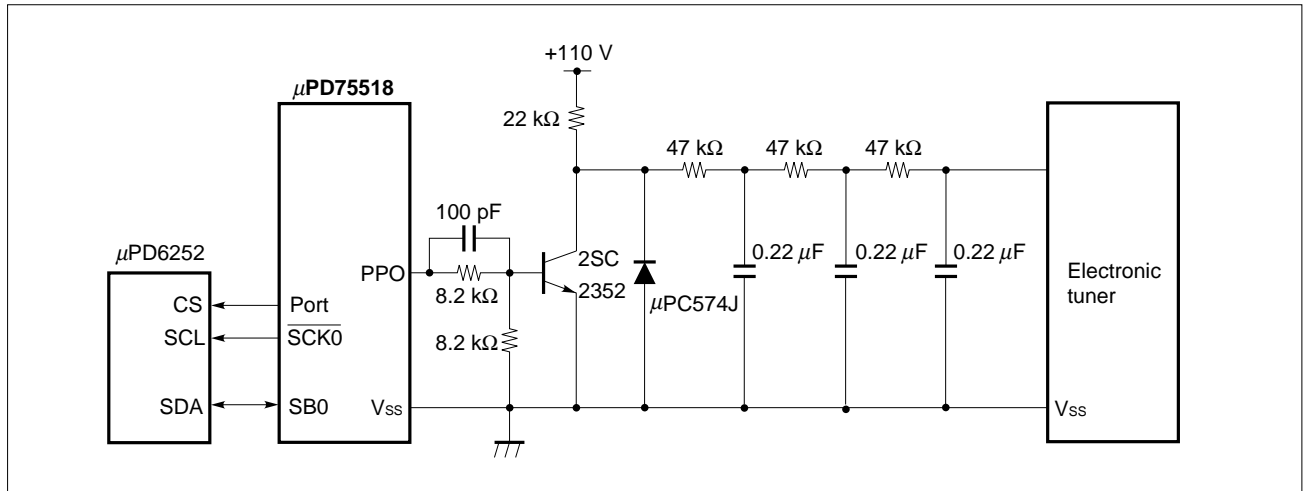
Figure 5-38. Sample Circuit Applicable to TV Tuners *
