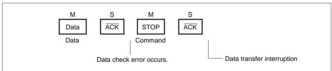
Figure 5-75. Transfer Format of the STOP Command
