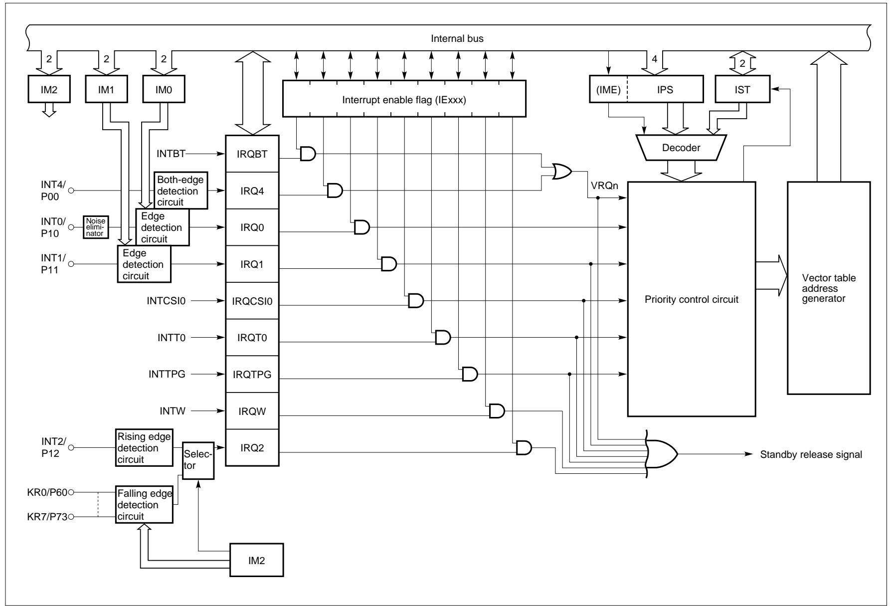
Figure 6-1. Block Diagram of Interrupt Control Circuit
