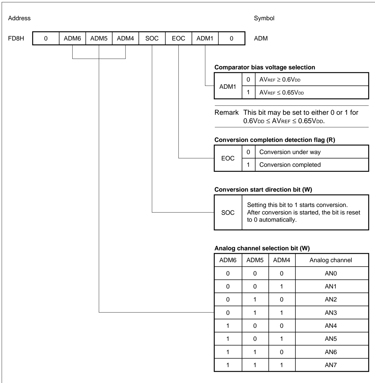
Figure 5-86. Format of the A/D Conversion Mode Register
