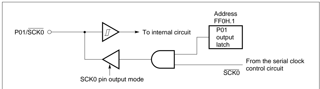
Figure 5-81. \overline{SCK0}/P01 Pin Circuit Configuration
