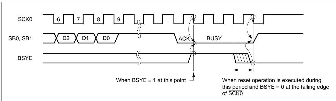
Figure 5-66. Operation of BSYE
