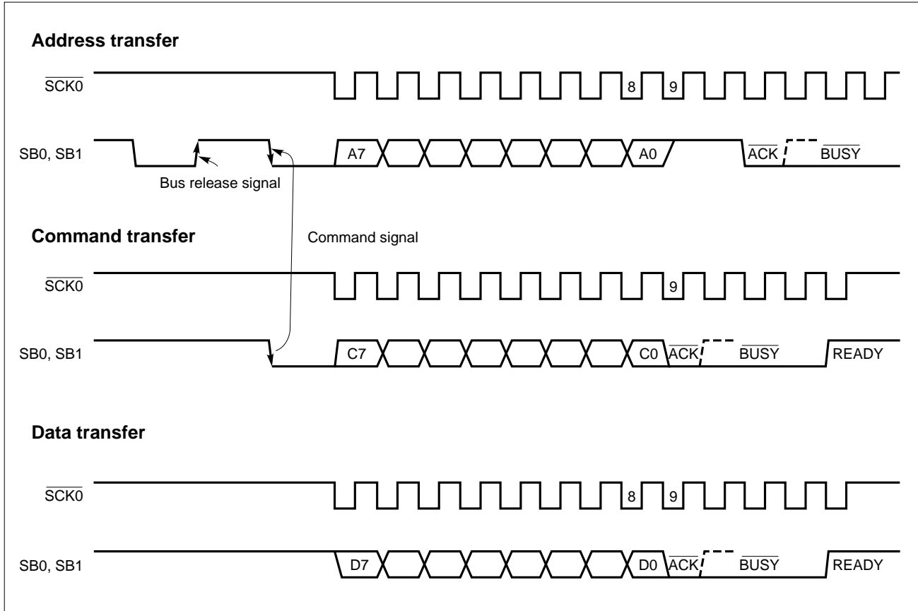
Figure 5-52. Timing of SBI Transfer
