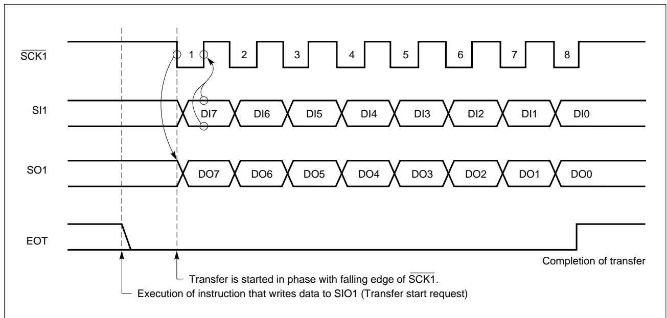
Figure 5-84. Timing of the Three-wire Serial I/O Mode
