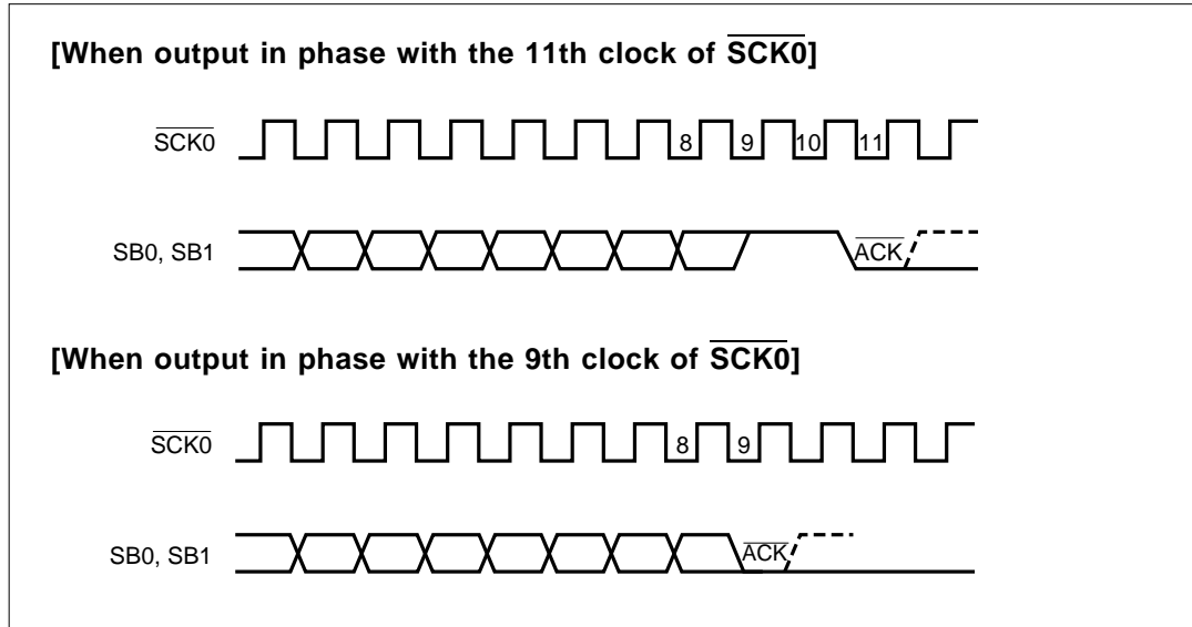
Figure 5-59. Acknowledge Signal
