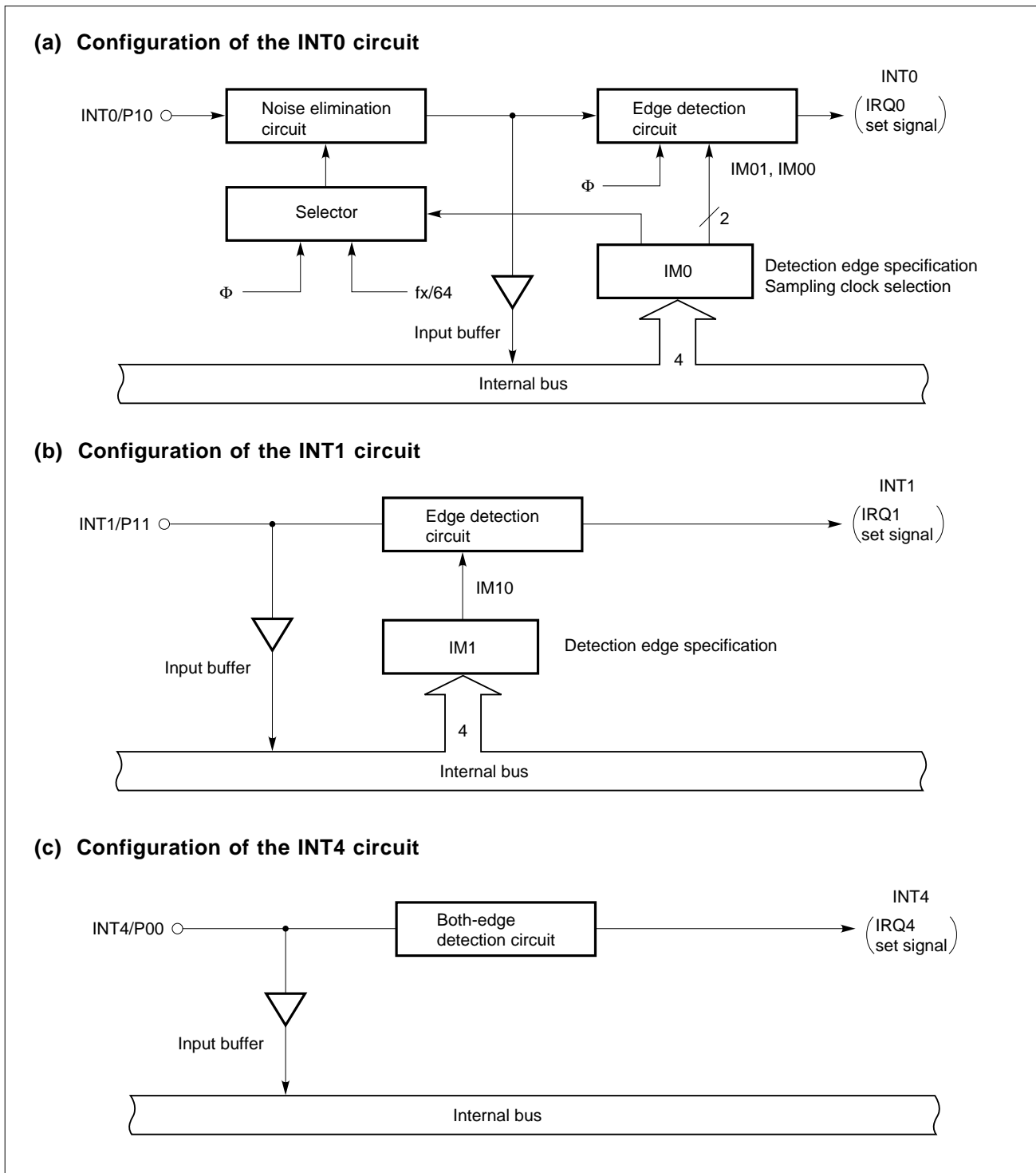
Figure 6-3. Configurations of the INT0, INT1, and INT4 Circuits
