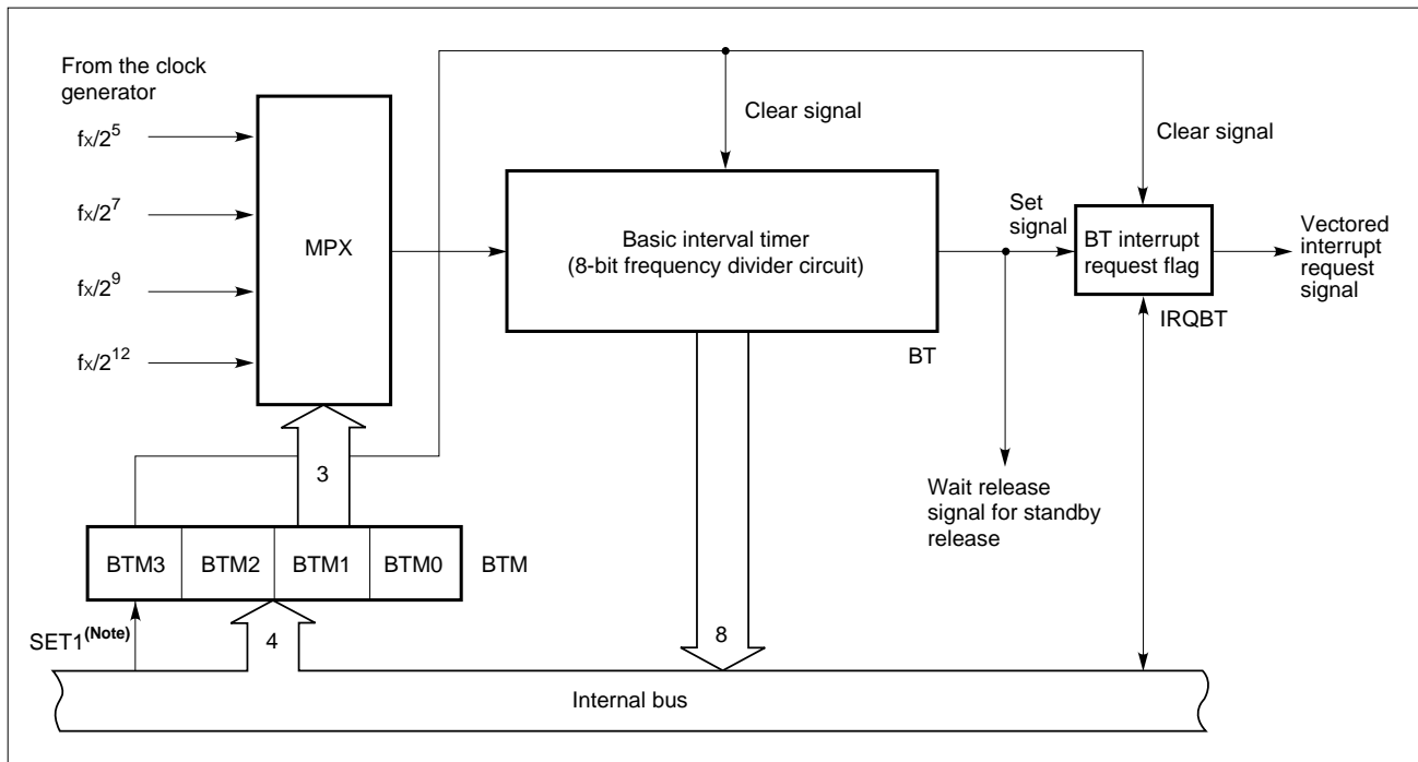
Figure 5-23. Configuration of the Basic Interval Timer
