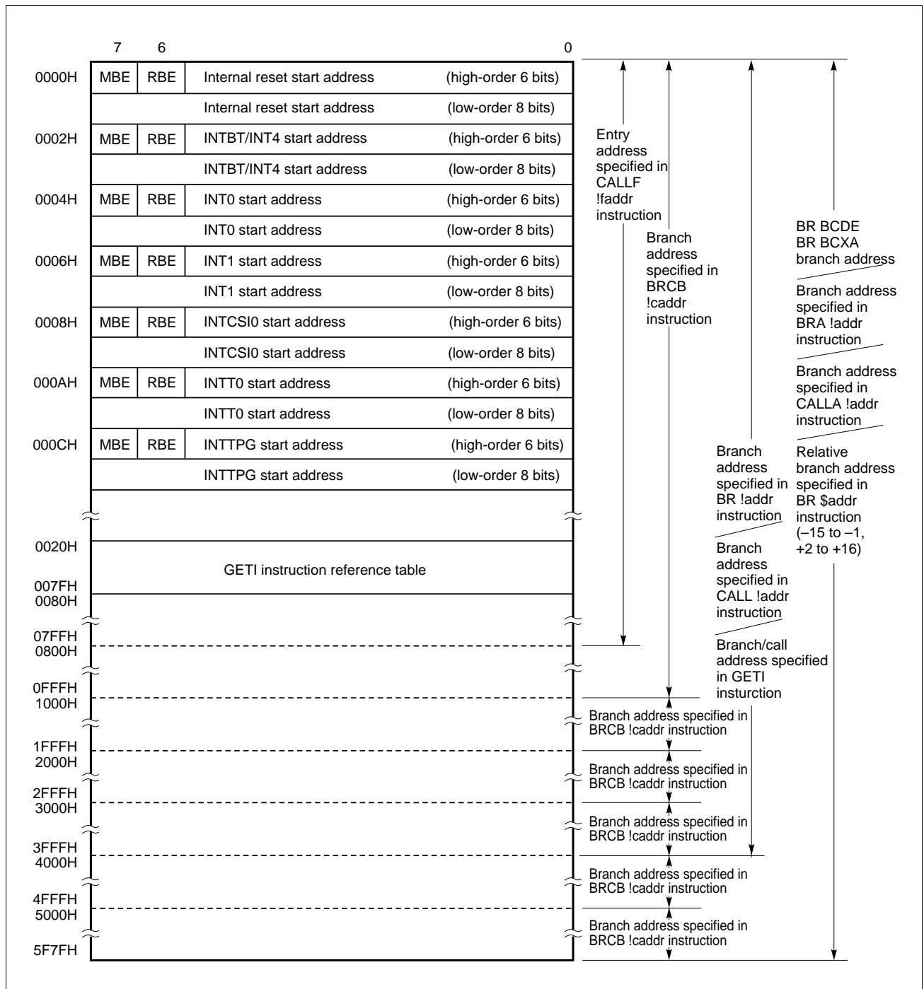
Figure 4-2. Program Memory Map ( \mu PD75517)
