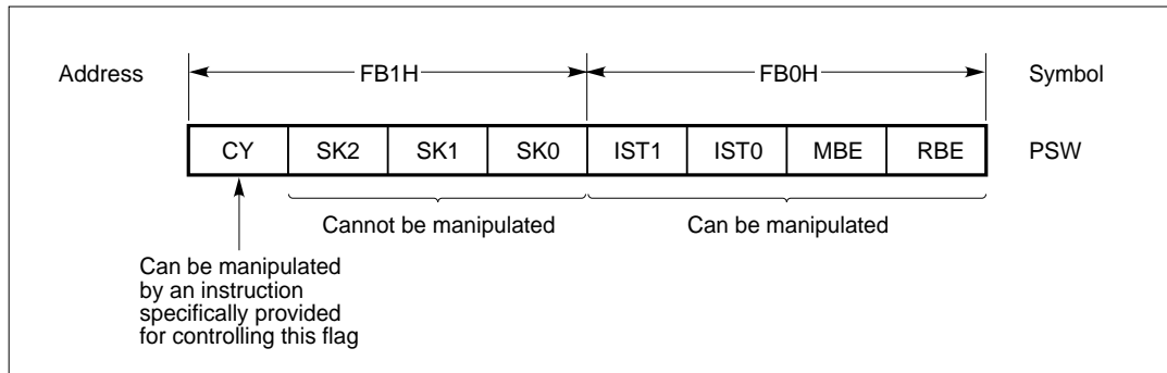
Figure 4-11. Program Status Word Format
