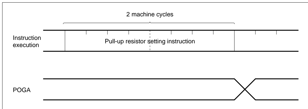
Figure 5-11. ON Timing of Pull-up Resistors by Software
