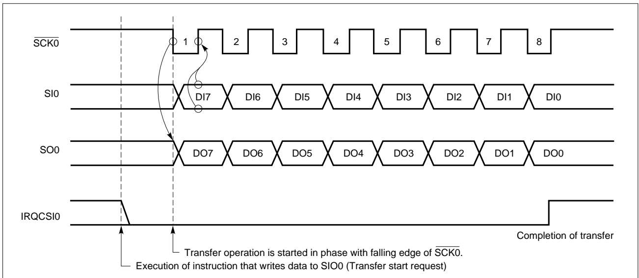
Figure 5-45. Timing of Three-Wire Serial I/O Mode
