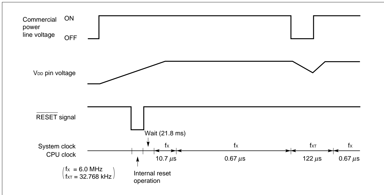
Figure 5-19. Changing the System Clock and CPU Clock
