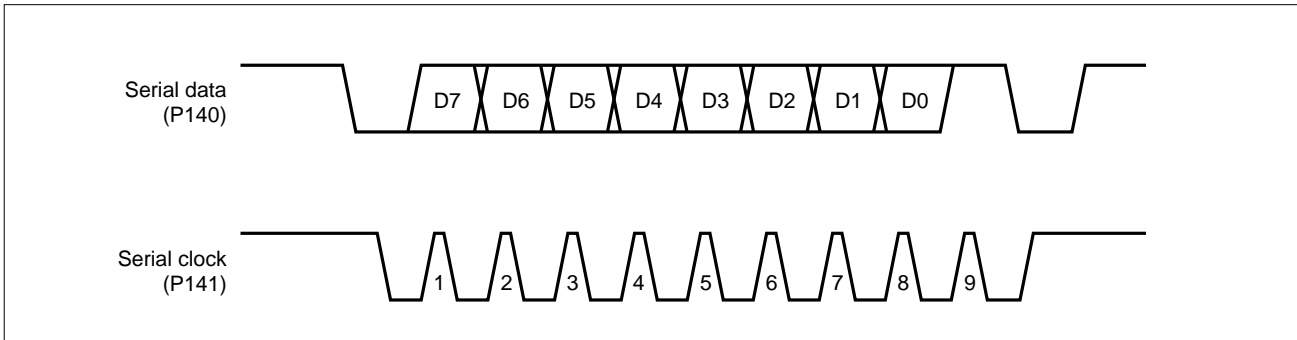
Figure 5-92. Serial Transfer Format (I)
