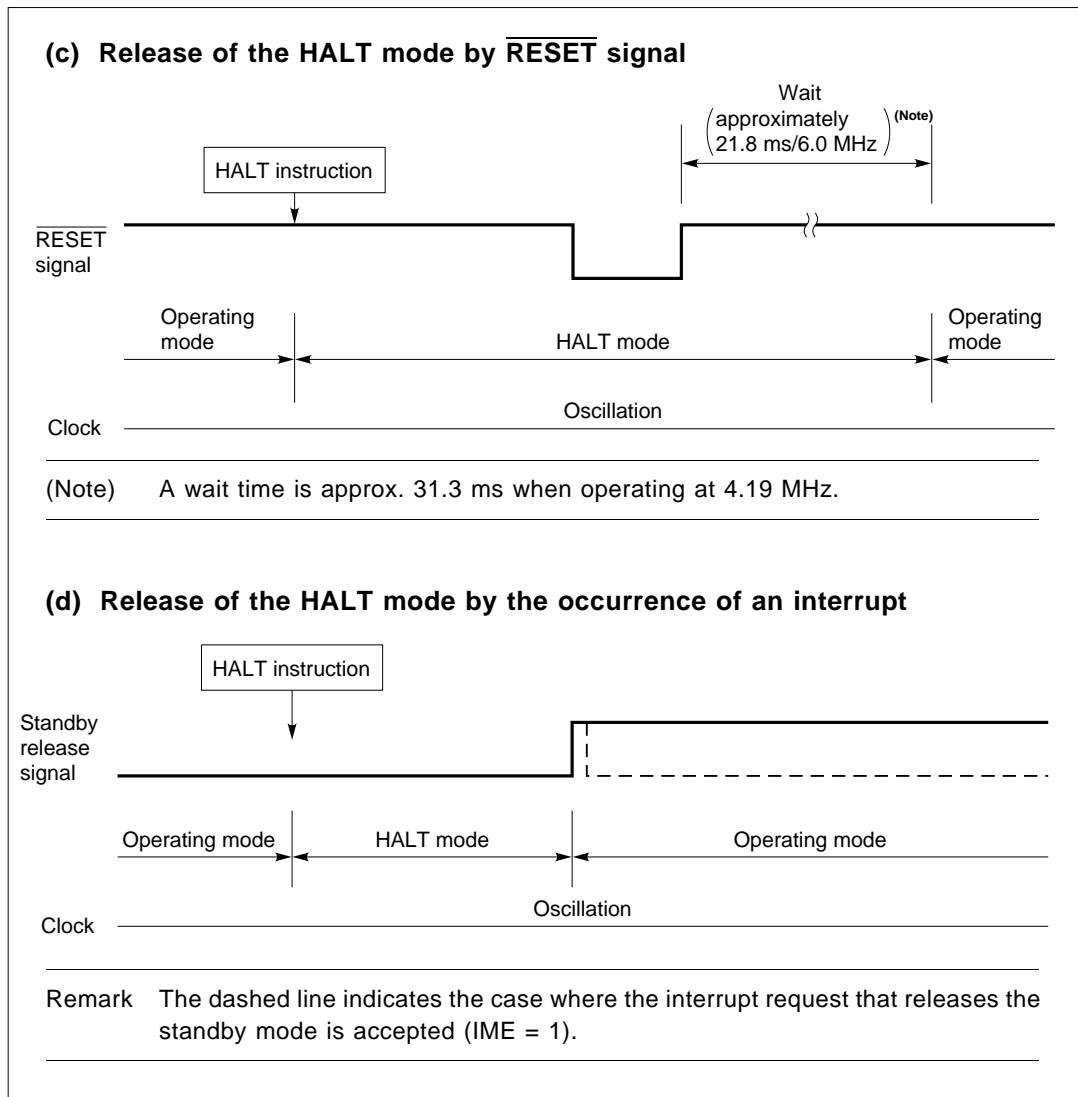
Figure 7-1. Standby Mode Release Operation (2/2)
