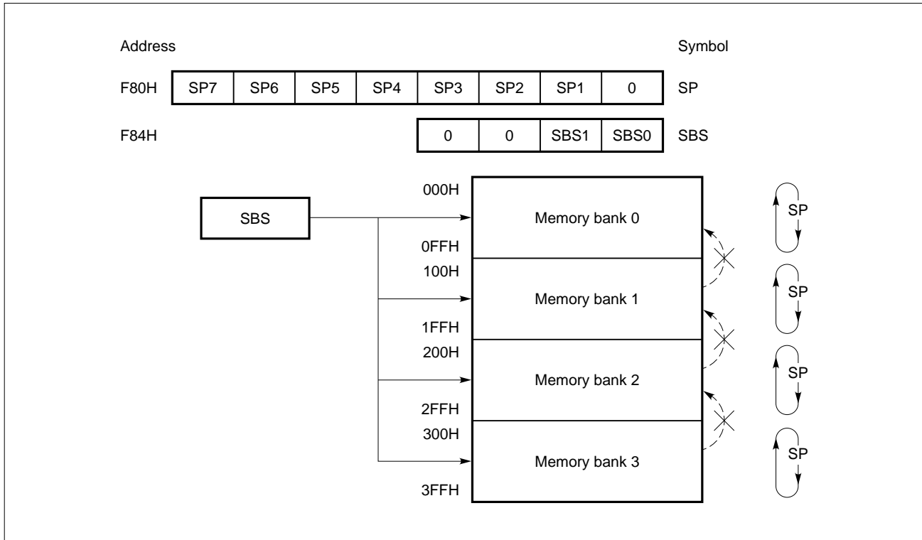
Figure 4-8. Format of Stack Pointer and Stack Bank Select Register
