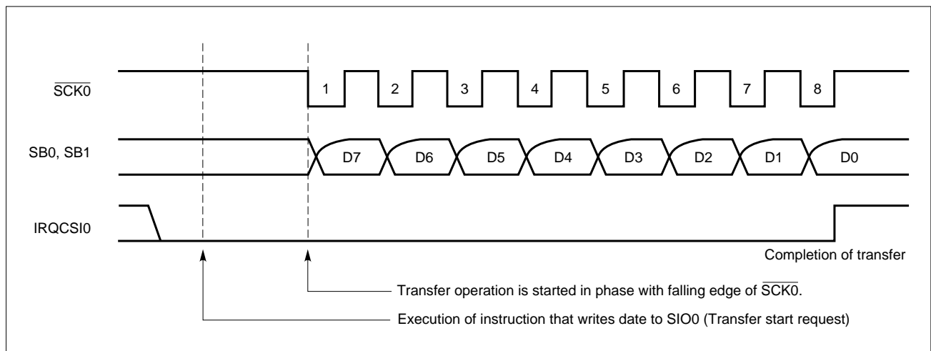
Figure 5-49. Timing of Two-Wire Serial I/O Mode
