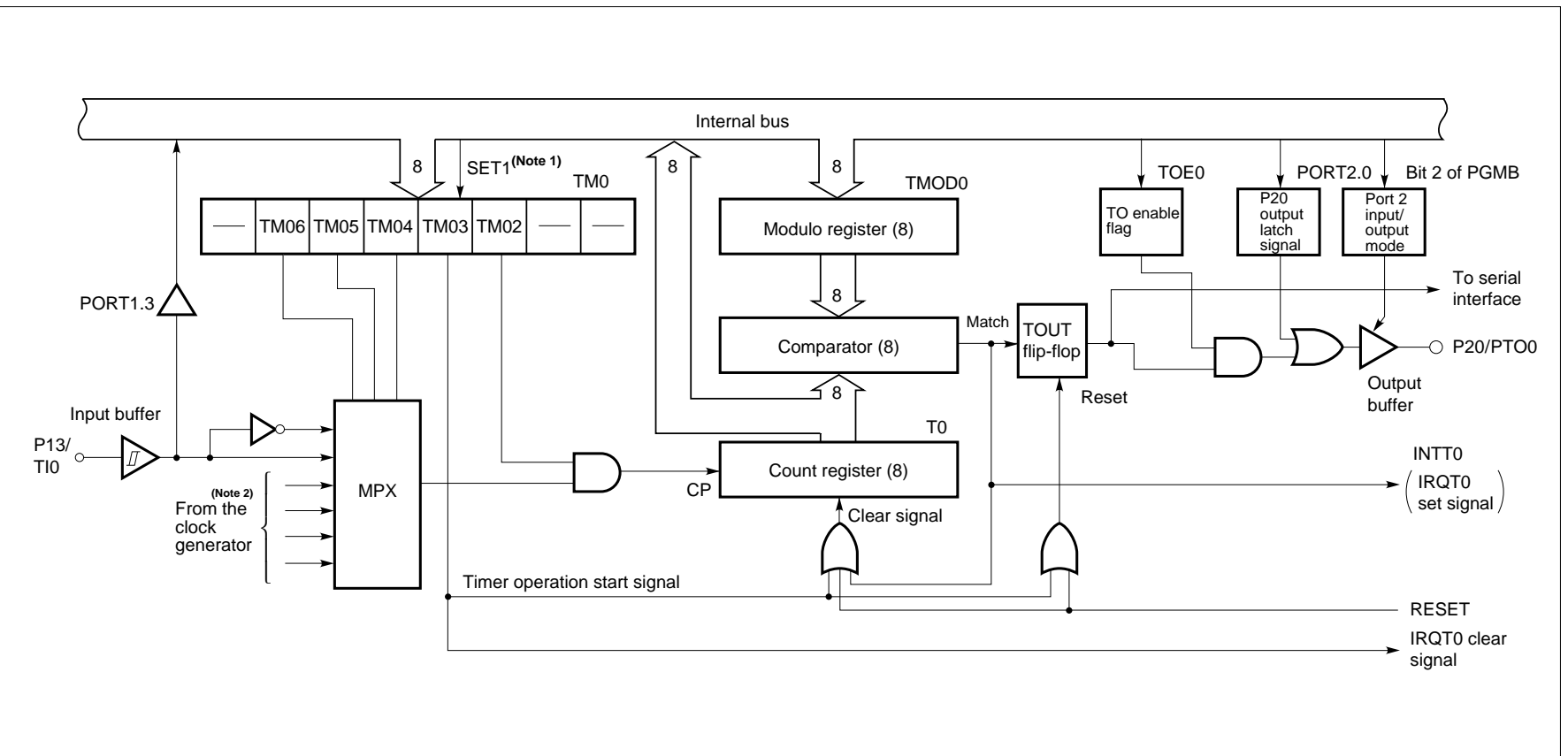
Figure 5-27. Block Diagram of the Timer/Event Counter
