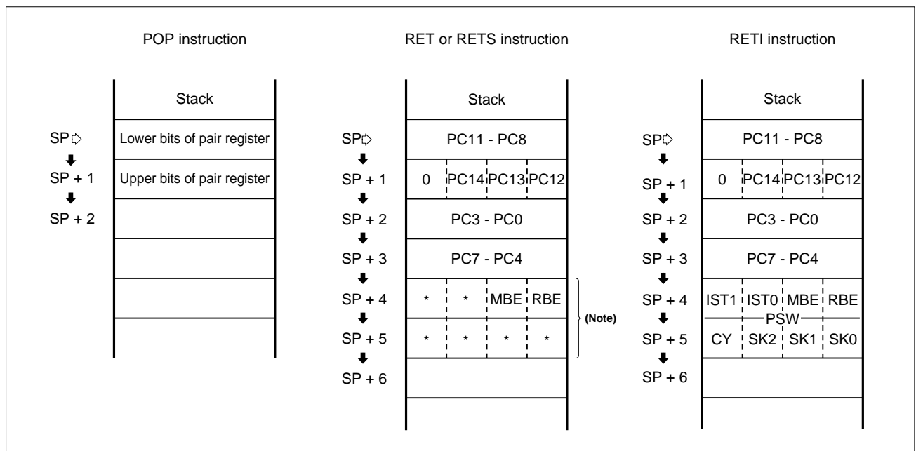
Figure 4-10. Data Restored from Stack Memory
