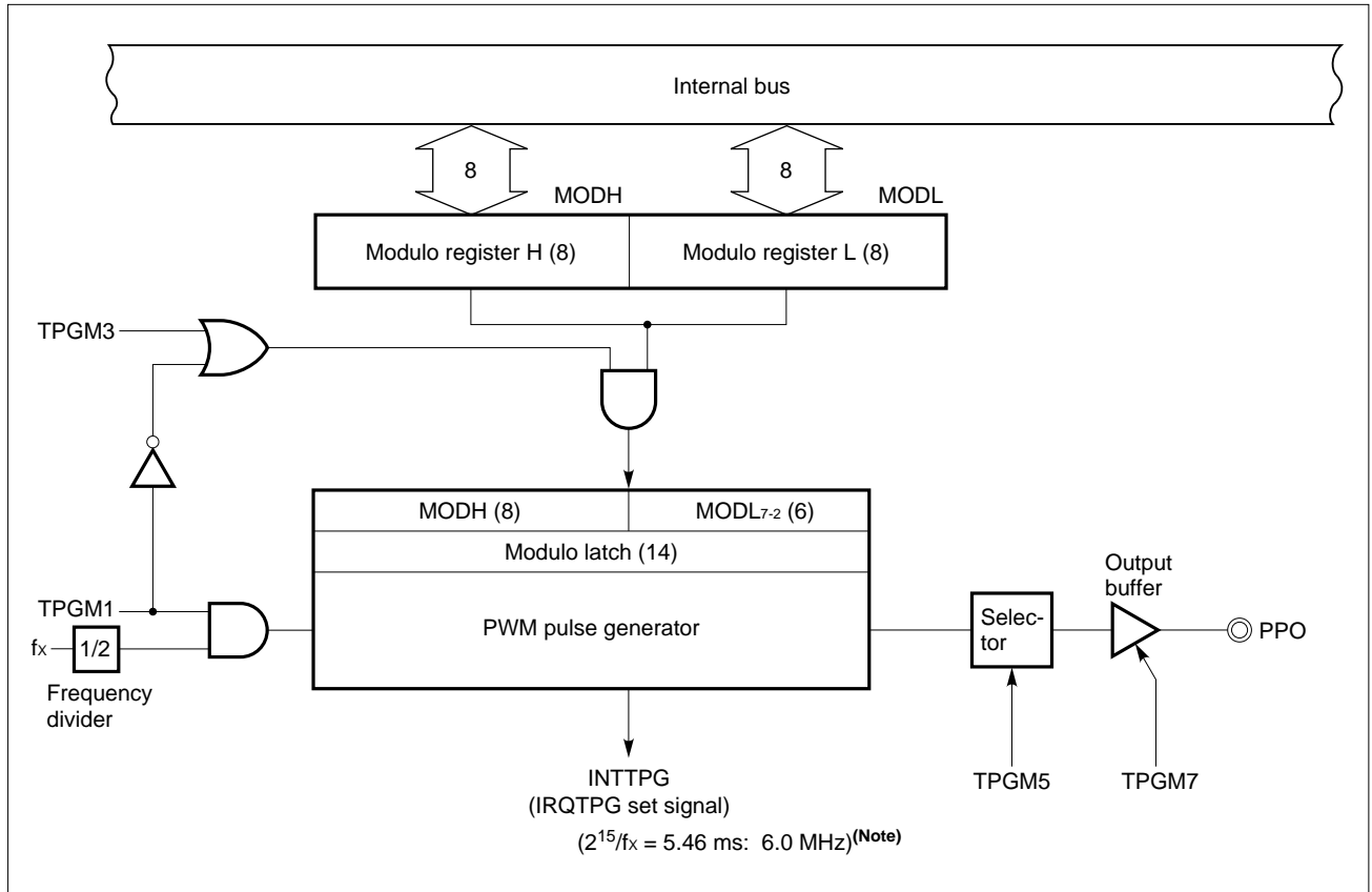
Figure 5-36. Block Diagram of the Timer/Pulse Generator (PWM Pulse Generation Mode)
