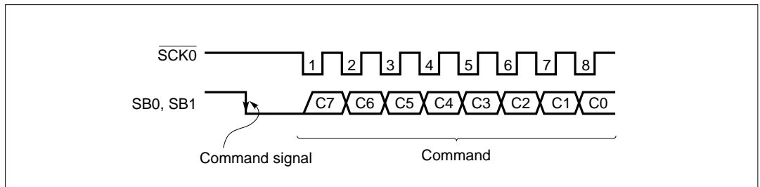
Figure 5-57. Command
