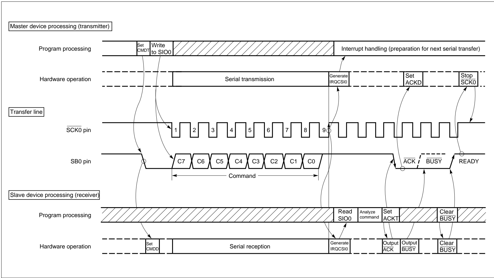
Figure 5-69. Command Transfer Operation from Master Device to Slave Device
