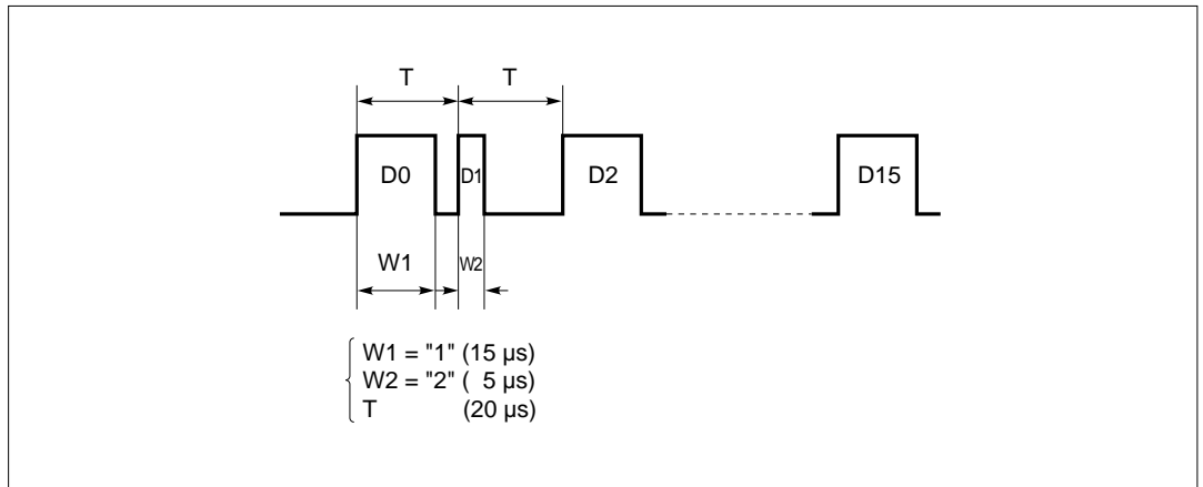
Figure 5-93. Serial Transfer Format (II)
