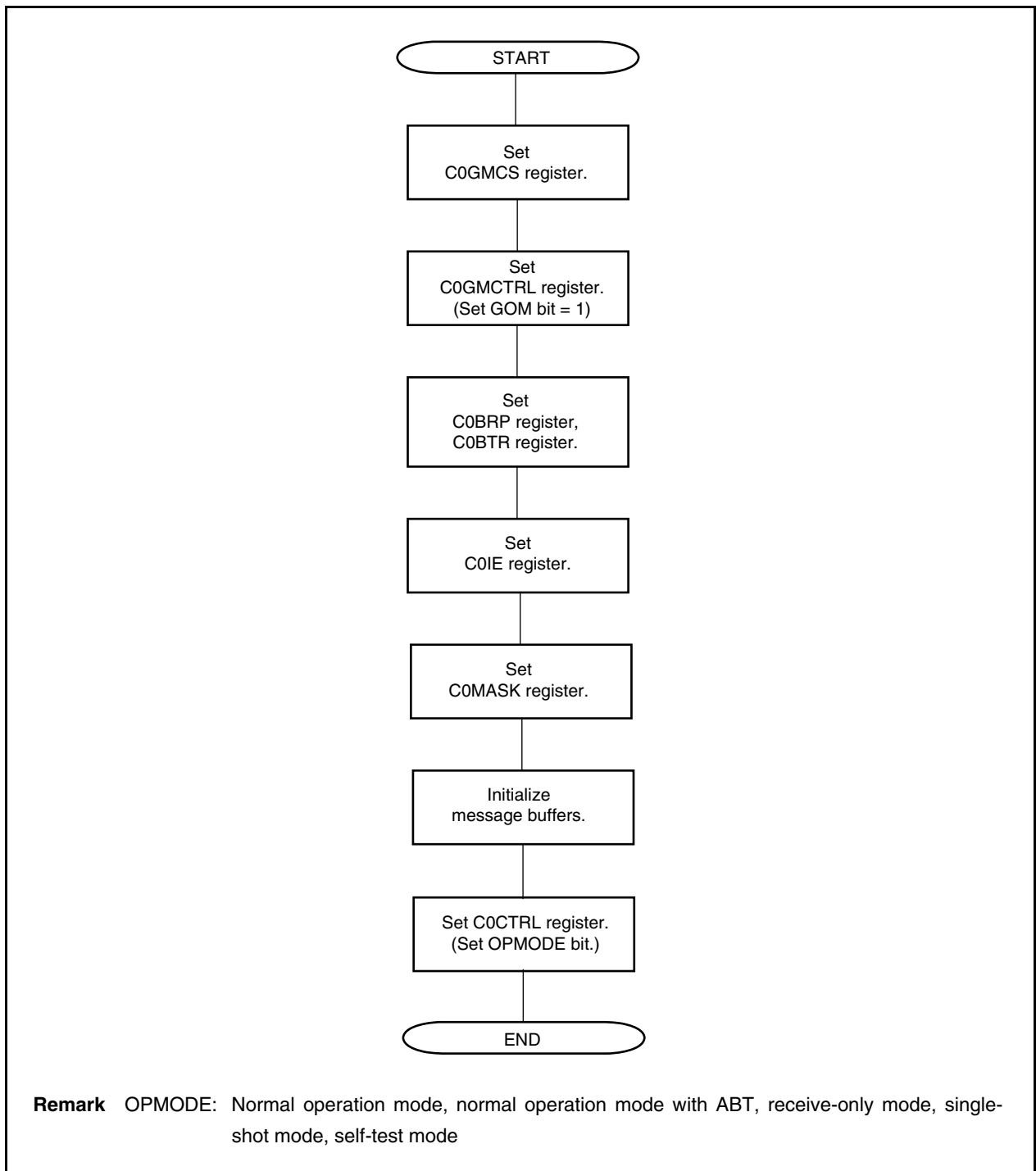
Figure 19-36. Initialization
