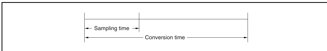
Figure 13-22. Sampling Time
