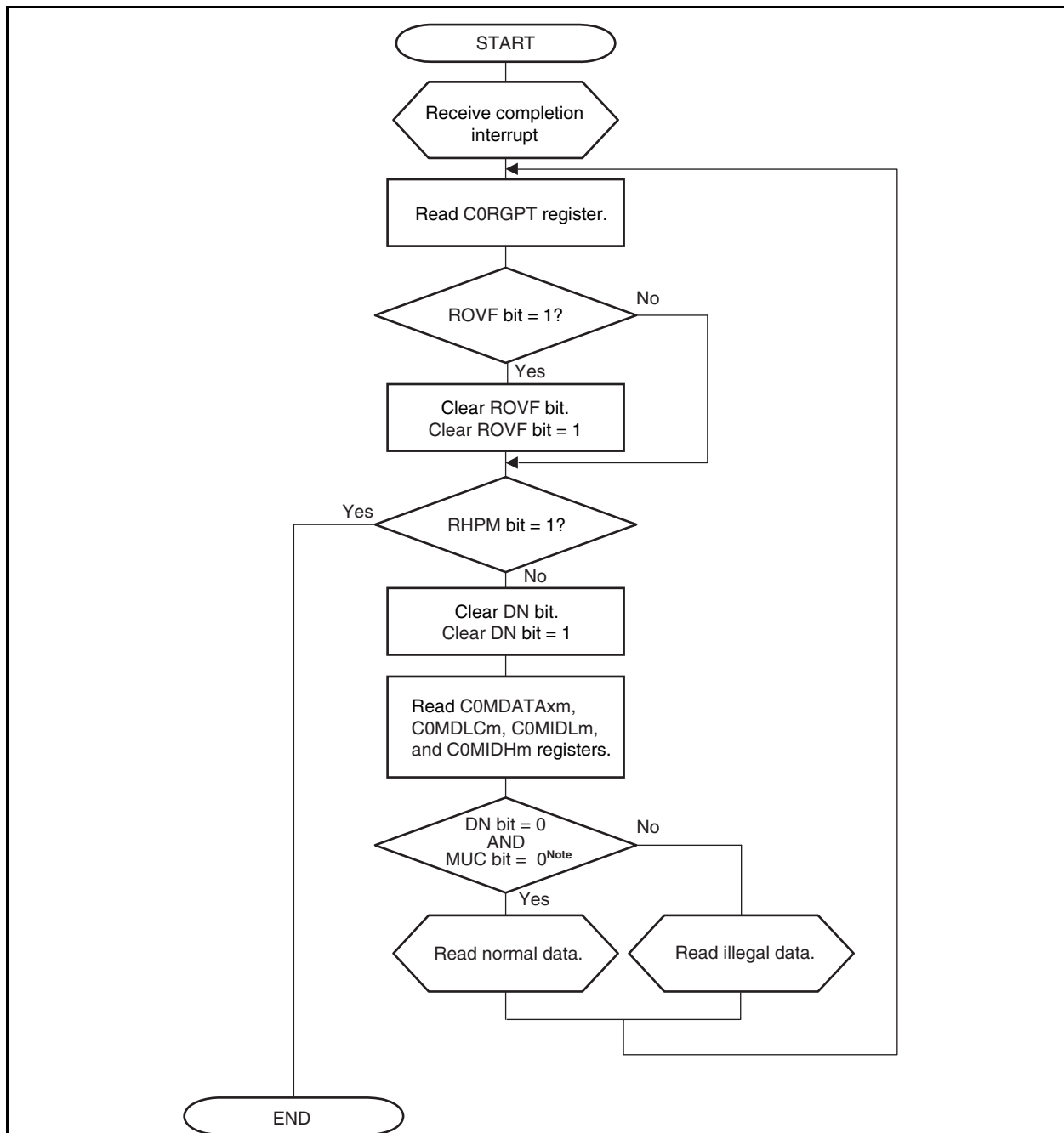
Figure 19-50. Reception via Interrupt (Using C0RGPT Register)
