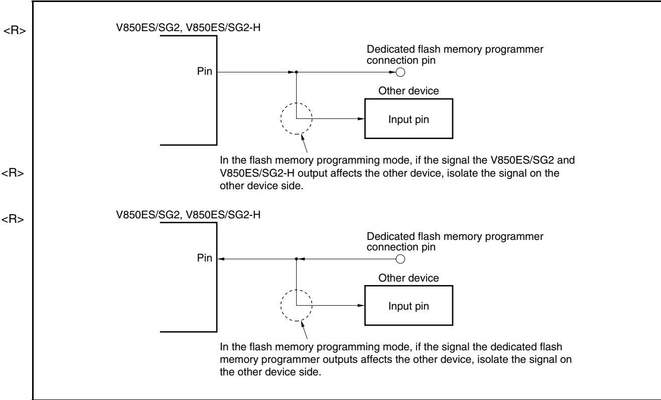
Figure 30-14. Malfunction of Other Device
