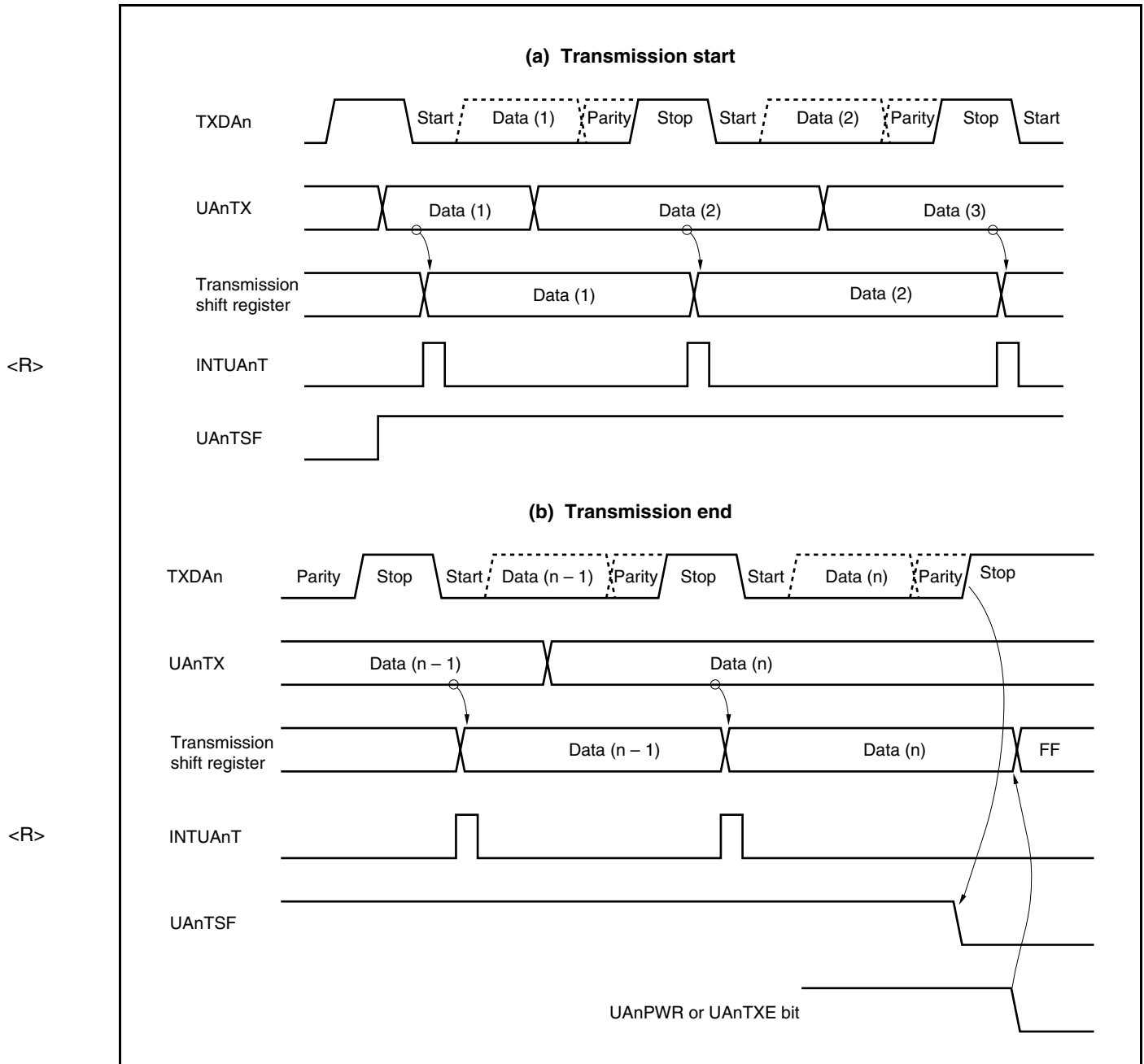
Figure 15-12. Continuous Transmission Operation Timing
