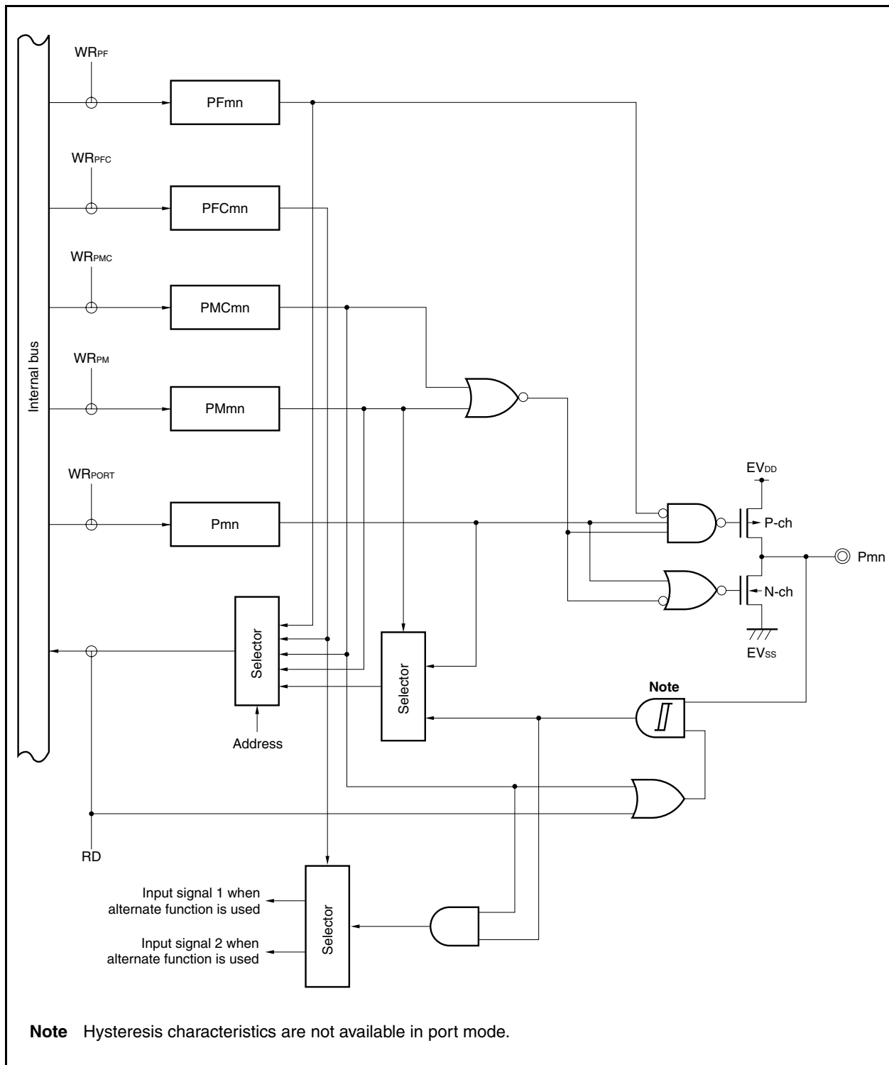
Figure 4-12. Block Diagram of Type G-4
