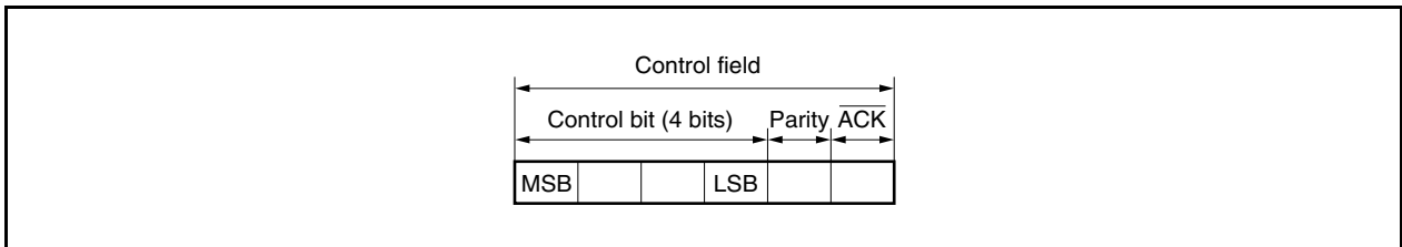
Figure 18-4. Control Field
