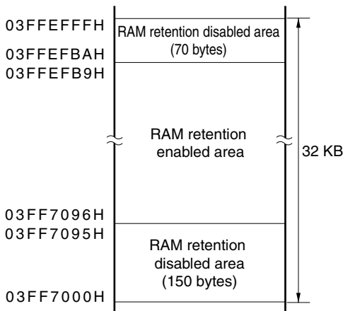
(a) Version with 32 KB RAM
