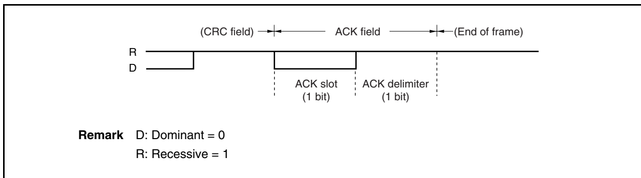
Figure 19-11. ACK Field
