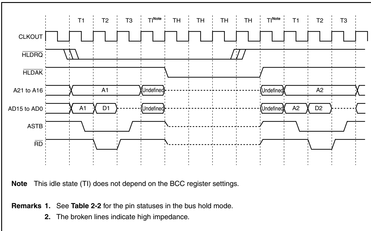
Figure 5-8. Multiplexed Bus Hold Timing (Bus Size: 16 Bits, 16-Bit Access)
