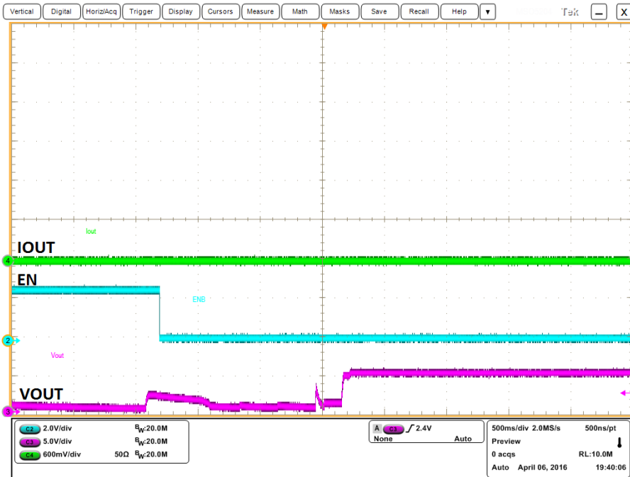
Figure 13. No Load Start-up by Rx Enable Signal (Ch2=EN, Ch3=Vout, Ch4=Iout)
