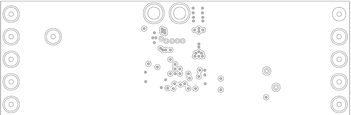
Figure 22. P9027LP-R-EVK Layout (Bottom Layer)
