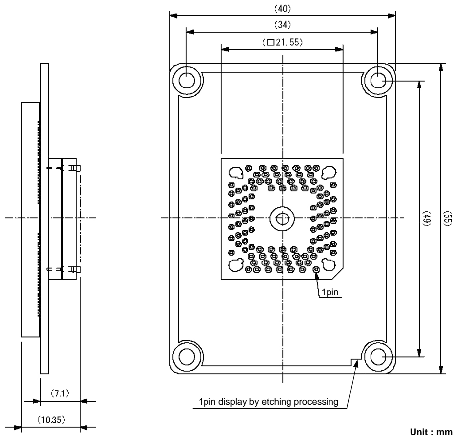
<Bottom view>
