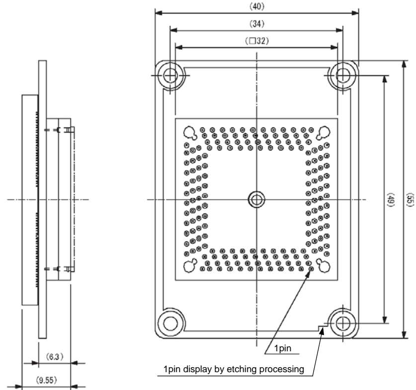
<Bottom view>
