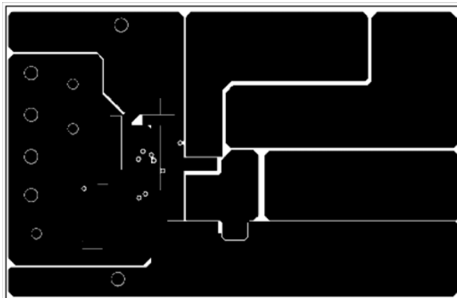
FIGURE 20. ISL6420BEVAL1Z - LAYER 3
