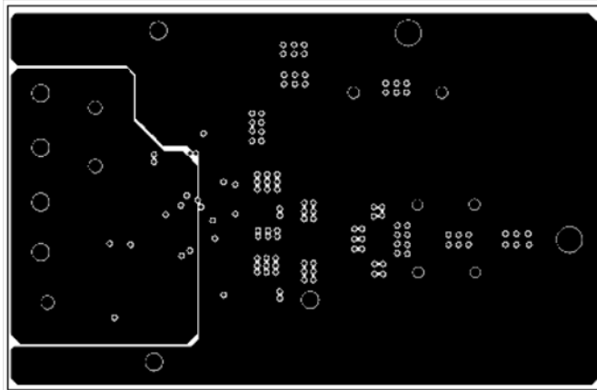
FIGURE 19. ISL6420BEVAL1Z - LAYER 2
