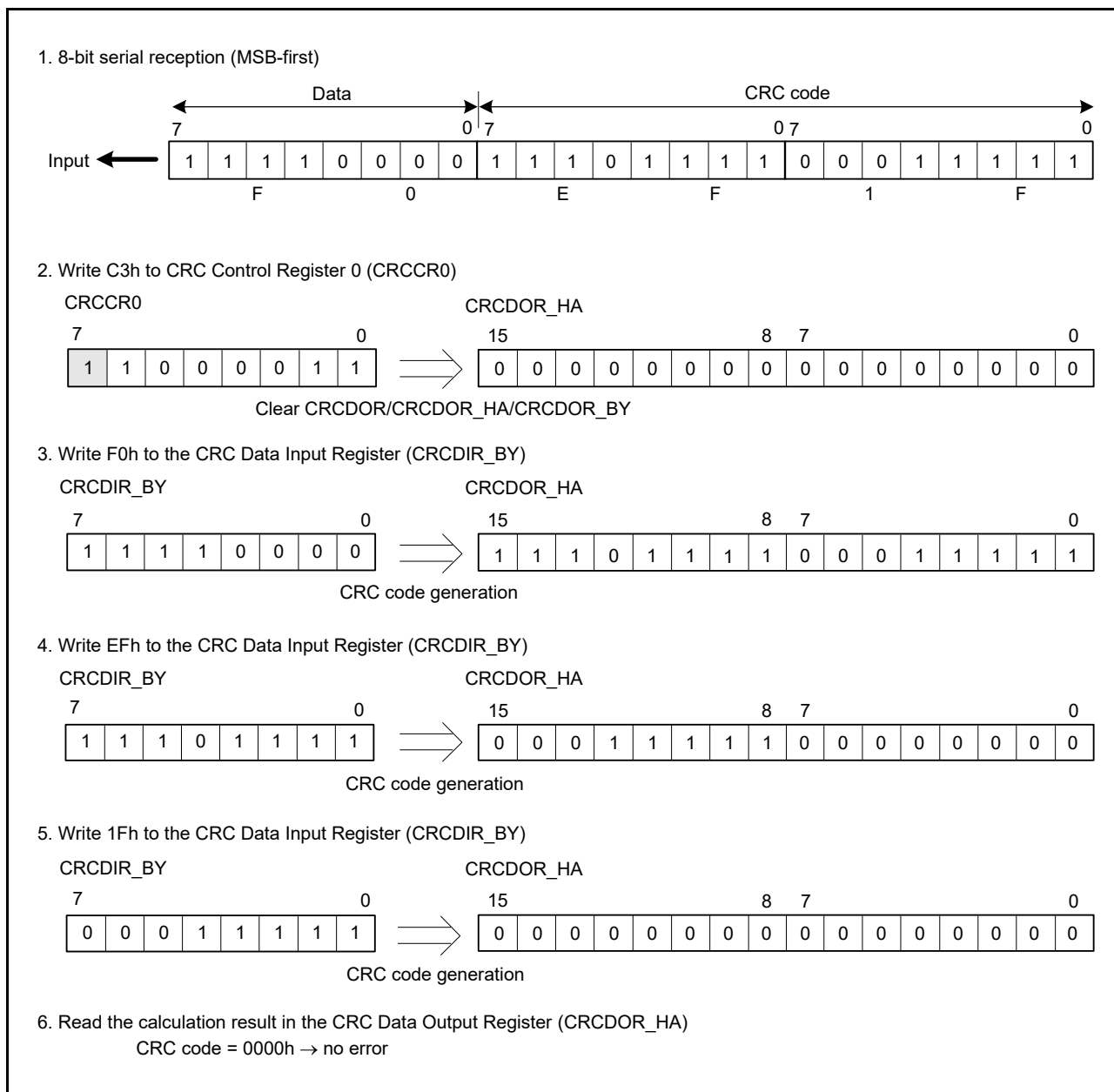
Figure 33.5 MSB-first data reception
