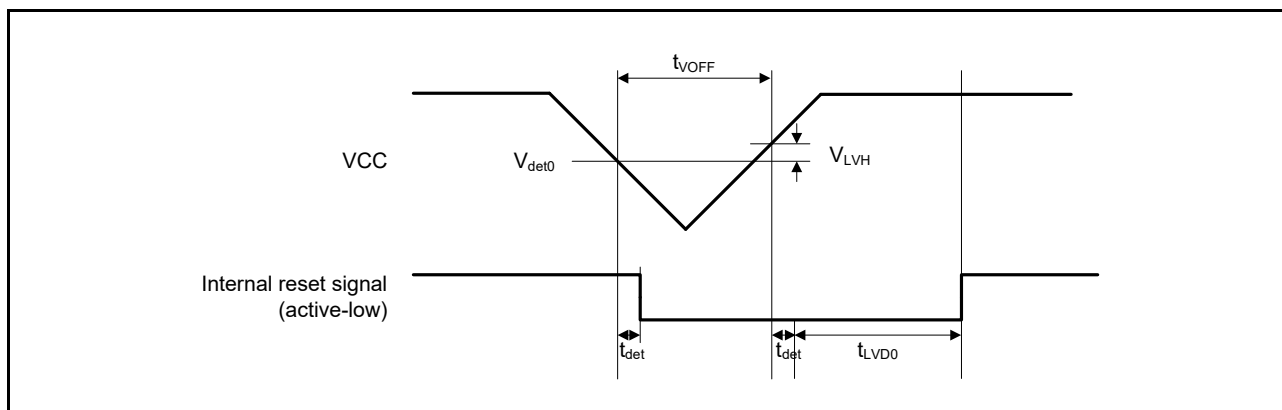
Figure 48.70 Voltage detection circuit timing ( V_{det0} )
