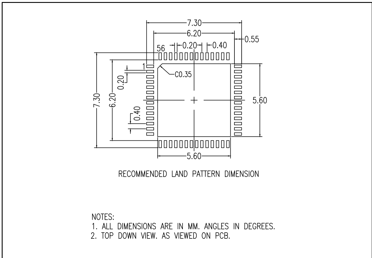
Figure 2.2 Land Pattern
