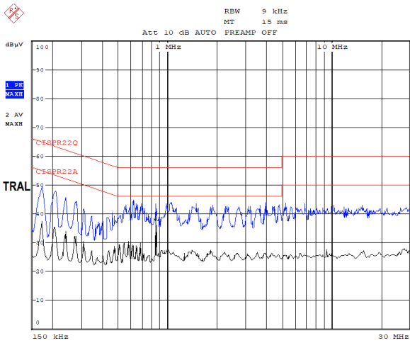
Figure 11. Neutral, 120V AC
