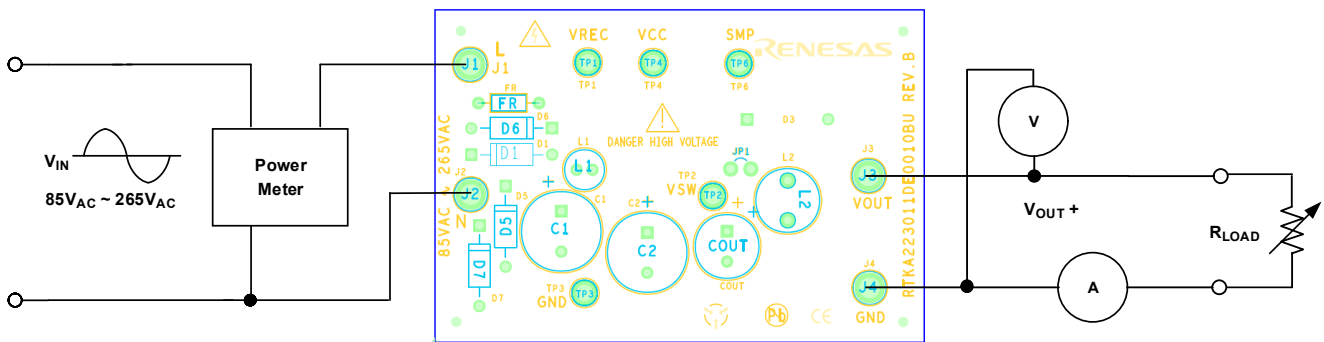
Figure 1. RTKA223011DE0010BU Connection Diagram
