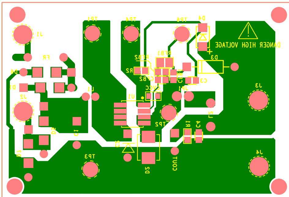
Figure 6. Bottom Layer
