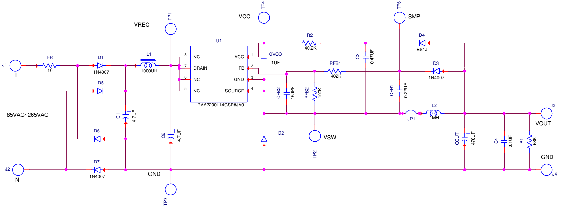
Figure 4. RTKA223011DE0010BU Schematic
