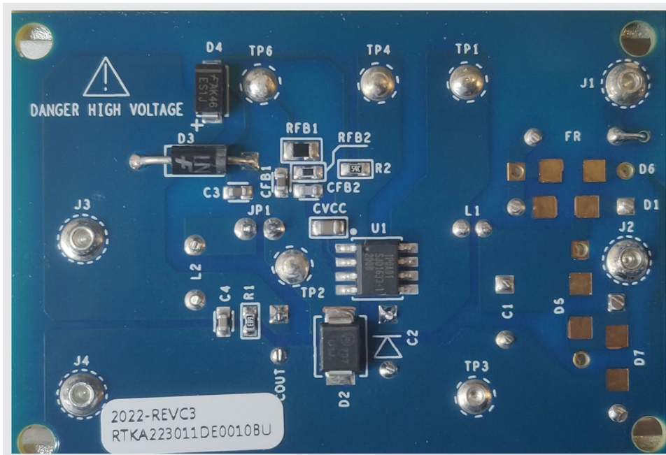
Figure 3. RTKA223011DE0010BU Evaluation Board (Bottom)
