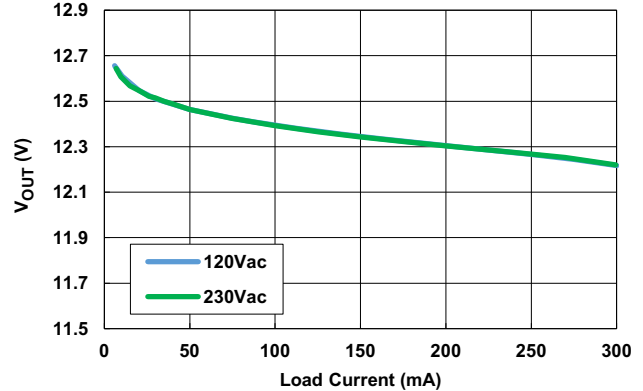
Figure 8. Load Regulation
