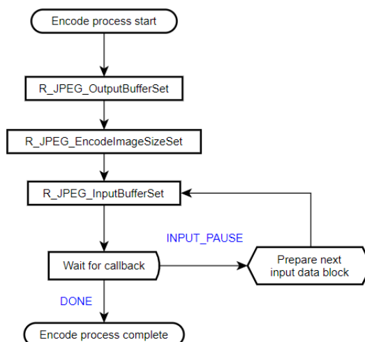
Figure 212: JPEG Encode Operational Flow
