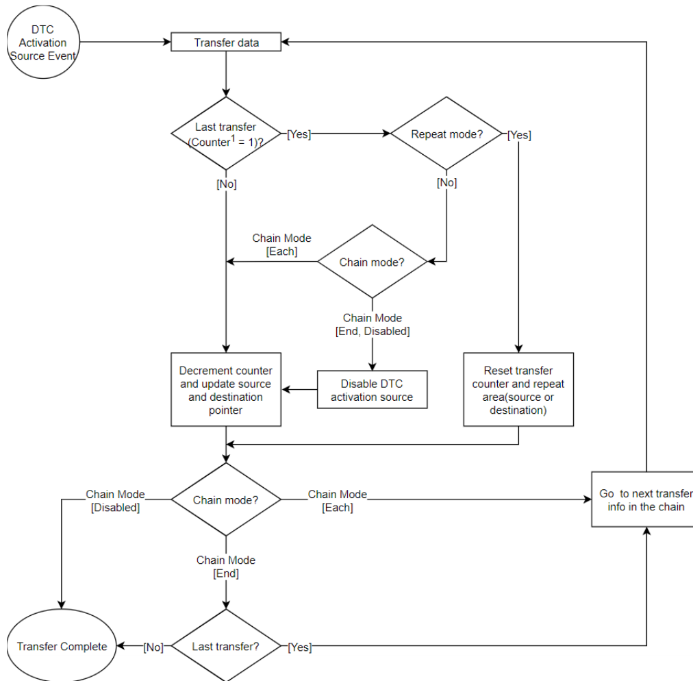
Figure 242: DTC Transfer Flowchart
