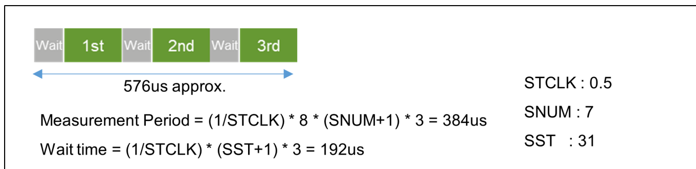
Figure 156: Self-capacitance Measurement Period (CTS2U)
