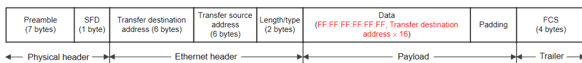
Figure 223: Magic Packet Frame Format Image
