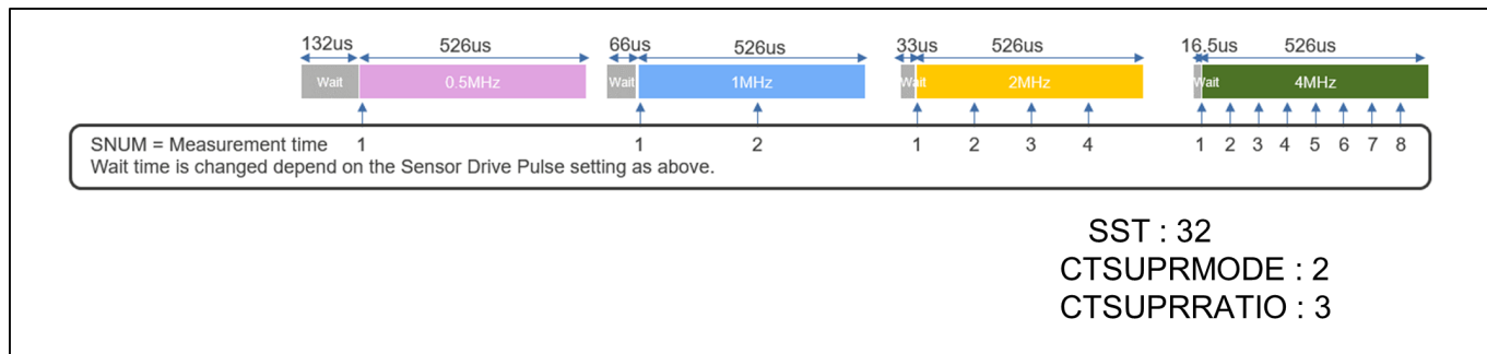
Figure 155: Self-capacitance Measurement Period (CTS1U1)
