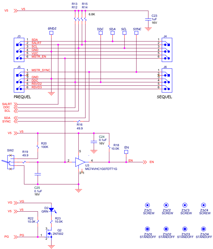
Figure 6. Schematic - Page 3
