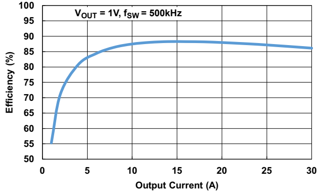
Figure 16. Efficiency
