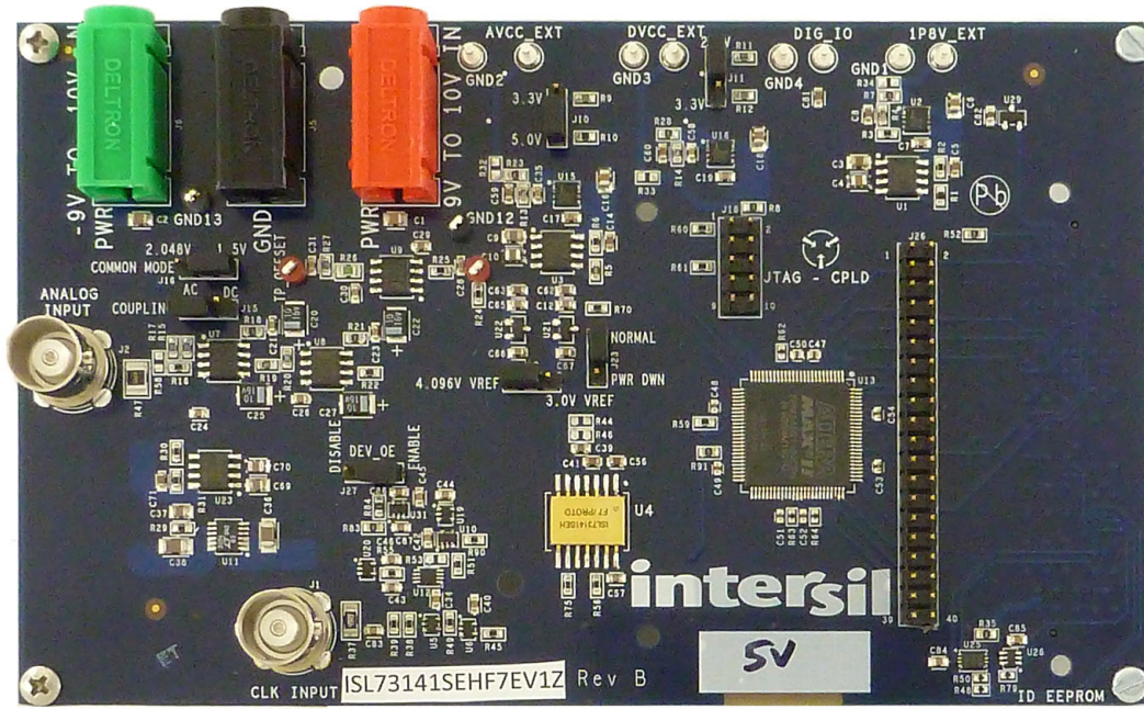
Figure 11. ISL73141SEHF7EV1Z Evaluation Board (Top)
