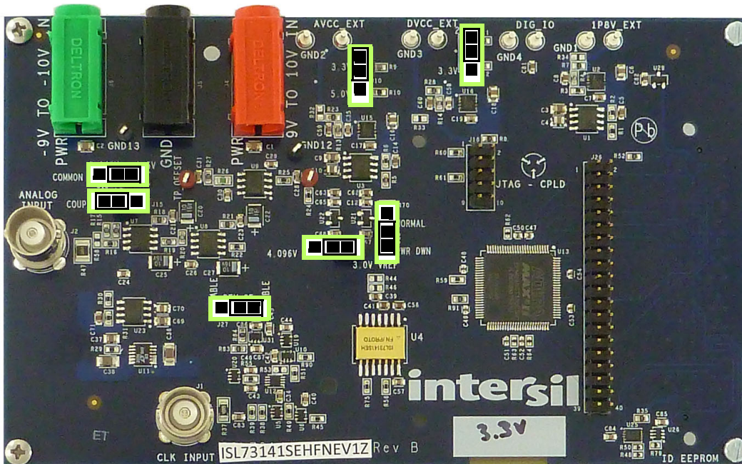
Figure 2. ISL73141SEHFNEV1Z Evaluation Board Jumper Location
