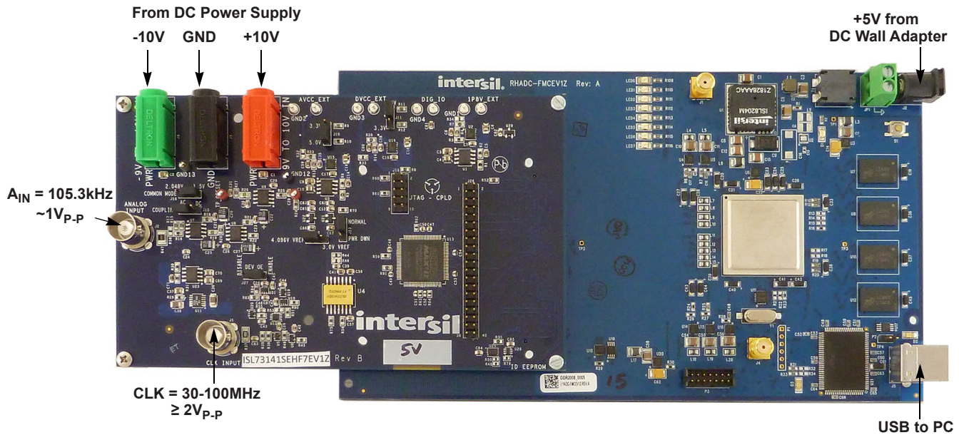
Figure 4. ISL73141SEHF7EV1Z/RHADC-FMCEV1Z Connection Diagram
