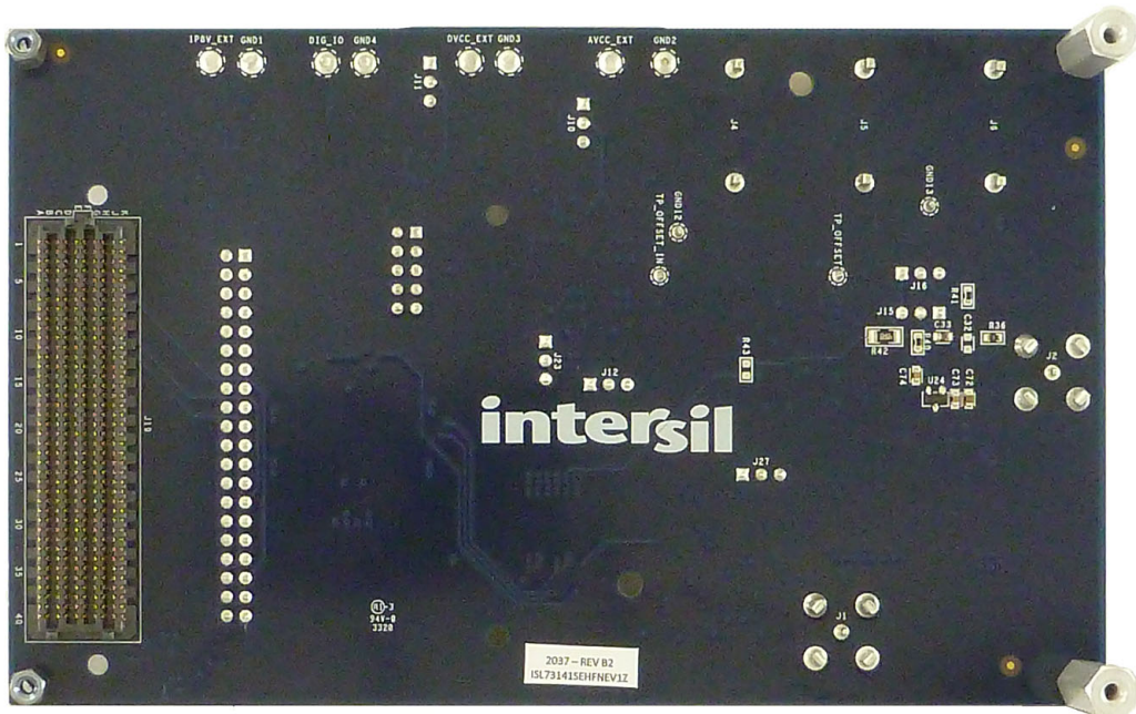
Figure 14. ISL73141SEHFNEV1Z Evaluation Board (Bottom)
