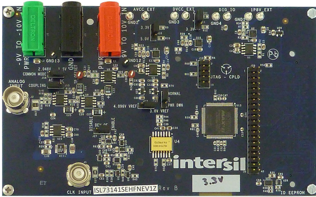
Figure 13. ISL73141SEHFNEV1Z Evaluation Board (Top)
