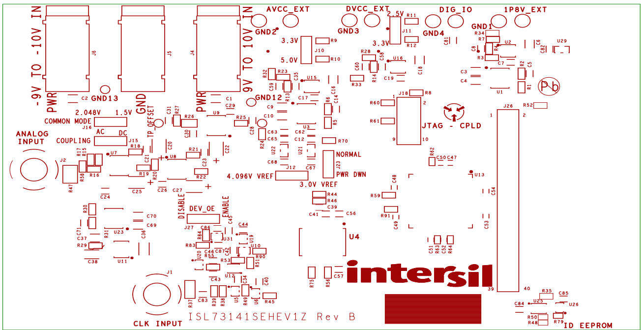
Figure 21. Top Silkscreen
