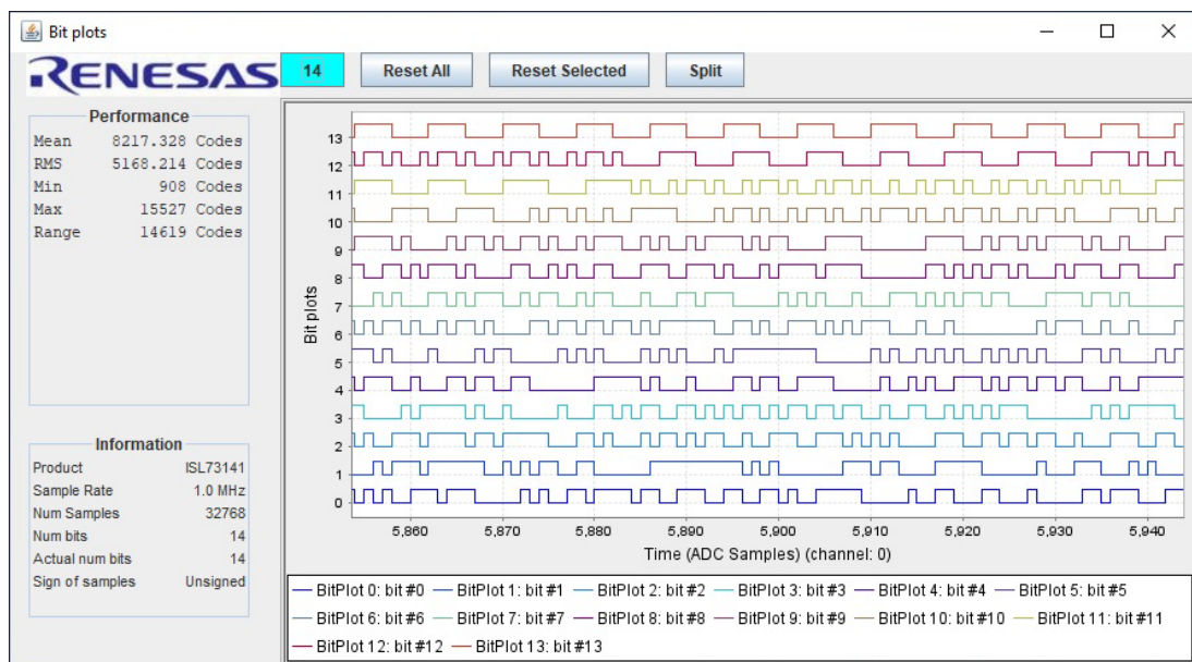
Figure 9. iRADAnalyzer Time Domain Bit Plot
