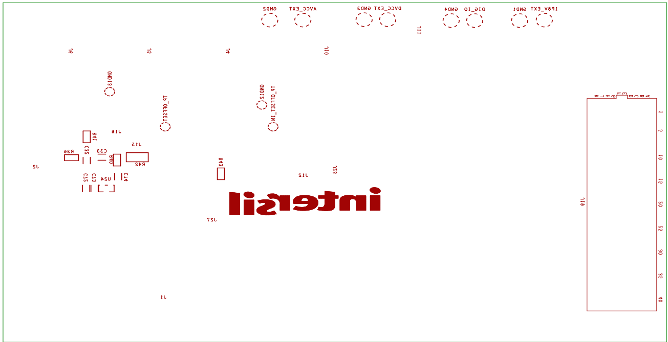
Figure 30. Bottom Silkscreen
