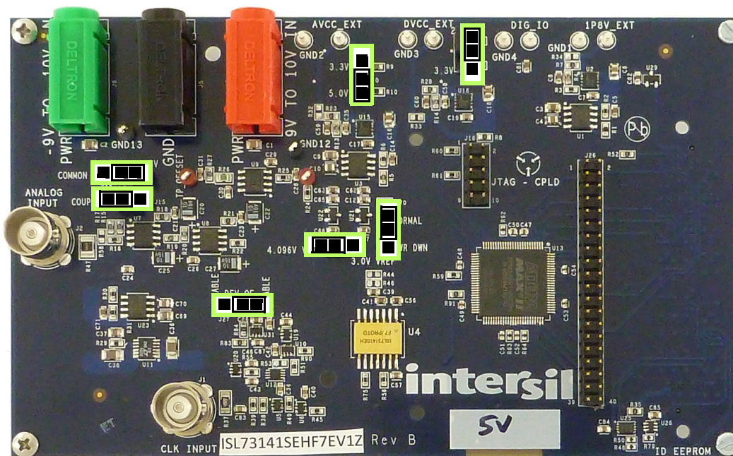
Figure 3. ISL73141SEHF7EV1Z Evaluation Board Jumper Location
