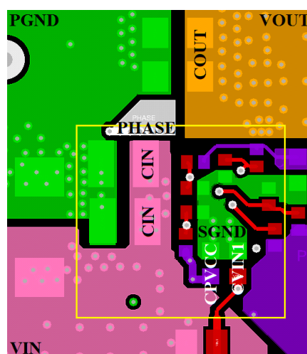
Figure 3. Layout Example - Bottom Layer
