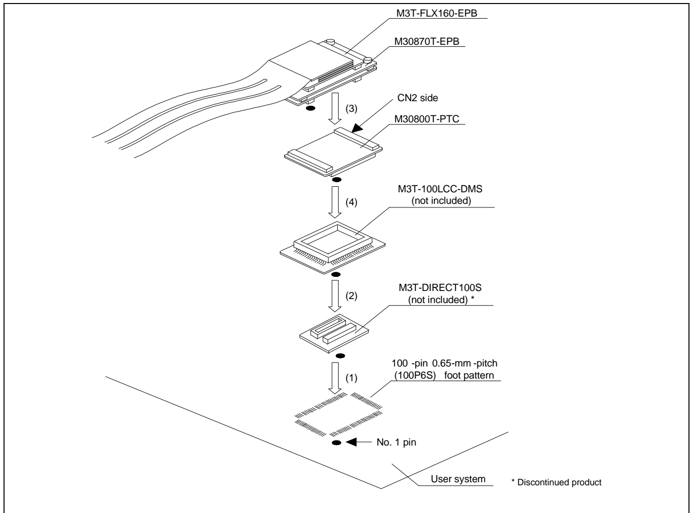
Figure 2.10 Connecting to a 100-pin 0.65-mm-pitch foot pattern (2/3)
