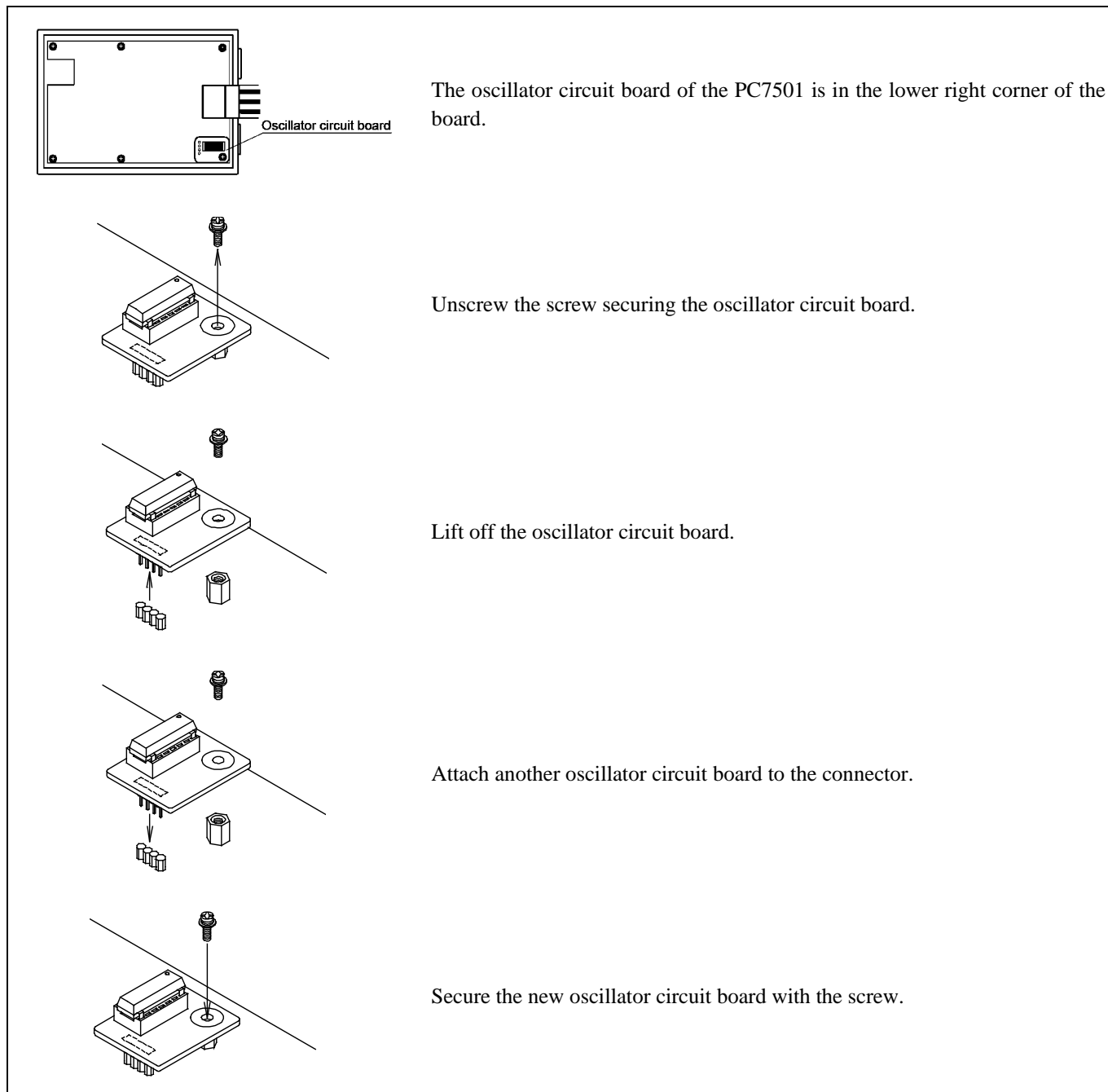
Figure 2.19 Replacing oscillator circuit boards
