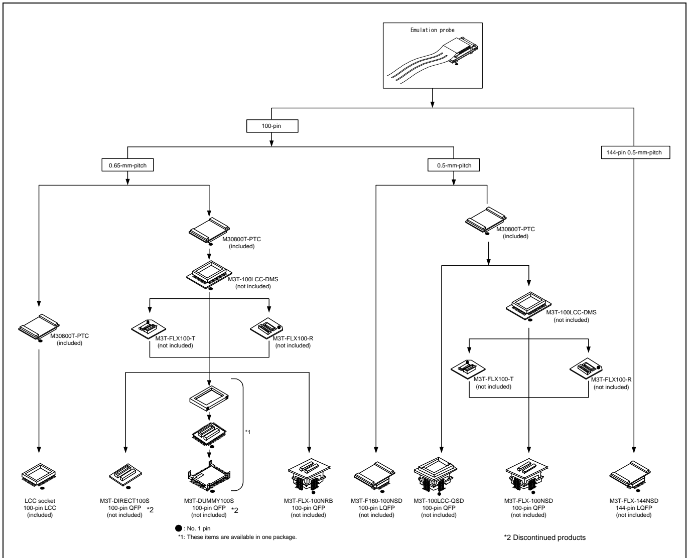
Figure 2.7 Connection of the M30870T-EPB and user system
