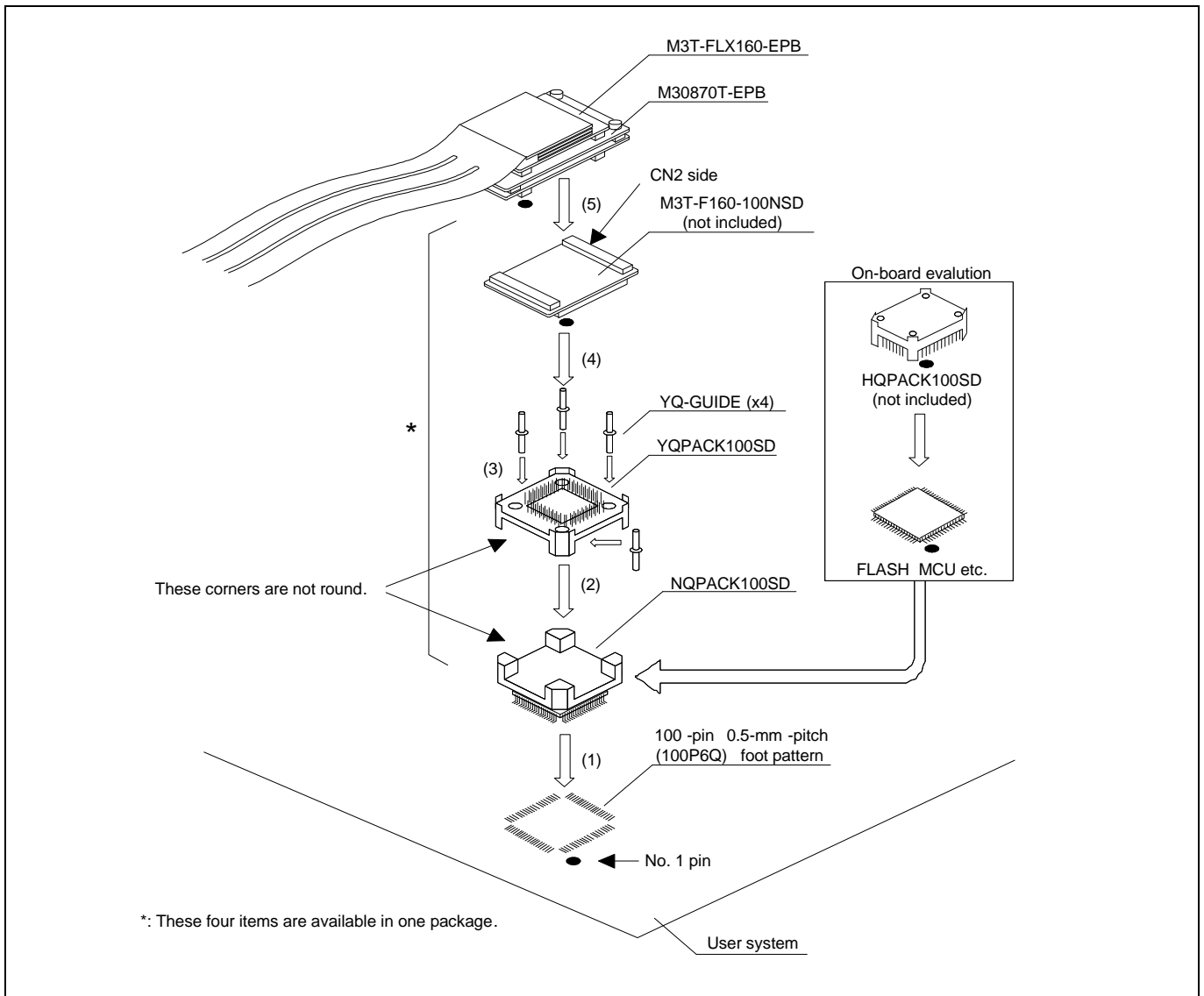
Figure 2.14 Connecting to a 100-pin 0.5-mm-pitch foot pattern (3/3)
