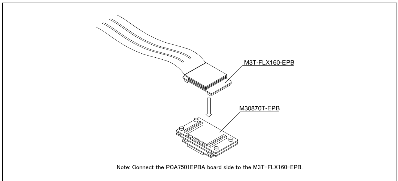
Figure 2.3 Connecting the PC7501 and emulation probe
