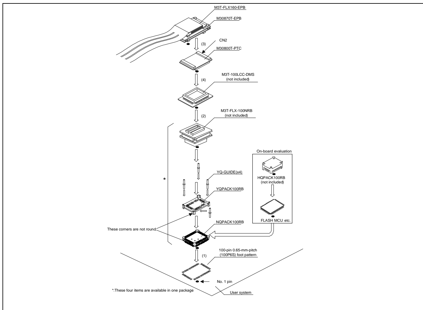
Figure 2.11 Connecting to a 100-pin 0.65-mm-pitch foot pattern (3/3)
