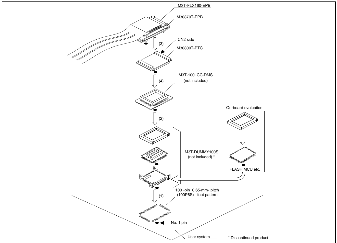
Figure 2.9 Connecting to a 100-pin 0.65-mm-pitch foot pattern (1/3)
