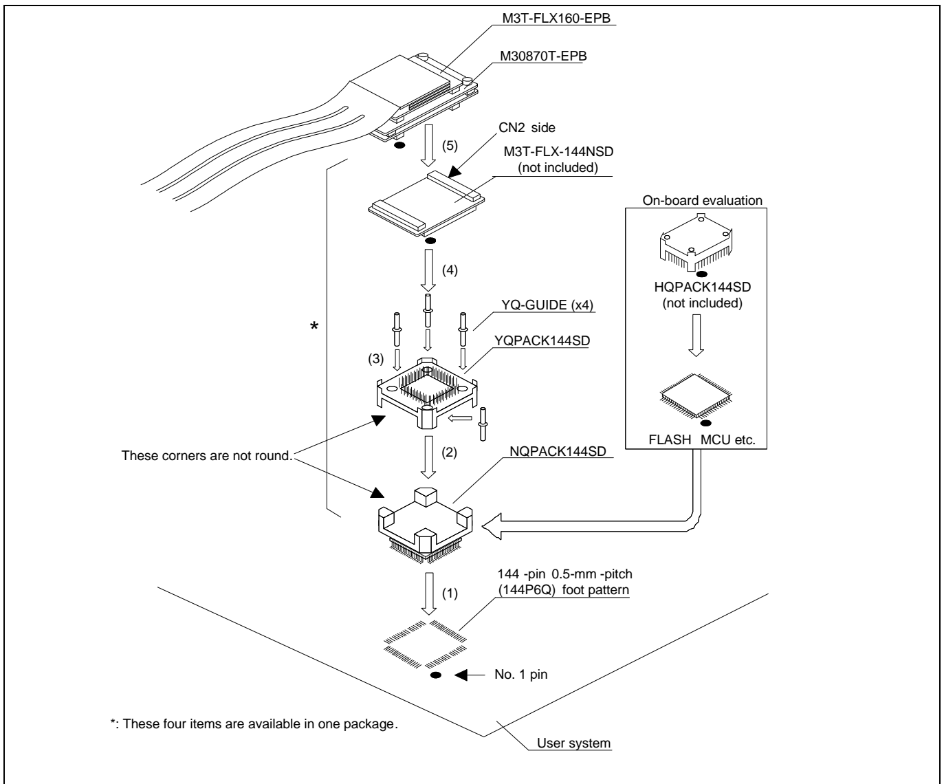
Figure 2.15 Connecting to a 144-pin 0.5-mm-pitch foot pattern
