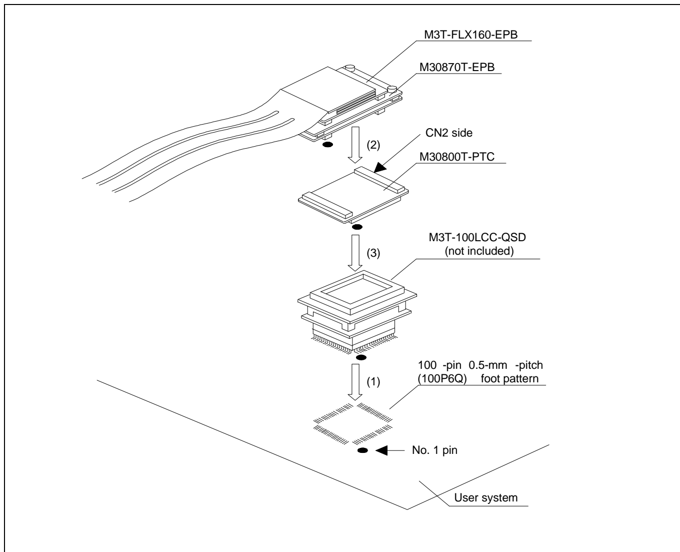
Figure 2.12 Connecting to a 100-pin 0.5-mm-pitch foot pattern (1/3)
