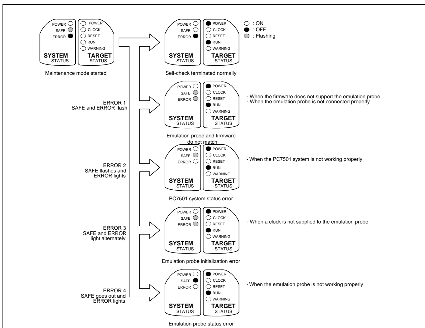
Figure 2.6 Self-check procedure
