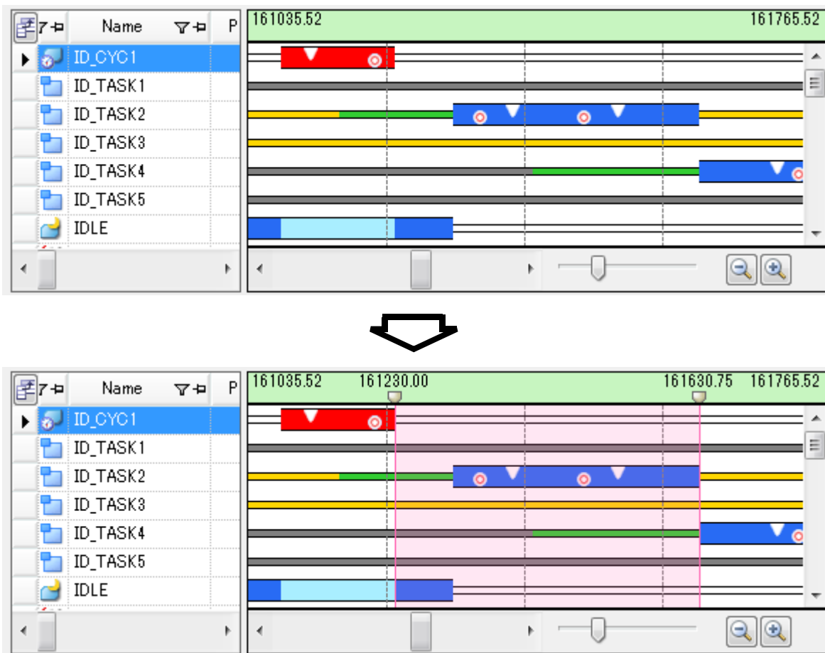
Figure 2.8 Limiting Range of Usage Status
