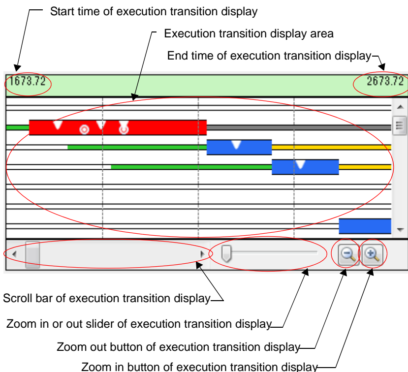
Figure A.4 Analysis Information Diagram Area
