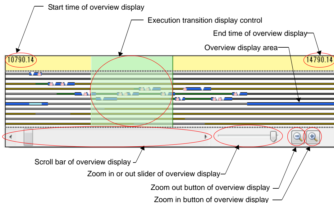
Figure A.6 Analysis information overview display area
