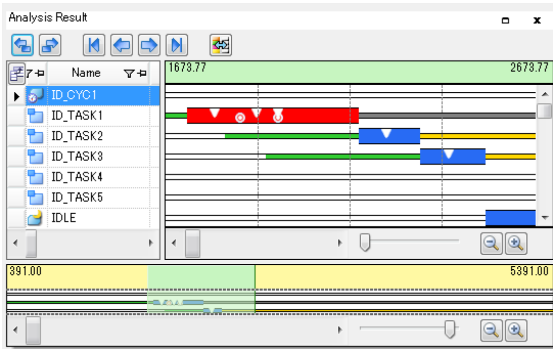
Figure 2.2 Analysis Result Panel
