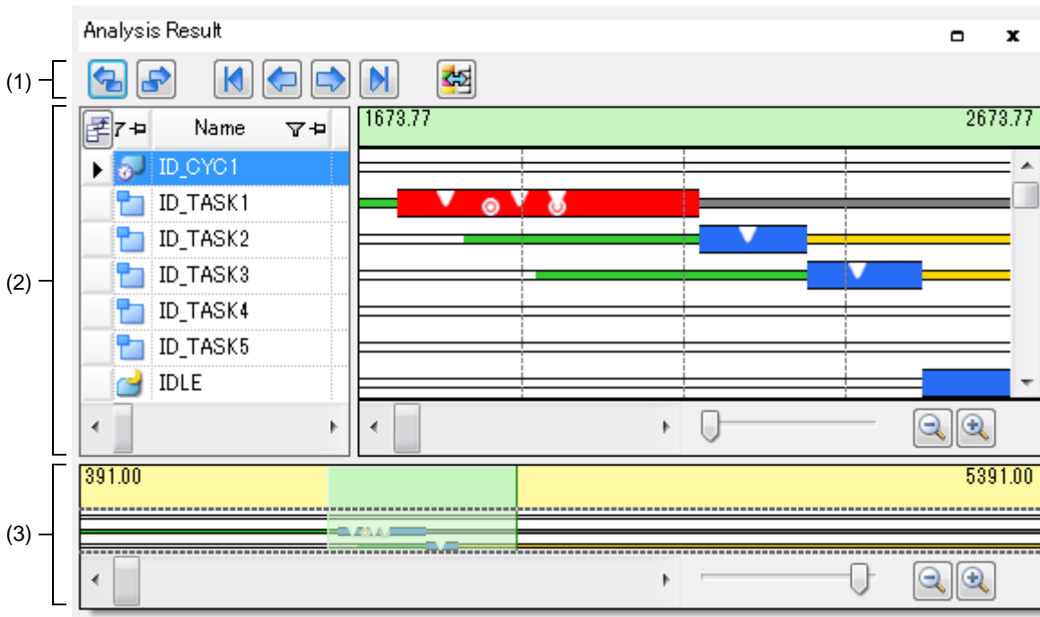
Figure A.2 Analysis Result Panel
