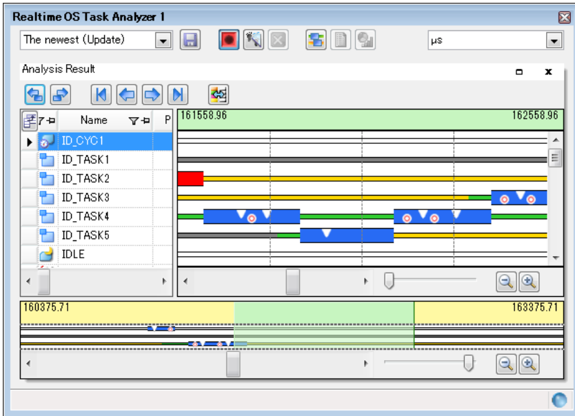
Figure 2.9 Clear Analysis Information
