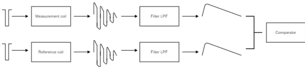
Figure 7. Working principle
