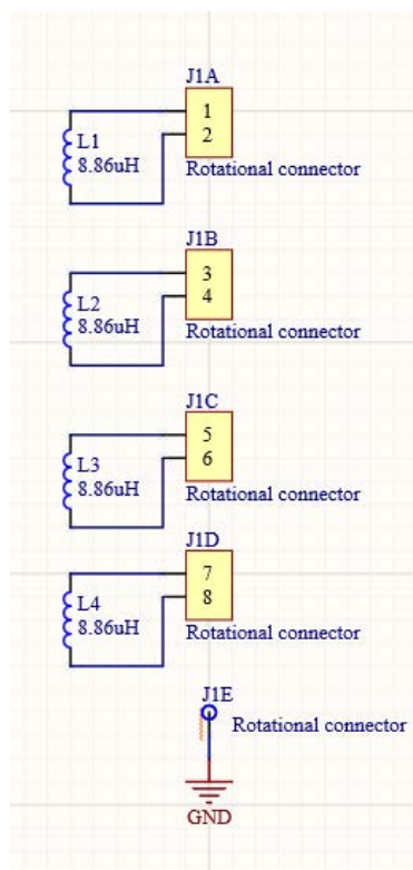
Figure 35. Rotation coils
