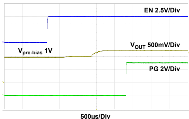
Figure 25. Pre-biased Power-Up Waveform, Pre-biased Voltage = 1V, V_{IN} = 5V , V_{OUT} = 1.2V , f_{SW} = 1.2MHz , I_{OUT} = \text{No Load} , C_{OUT} = 2x22µF Ceramic
