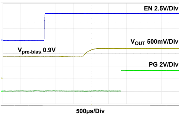
Figure 24. Pre-biased Power-Up Waveform, Pre-biased Voltage = 0.9V, V_{IN} = 3.3V , V_{OUT} = 1.2V , f_{SW} = 1.2MHz , I_{OUT} = \text{No Load} , C_{OUT} = 2x22µF Ceramic
