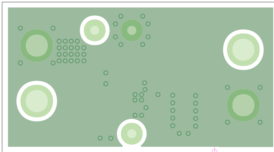
Figure 8. Bottom Layer
