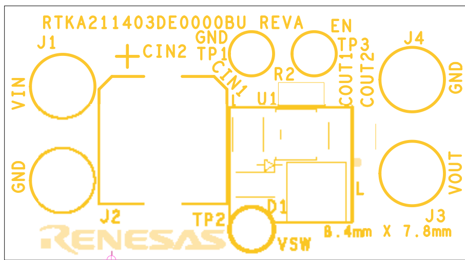
Figure 6. Silkscreen Top
