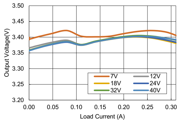
Figure 21. Load Regulation
