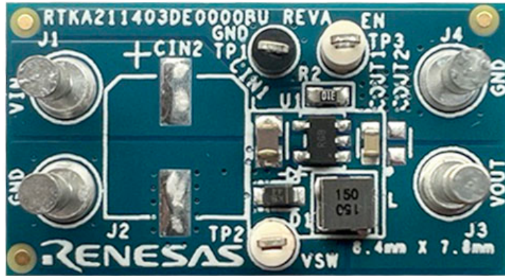
Figure 4. RTKA211403DE0000BU Evaluation Board (Top)
