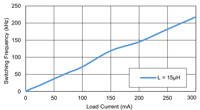
Figure 3. Switching Frequency (VIN: 24V) vs. Load Current
