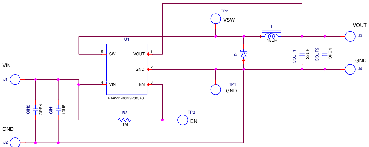
Figure 5. RTKA211403DE0000BU Schematic
