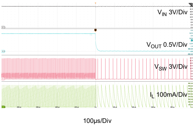
Figure 14. Short-Circuit
