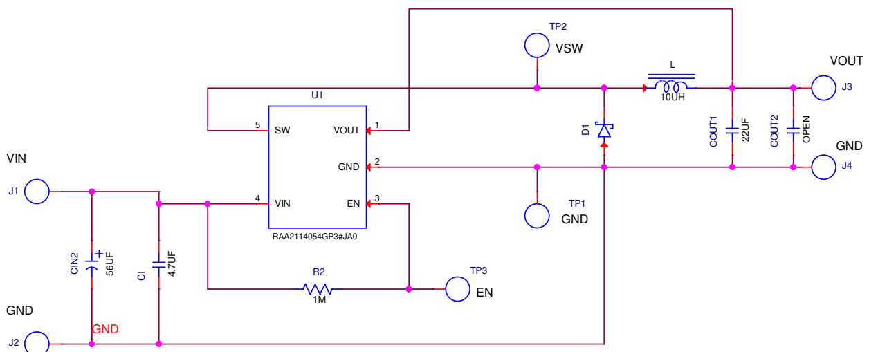
Figure 5. RTKA211405DE0000BU Schematic
