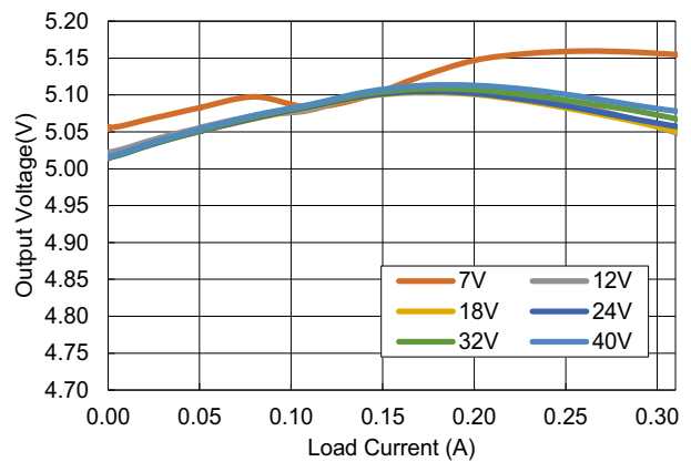
Figure 21. Load Regulation
