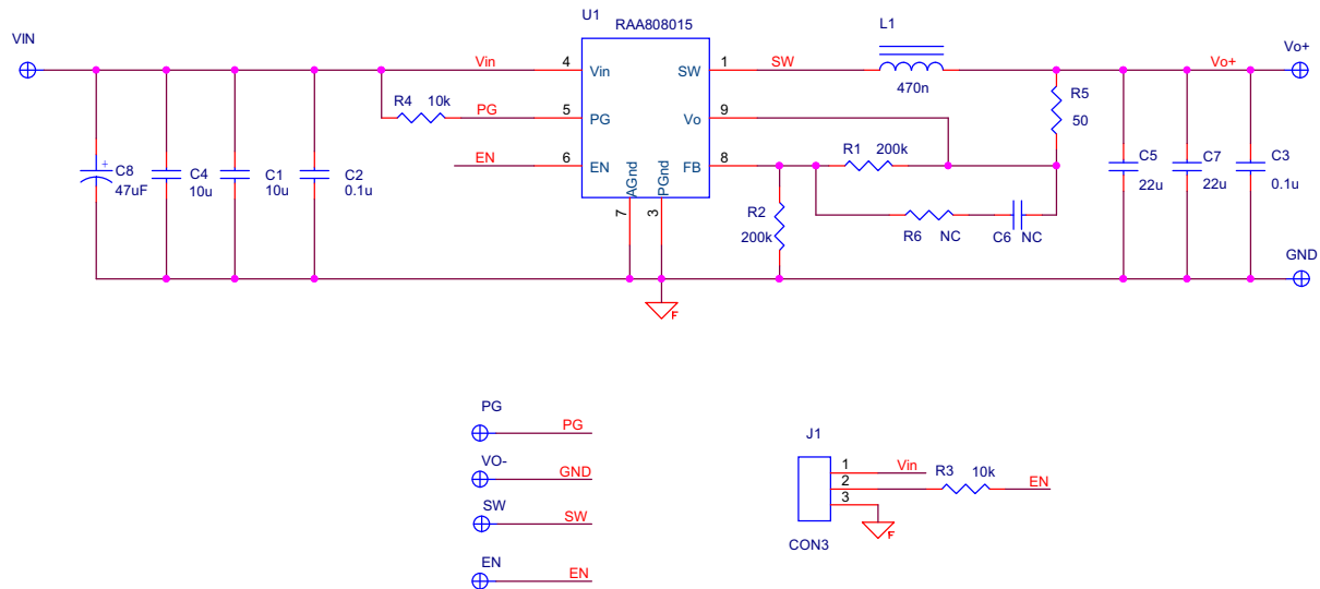
Figure 3. RTKA808015DE0020BU Schematic
