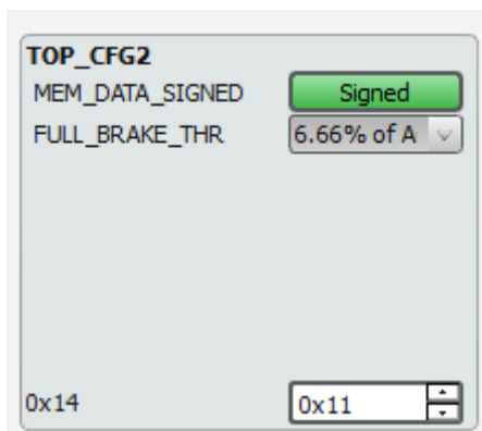
Figure 30: MEM_DATA_SIGNED Bit
