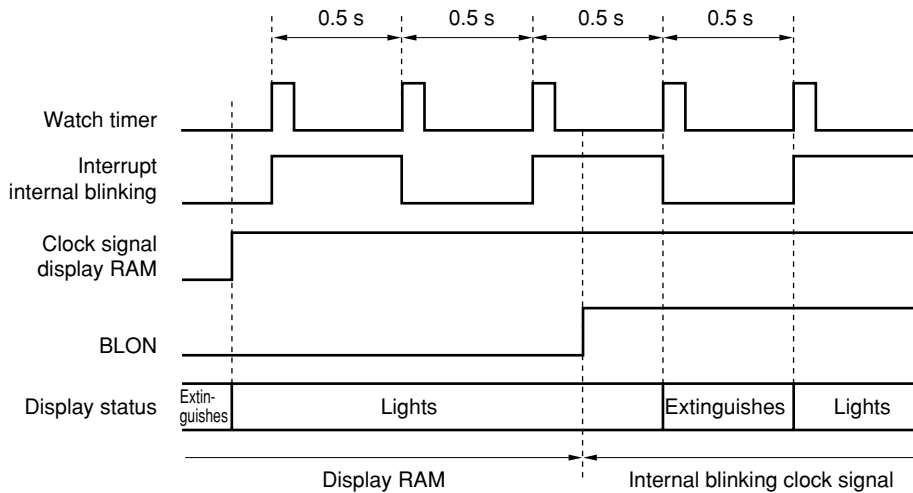
Figure 17-3. Blinking Function
