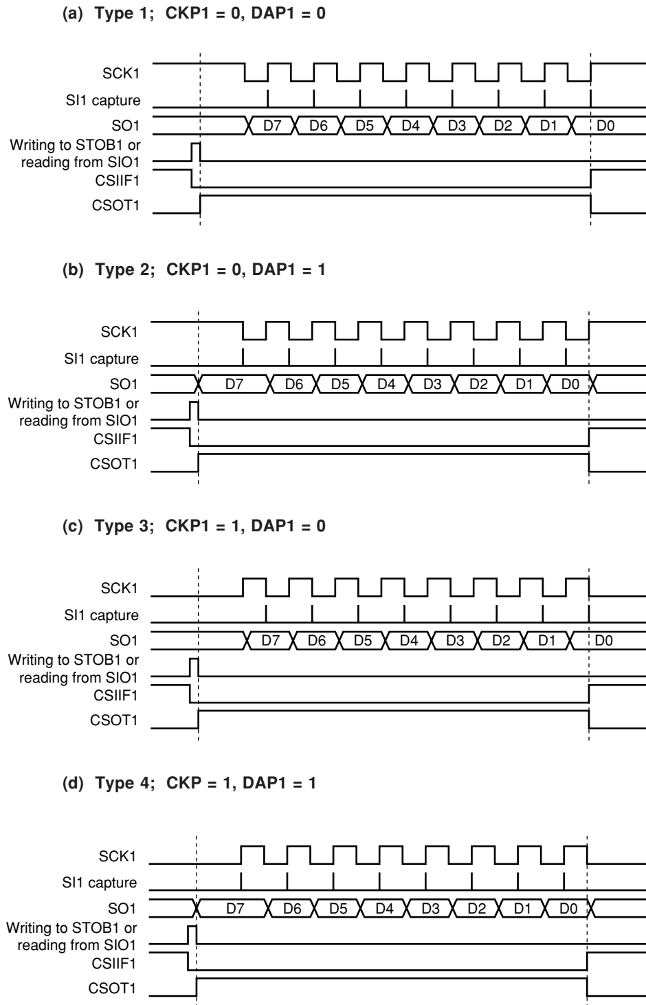
Figure 16-5. Timing of Clock/Data Phase
