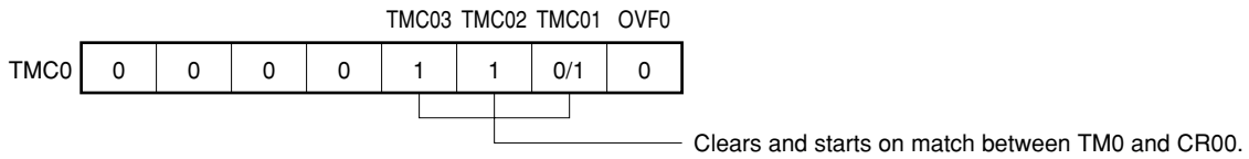
(b) Capture/compare control register 0 (CRC0)
