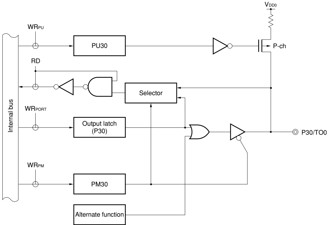
Figure 4-7. P30 Block Diagram
