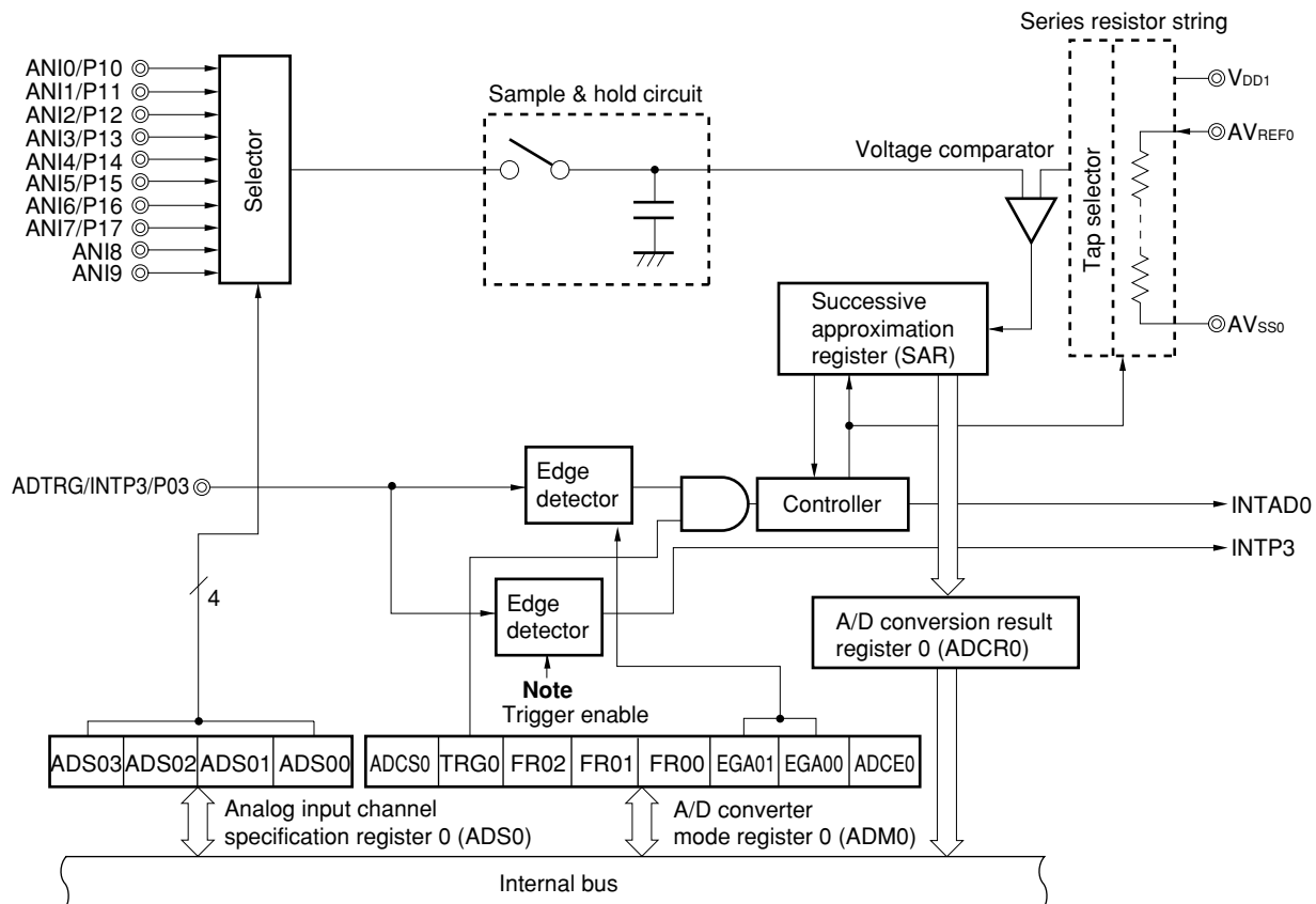
Figure 12-1. A/D Converter Block Diagram
