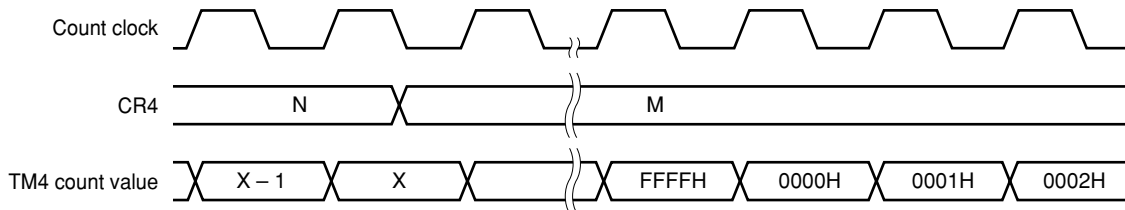
Figure 7-8. Timings After Change of Compare Register During Timer Count Operation
