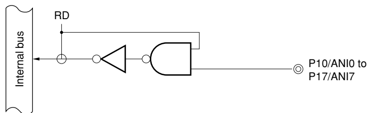
Figure 4-4. P10 to P17 Block Diagram
