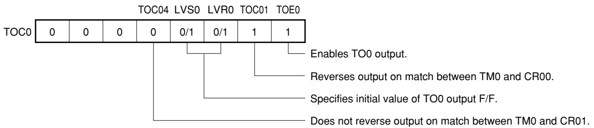
(c) 16-bit timer output control register 0 (TOC0)
