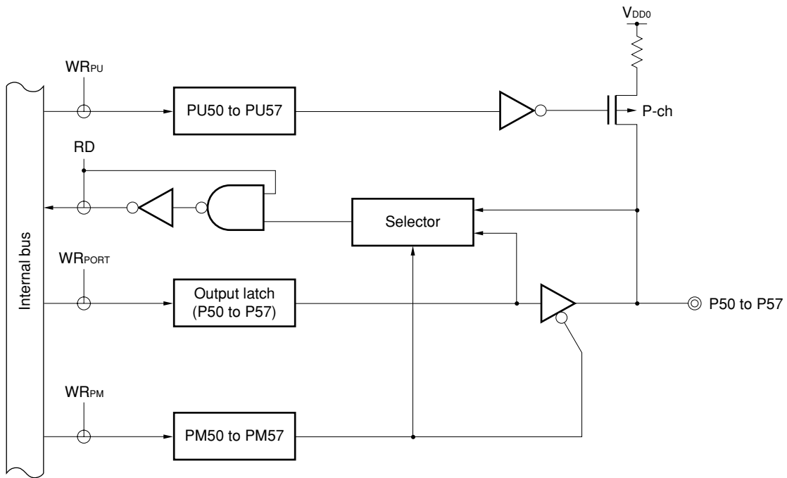
Figure 4-12. P50 to P57 Block Diagram
