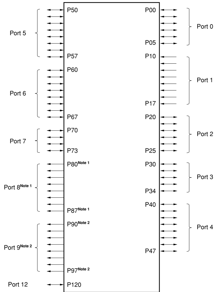
Figure 4-1. Port Types
