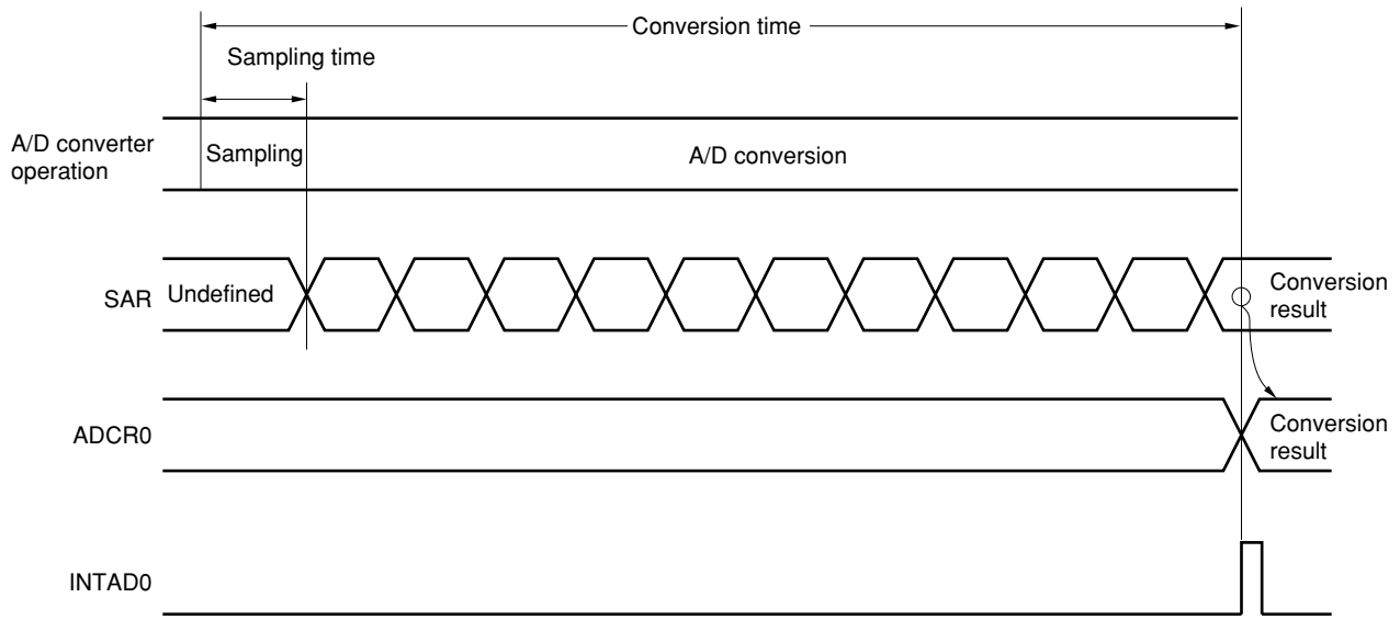
Figure 12-5. Basic Operation of A/D Converter
