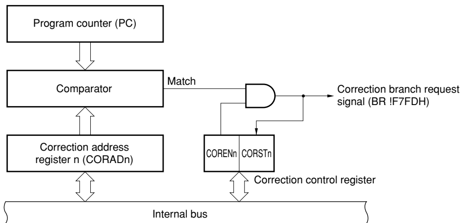
Figure 21-1. ROM Correction Block Diagram
