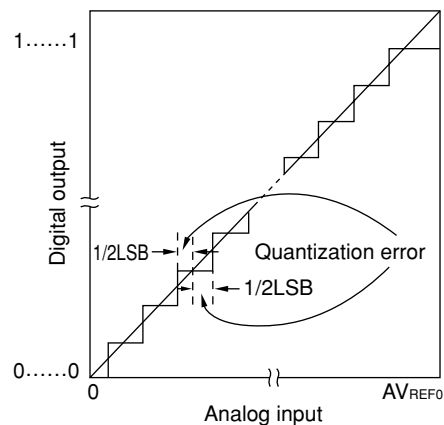
Figure 12-10. Quantization Error
