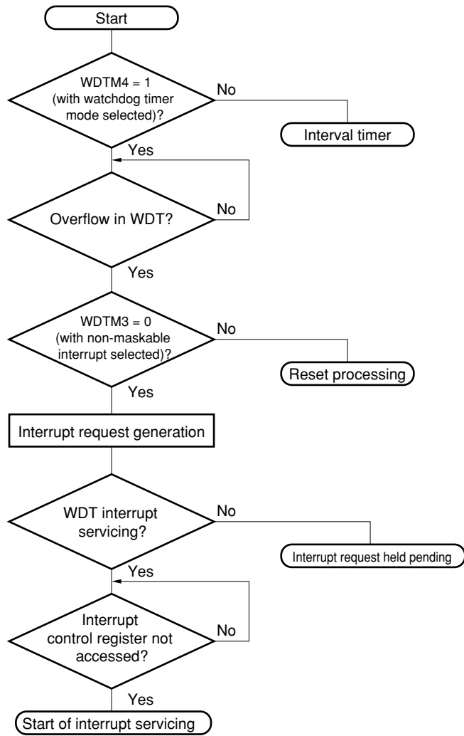
Figure 18-7. Non-Maskable Interrupt Request Generation to Acknowledge Flowchart
