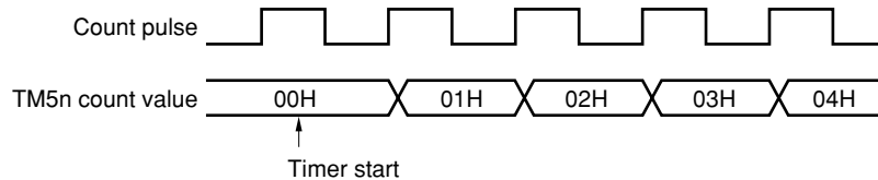
Figure 8-14. 8-Bit Timer Counter Start Timing
