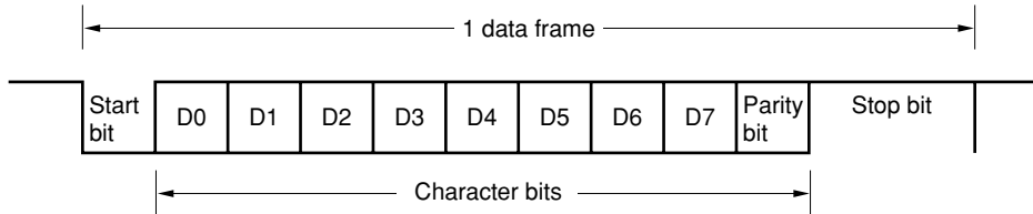
Figure 14-7. Format of Transmit/Receive Data in Asynchronous Serial Interface
