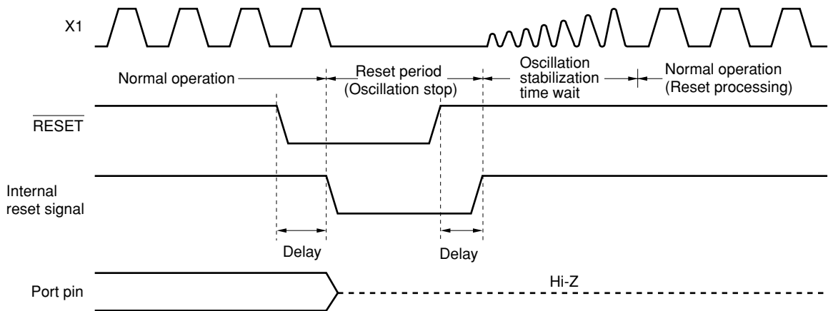
Figure 20-3. Timing of Reset Due to Watchdog Timer Overflow
