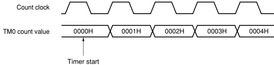
Figure 6-26. 16-Bit Timer Counter 0 (TM0) Start Timing
