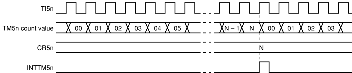
Figure 8-10. External Event Counter Operation Timing (with Rising Edge Specified)
