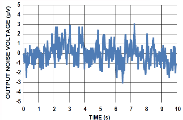
V_{OUT} vs NOISE, 0.1Hz TO 10Hz
