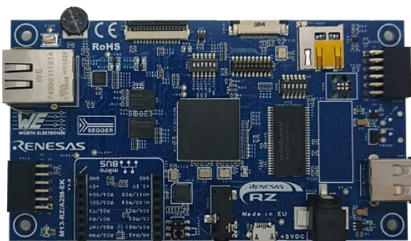
Component Side View
