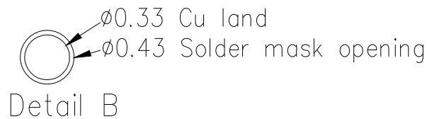
Recommended Land Pattern (PCB Top View, NSMD Design)
