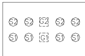
TERMINAL LAYOUT (Top view)
