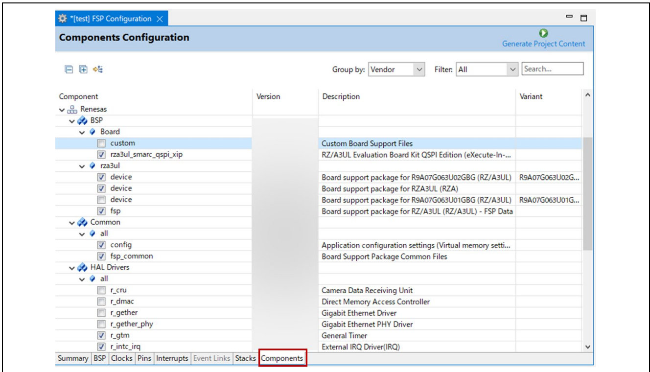
Figure 98 : Components Tab
