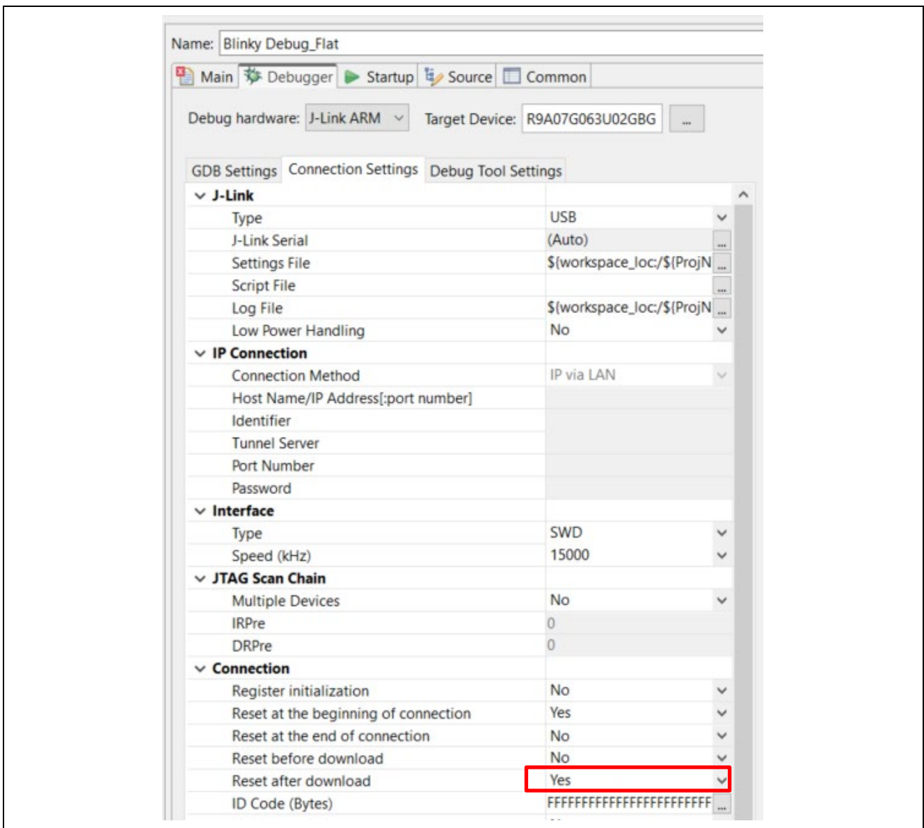
Figure 59 : e2 studio Debugger Configurations window with Blinky project (4)
