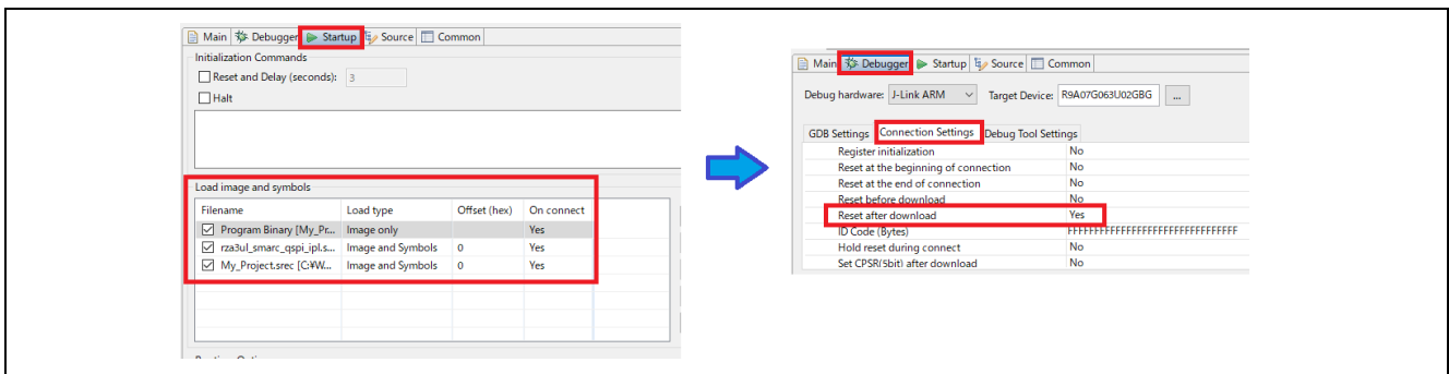
Figure 101 : Debug Setting
