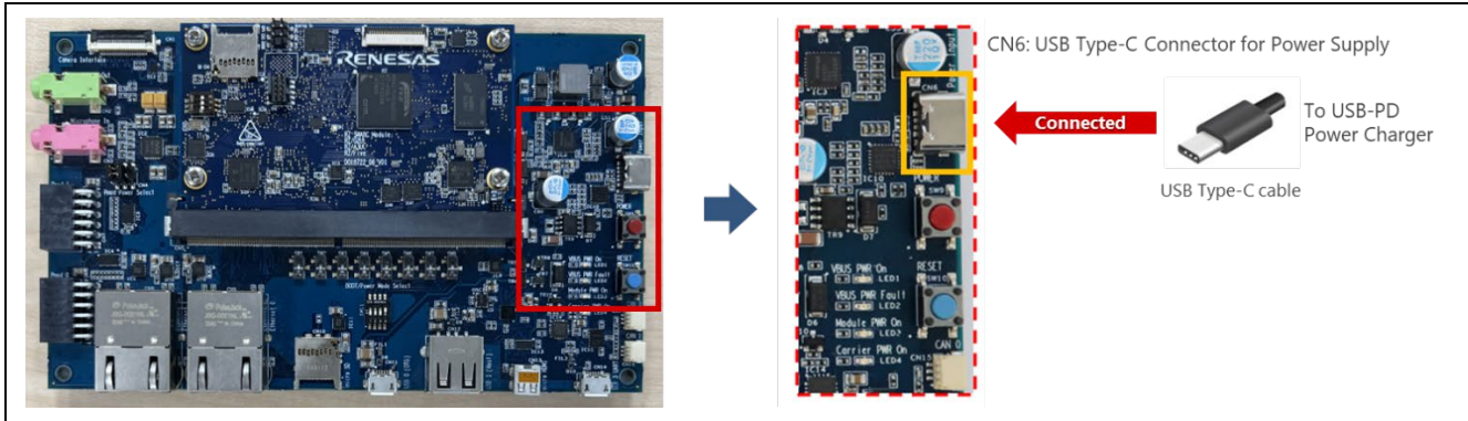
Figure 40: Power Supply
