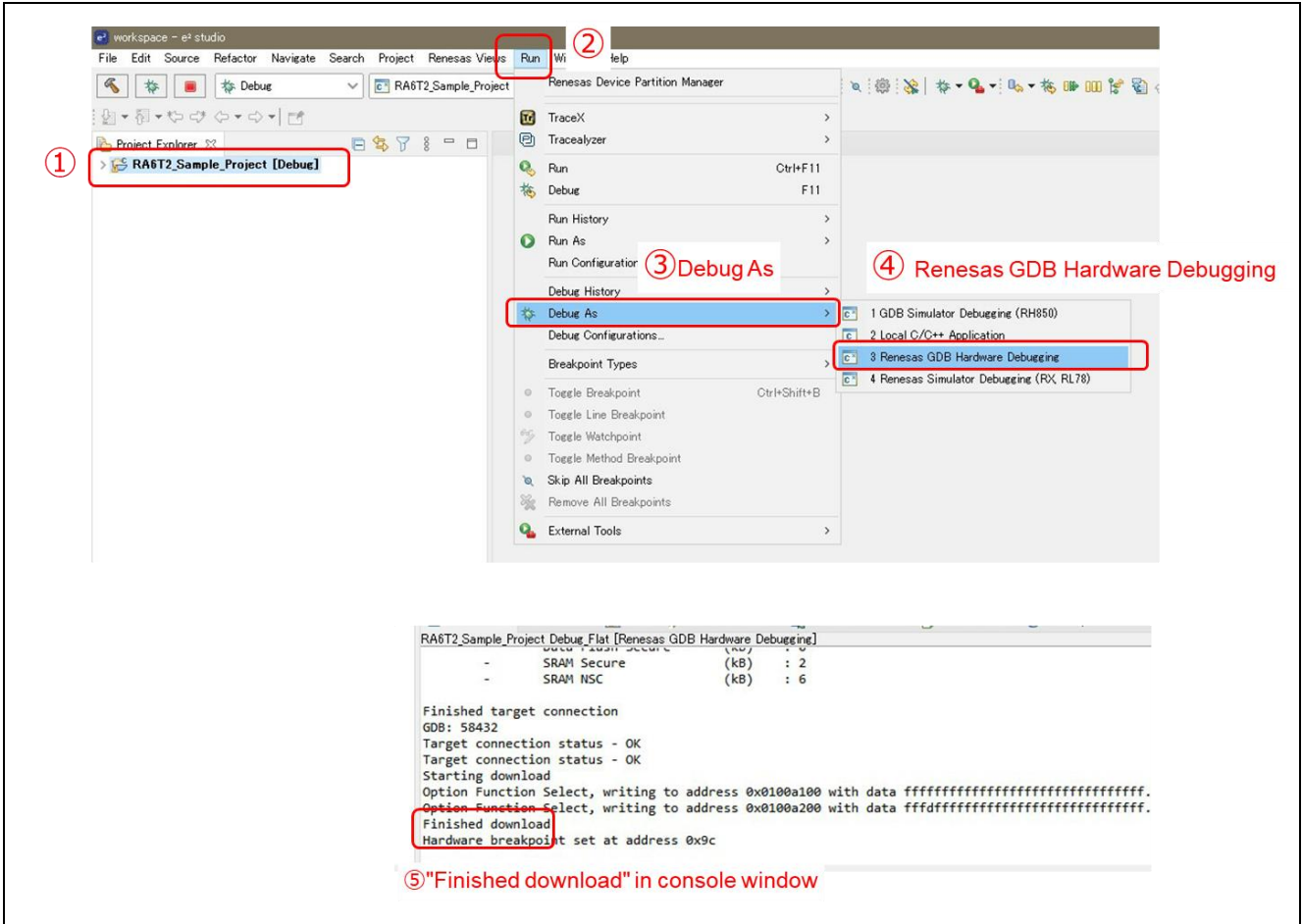
Figure 5-5 Flash programming
