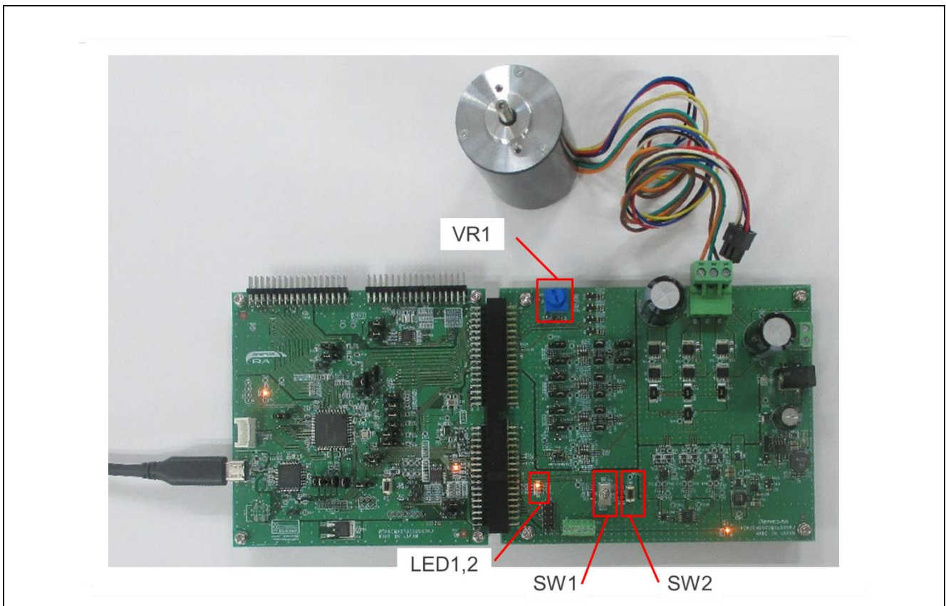
Figure 4-6 Operating State
