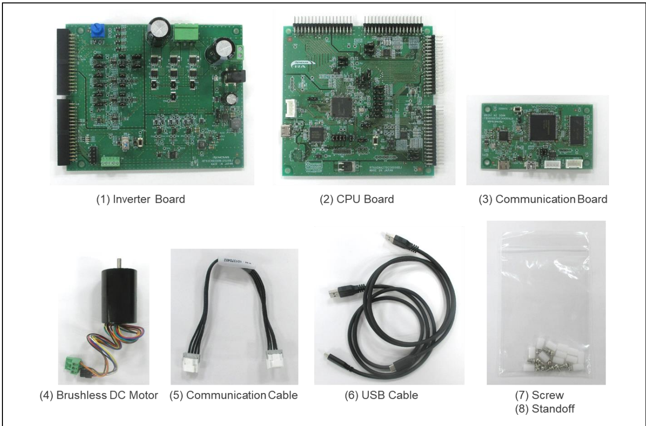
Figure 2-1 Product contents
