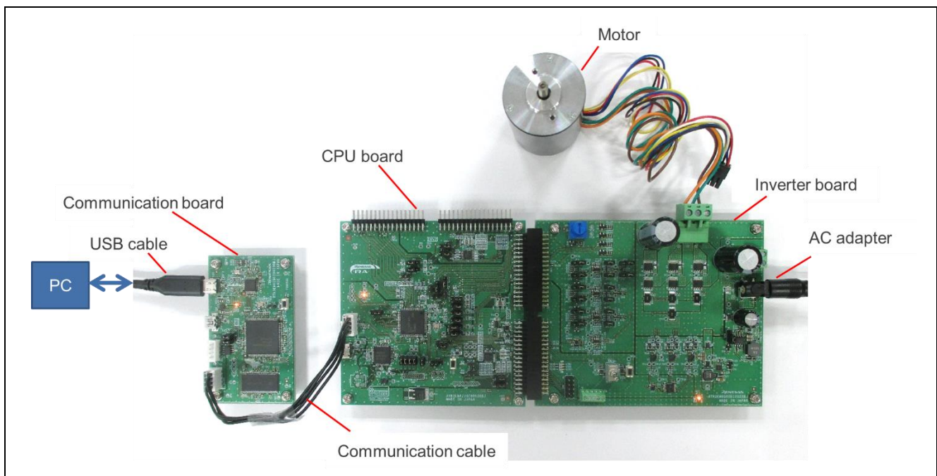
Figure 6-1 Hardware Configuration
