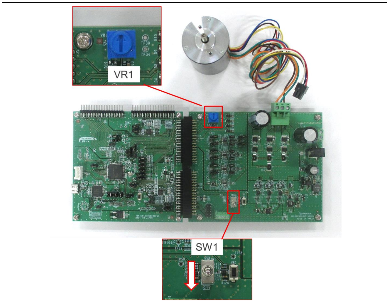
Figure 4-4 Hardware configuration
