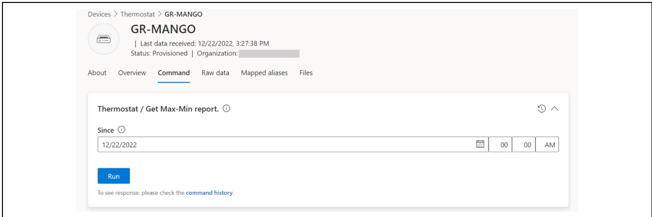
Figure 7-14 Send commands
