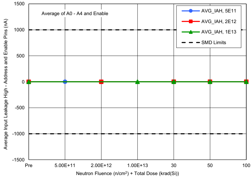
Figure 3. HS-1840AxH average input leakage current high, address or enable pins ( I_{AH} ) at V+ = +15V , V- = -15V , following irradiation to each level. The error bars (if visible) represent the minimum and maximum measured values across all pins. The SMD limits are -1000nA minimum and 1000nA maximum.
