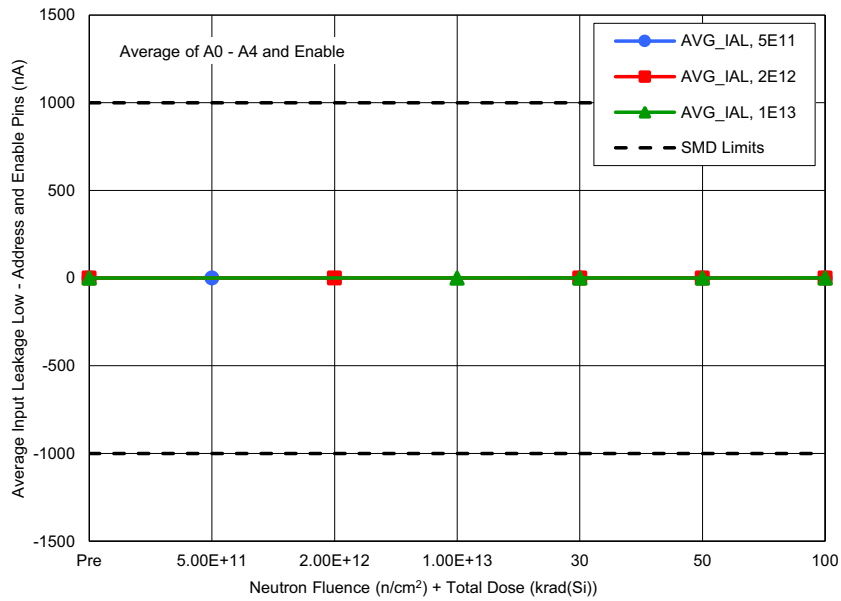
Figure 4. HS-1840AxH average input leakage current low, address or enable pins ( I_{AL} ) at V+ = +15V , V- = -15V , following irradiation to each level. The error bars (if visible) represent the minimum and maximum measured values across all pins. The SMD limits are -1000nA minimum and 1000nA maximum.
