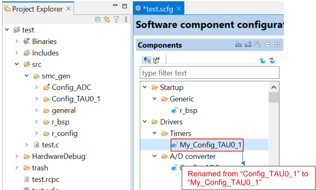
Figure 6-6 The Interval Timer component configuration after renaming
