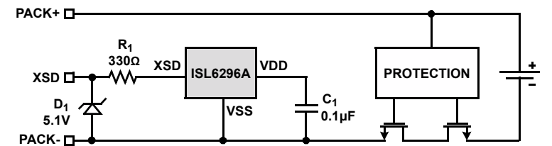
FIGURE 2. TYPICAL APPLICATION WITH THE ISL6296A POWERED BY THE XSD BUS
