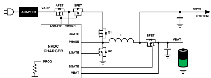
FIGURE 2. NVDC CHARGER CONFIGURATION
