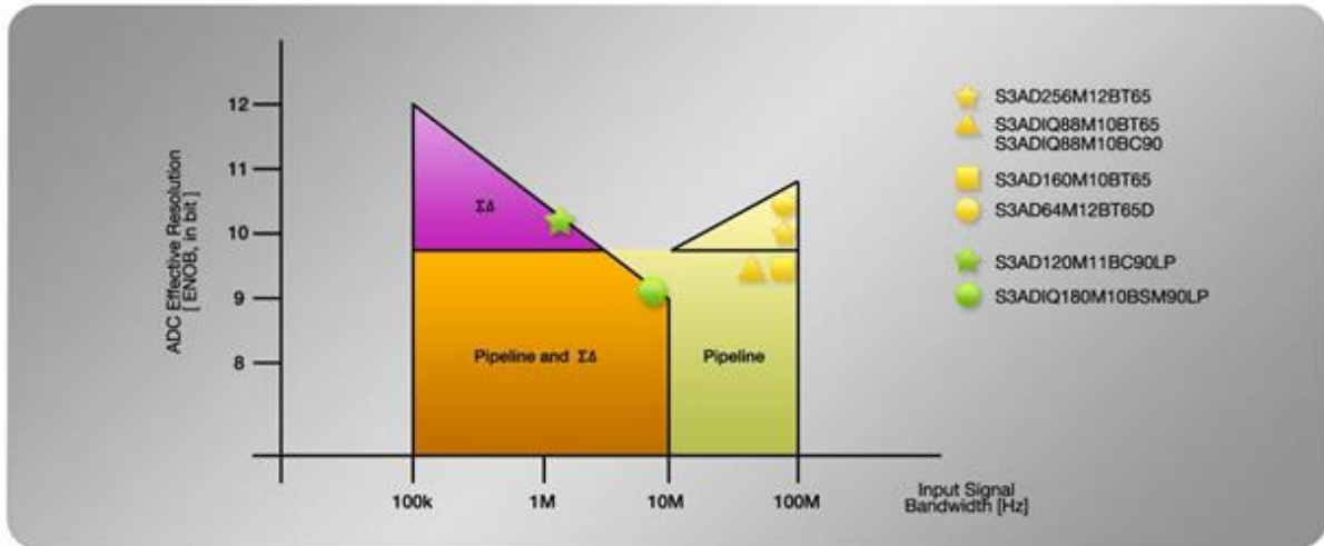
Figure 3: Performance range of Pipeline and \Sigma\Delta ADCs
